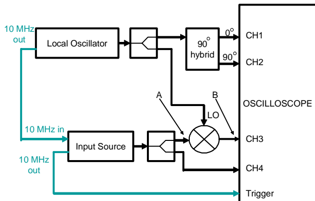
Fig. 1. Our measurement setup. Not shown in the figure are an isolator in the LO path and 16 dB attenuators at the two output ports of the lower splitter that prevent signals reflected from or generated in the mixer from interfering with the signals on channels 1, 2, and 4.
