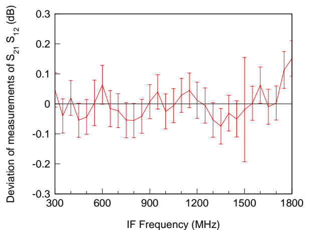
Fig. 6. Comparison of the product of the up-conversion and down-conversion loss |S_{21} S_{12}| measured with our oscilloscope and the average of the round-trip conversion losses measured with a VNA.
