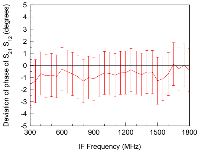
Fig. 8. Comparison of the phase of the product S_{21} S_{12} measured with our oscilloscope and with a VNA.
