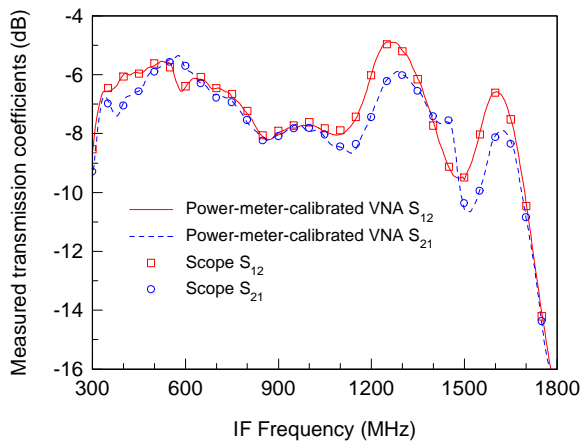
Fig. 5. Comparison of the up-conversion loss |S_{21}| and the down-conversion loss |S_{12}| measured with our oscilloscope and a power-meter-calibrated VNA.
