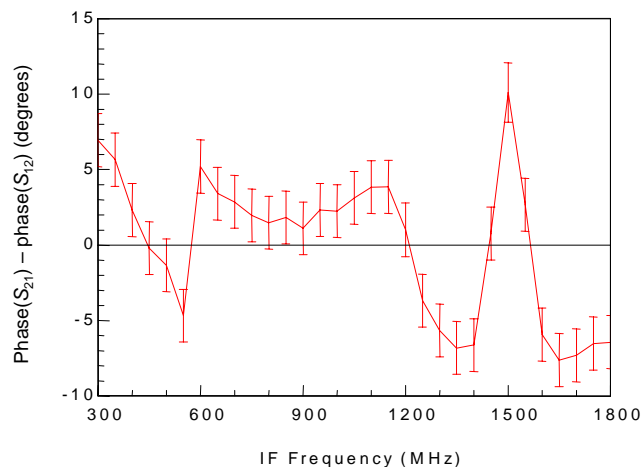
Fig. 9. The difference of the phase of S_{21} and S_{12} measured with our oscilloscope after subtracting a constant offset due to the unknown phase of the local oscillator.
