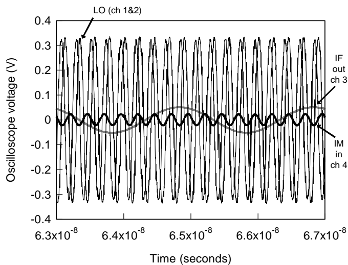
Fig. 2. Typical oscilloscope traces measured during our experiment before time-base and jitter correction. The thin traces are the in-phase and quadrature copies of the local oscillator measured on channels 1 and 2 of the oscilloscope. These traces are used to establish the time base. The thick black line is the copy of the signal going into the image port of the mixer measured on channel 4 of the oscilloscope. The thick grey line is the signal at the IF output of the mixer measured on channel 3 of the oscilloscope.
