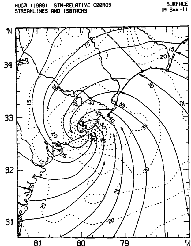
FIG. 8. As in Fig. 4, but for surface winds measured by oceanic, land-based, and adjusted aircraft platforms for 0400 UTC for 22 September 1989.
