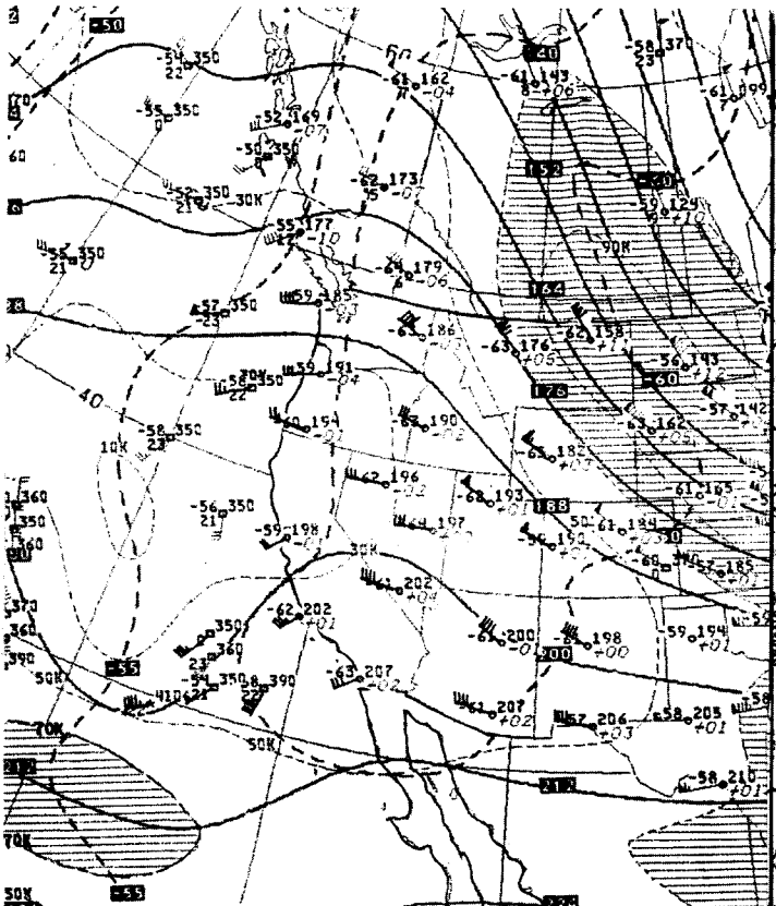
FIGURE 1. 200-mb analysis, 00Z December 29, 1985
