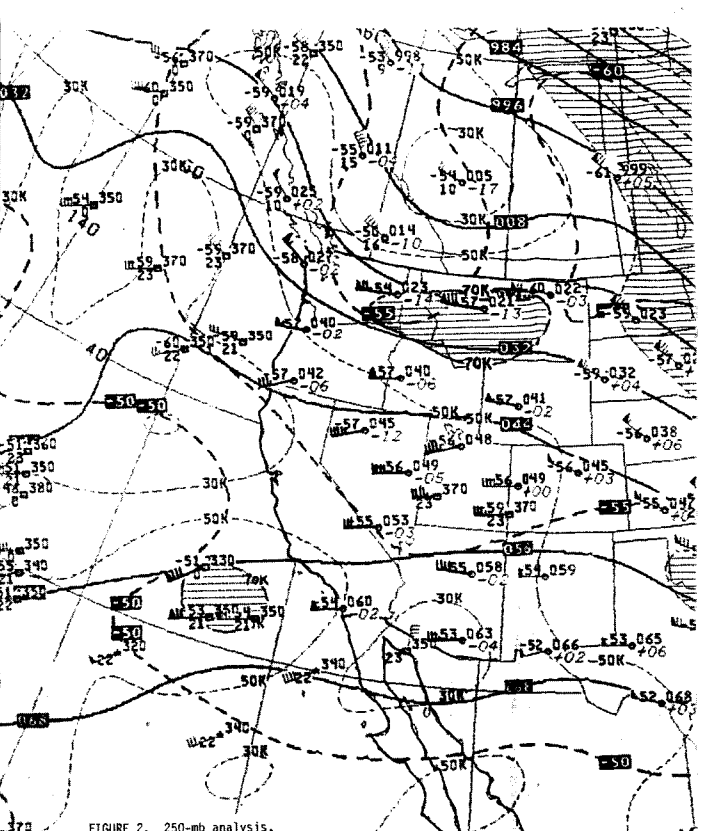
FIGURE 2. 250-mb analysis, 00Z December 30, 1985
