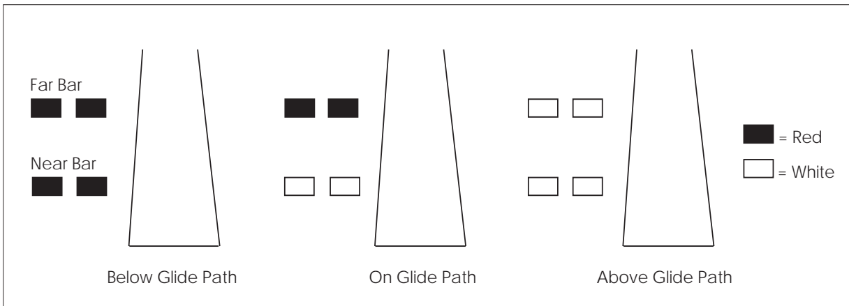
FIG AD 1.1-2 2-Bar VASI
