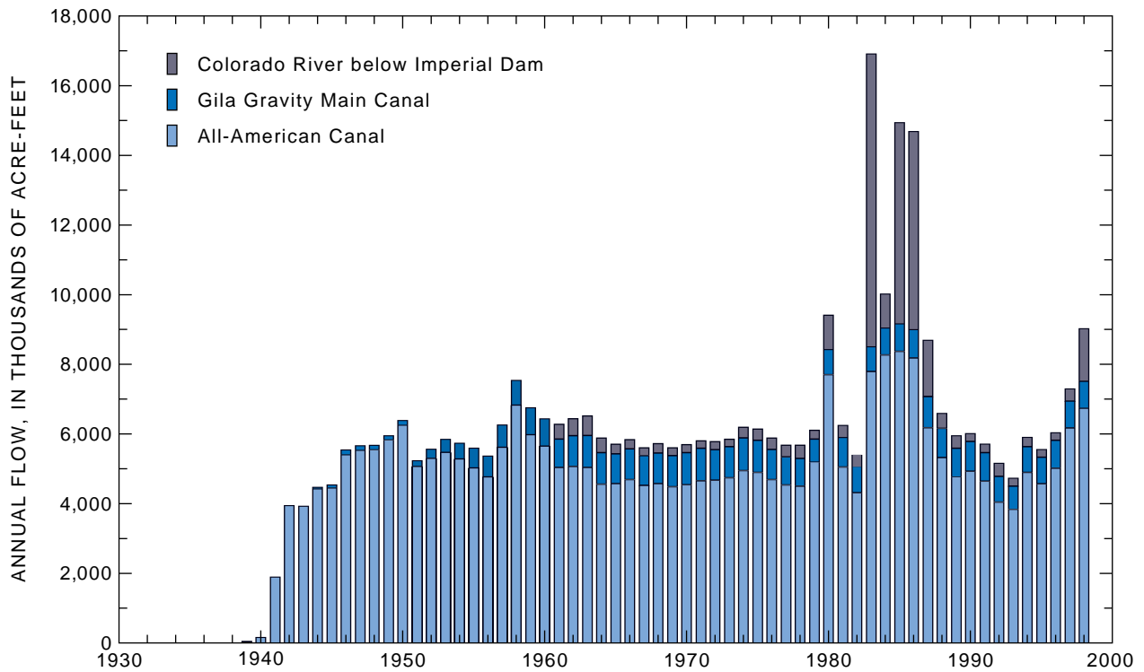
Figure 4. Annual flow in the Colorado River above Imperial Dam. This flow is the sum of flow diverted from the Colorado River into the All-American Canal near Imperial Dam, 1938–98, flow diverted into the Gila Gravity Main Canal, 1944–98, and flow in the Colorado River below Imperial Dam, 1961–98.
