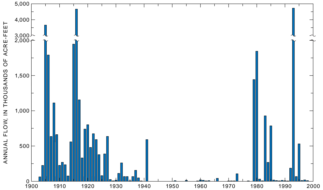
Figure 6. Annual flow in the Gila River near Dome, 1903–98.
