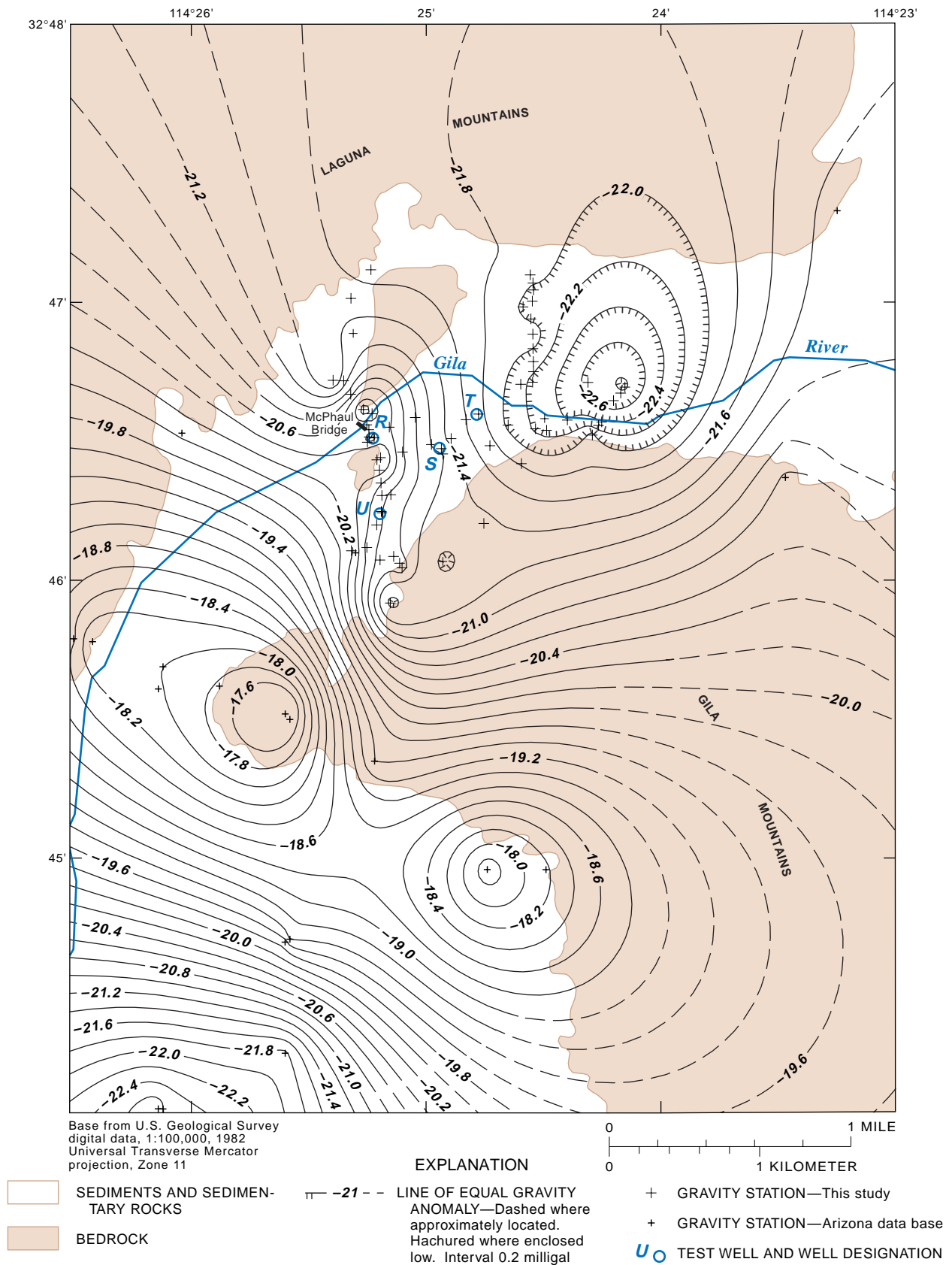
Figure 12. The complete Bouguer gravity anomaly for Gila River canyon, Arizona.
