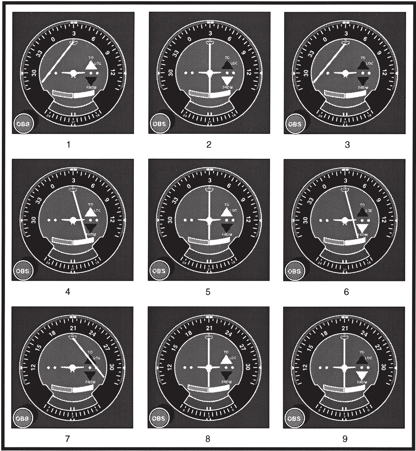
FIGURE 29.—VOR.
