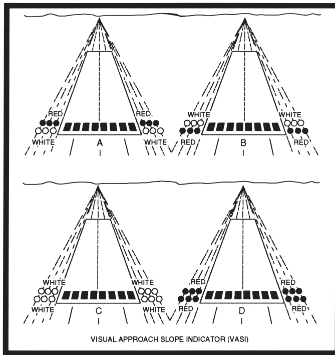
FIGURE 48.—VASI Illustrations.
