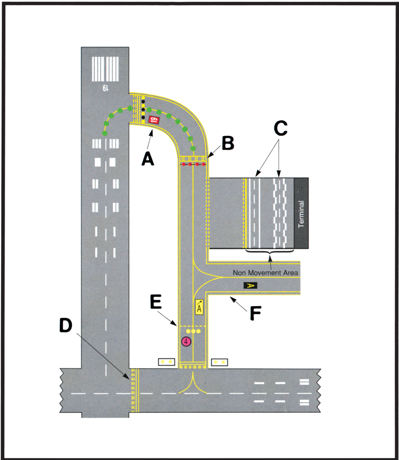
FIGURE 65.—Airport Markings.
