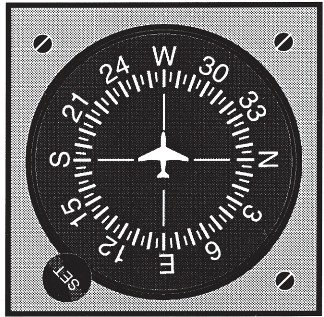
FIGURE 6.—Heading Indicator.
