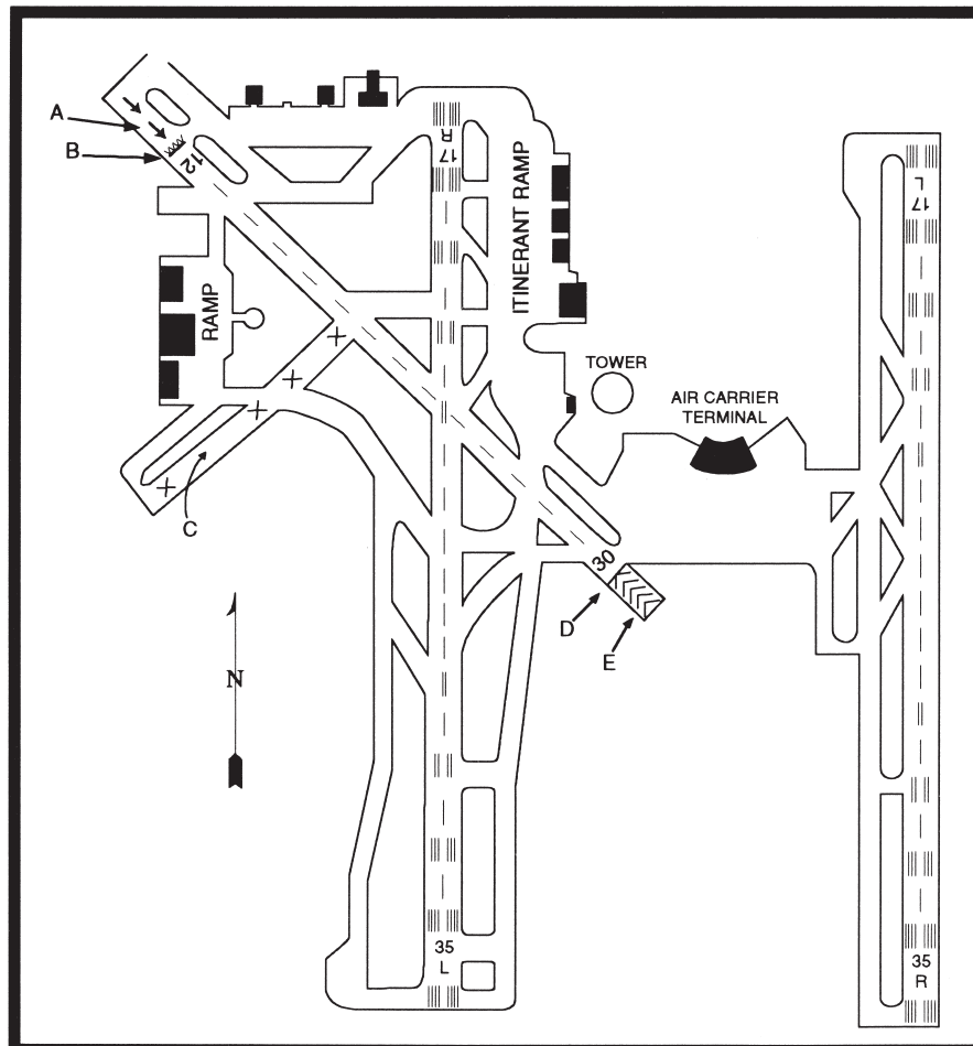
FIGURE 49.—Airport Diagram.
