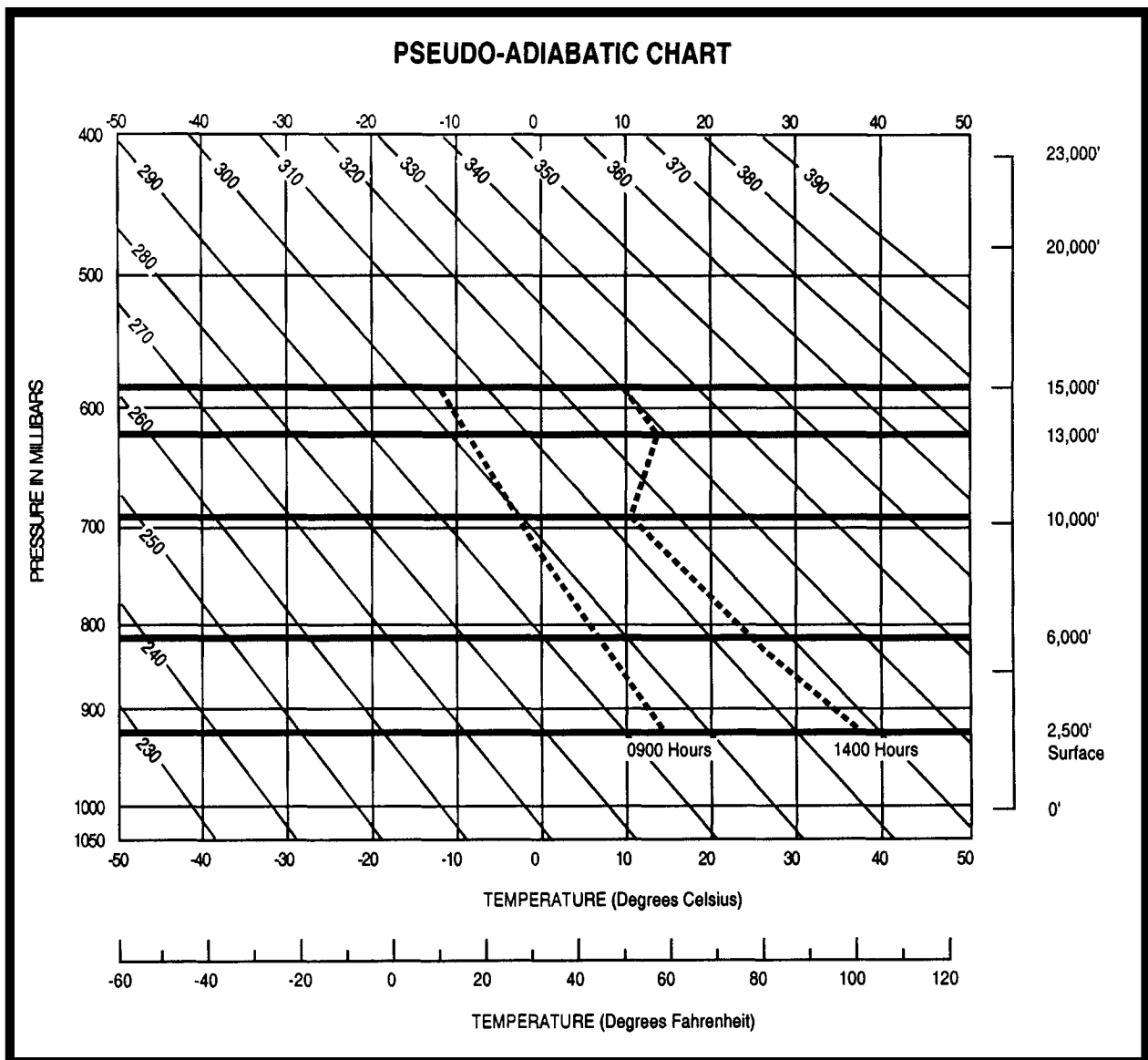
FIGURE 2.—Pseudo-Adiabatic Chart.
