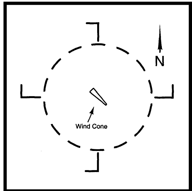
FIGURE 64.—Airport Landing Indicator.
