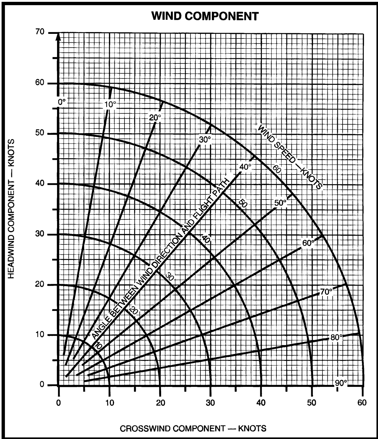
FIGURE 30.—Wind Component Chart.
