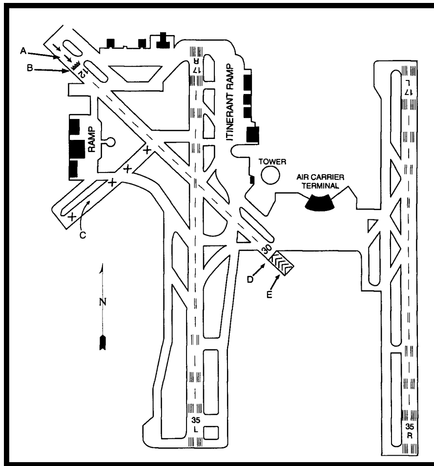
FIGURE 62.—Airport Diagram.
