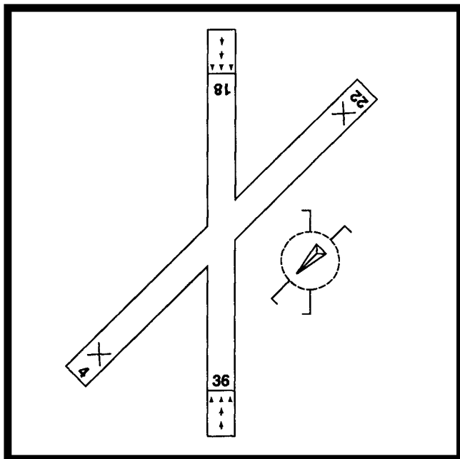
FIGURE 63.—Airport Diagram.
