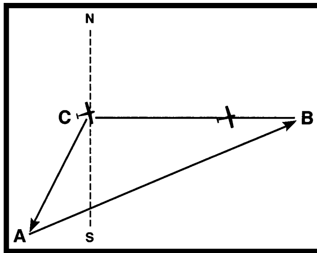
FIGURE 40.—Wind Triangle.
