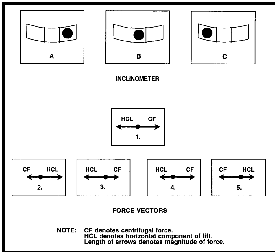
FIGURE 22.—Force Vectors.
