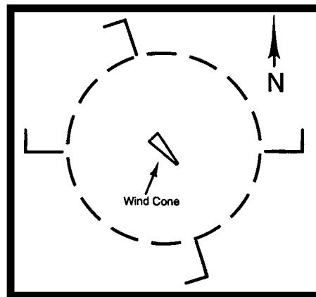
FIGURE 54.—Traffic Pattern Indicator.
