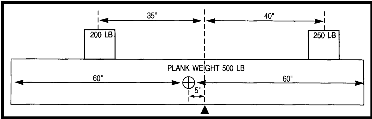
FIGURE 33.—Weight and Balance Diagram.
