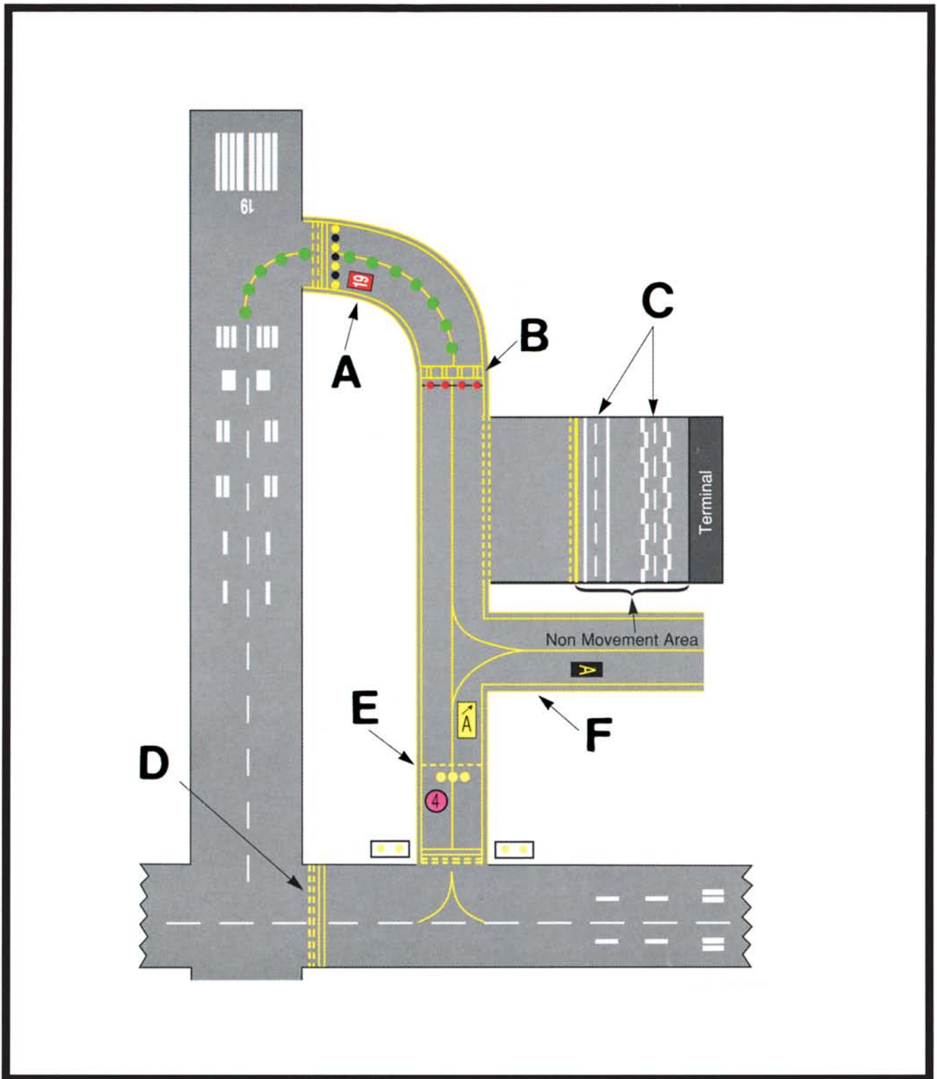
FIGURE 72.—Airport Markings.
