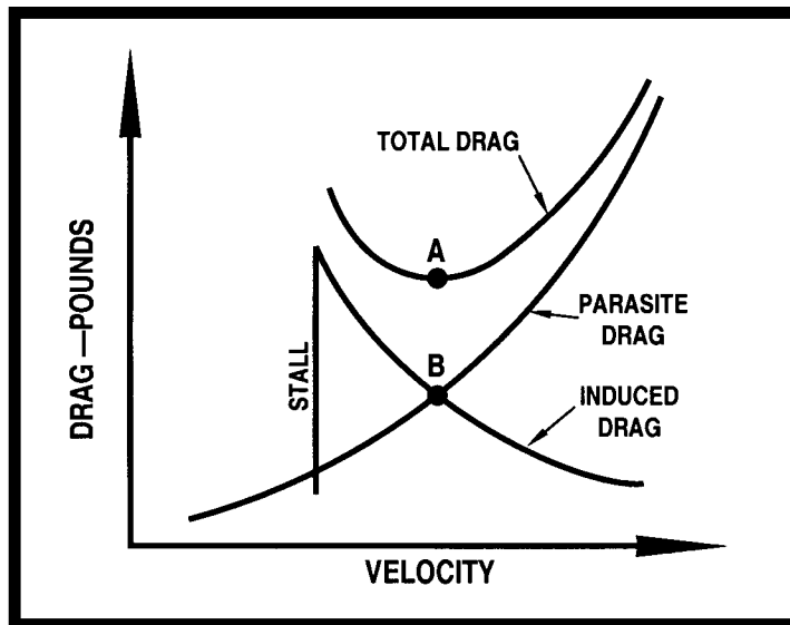
FIGURE 20.—Drag Chart.
