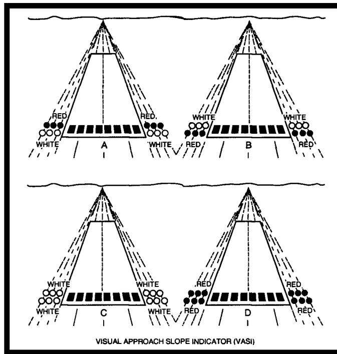
FIGURE 65.—VASI Illustrations.
