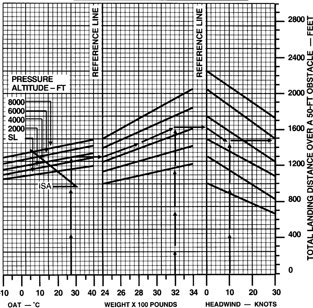
FIGURE 31.—Landing Distance Chart.
