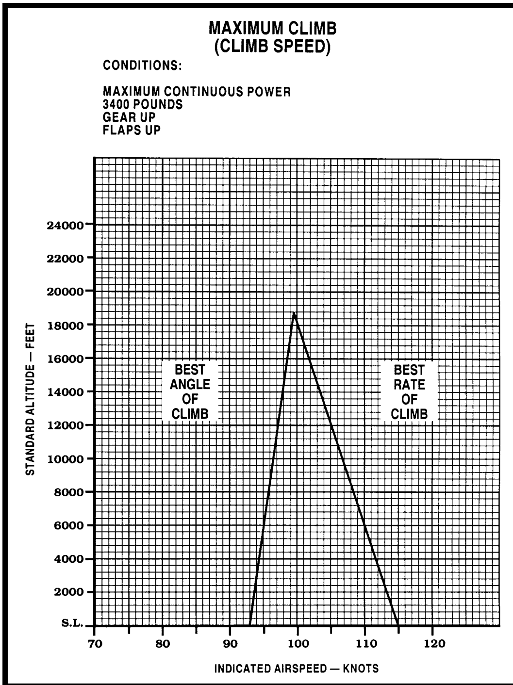
FIGURE 27.—Maximum Climb Chart.
