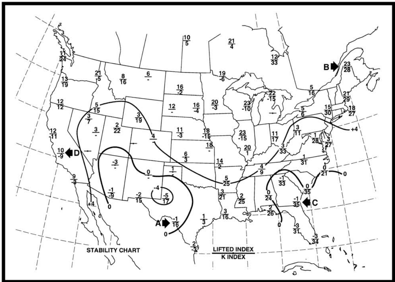
FIGURE 16.—Stability Chart.
