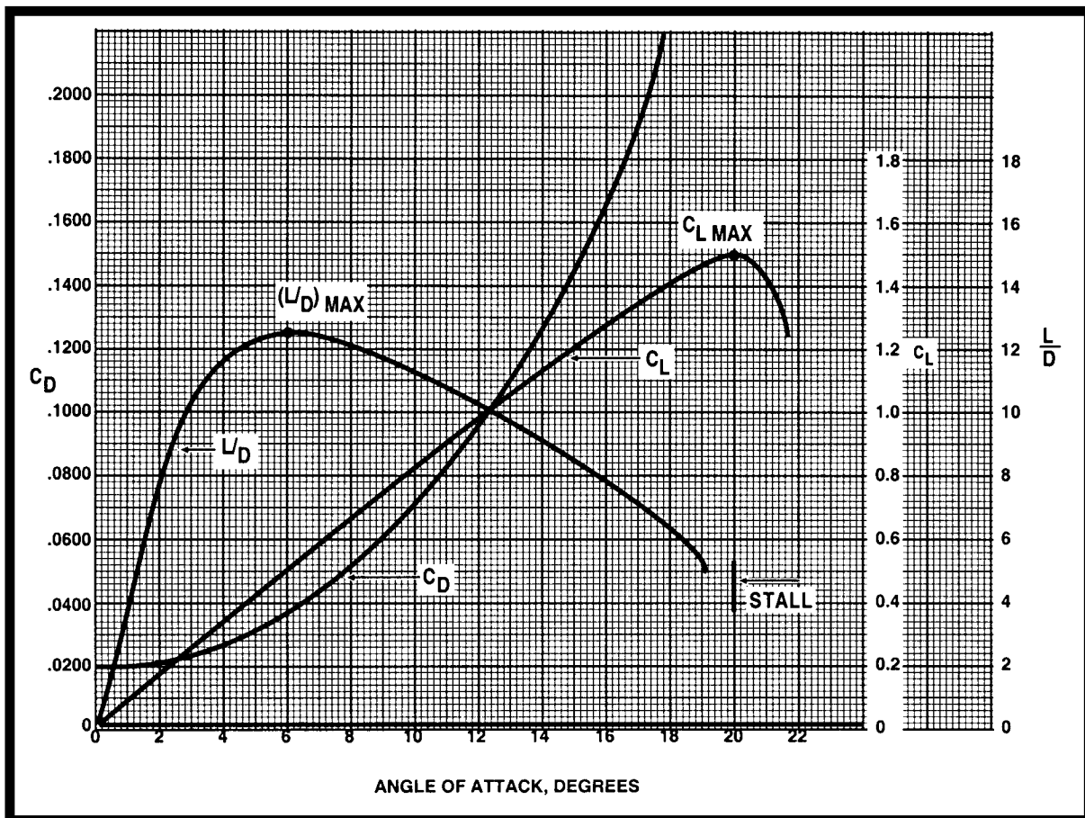
FIGURE 19.—Angle-of-Attack Chart.
