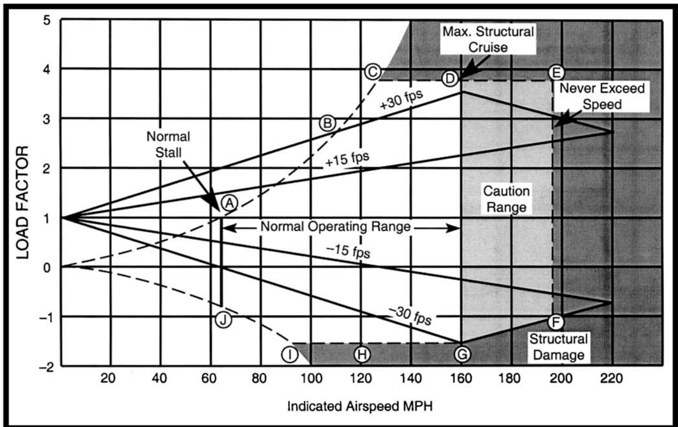
FIGURE 68.—Velocity vs. G-Loads.
