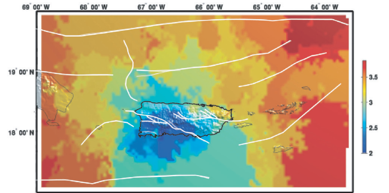
Figure 10. Geographical distribution of the magnitude of completeness values in Puerto Rico and its vicinity as determined from the Puerto Rico Seismic Network Catalog for the interval January 1986-March 2006 (adapted from Clinton and others 2006). http://redsismica.uprm.edu/spanish/tsunami/media/PRMonitoring.pdf
