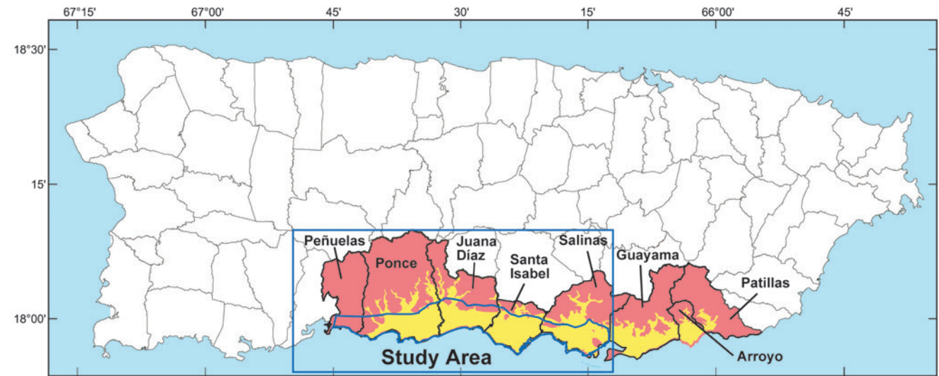
Figure 1. Location of the Peñuelas to Salinas study area. Insert shows extent of the Southern Coastal Plain of Puerto Rico (adapted from Renken and others, 2002).
