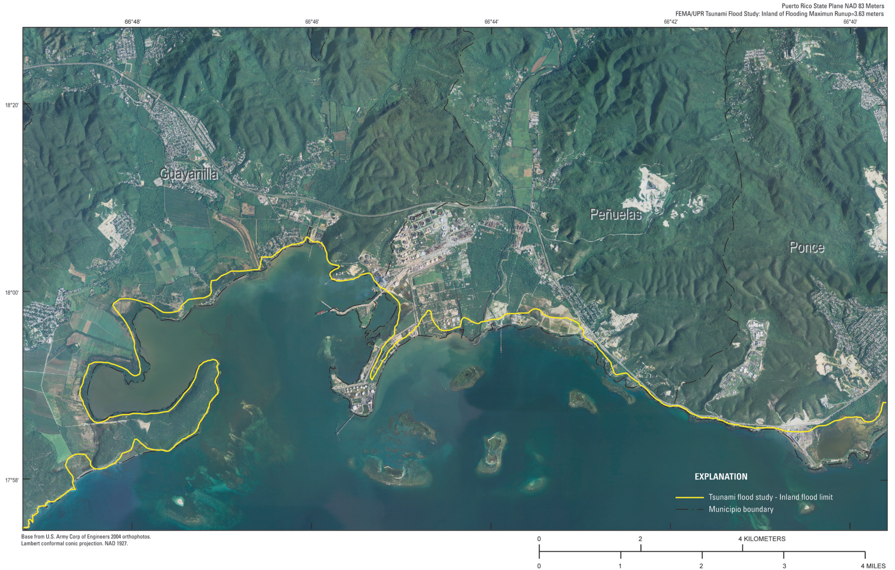
Figure 12. Inland extent of tsunami-induced flooding in the Punta Verraco and Punta Cuchara quadrangles (adapted from Mercado and Justiniano, 2007). http://coastalhazards.uprm.edu/index.html
