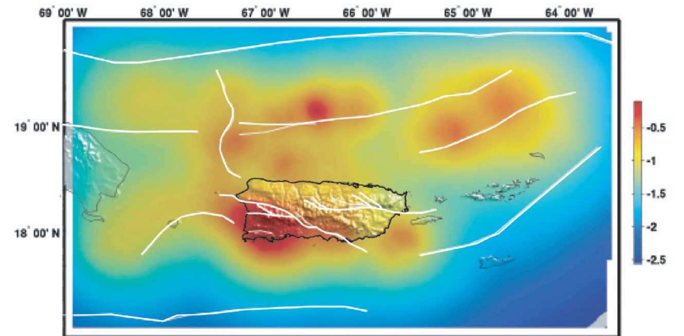
Figure 11. Seismicity density in Puerto Rico and its vicinity (adapted from Clinton and others, 2006). http://redsismica.uprm.edu/spanish/tsunami/media/PRMonitoring.pdf
