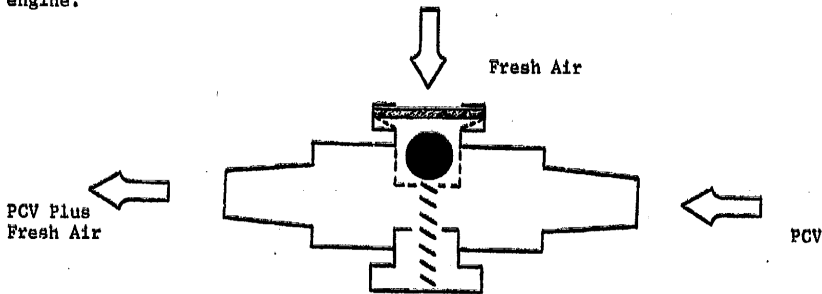
Figure 1: Cross Sectional View of the Ram-Jet
