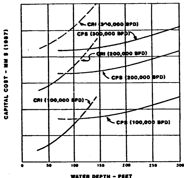
Figure 3. Production platform capital cost versus water depth - borrow source at site.
