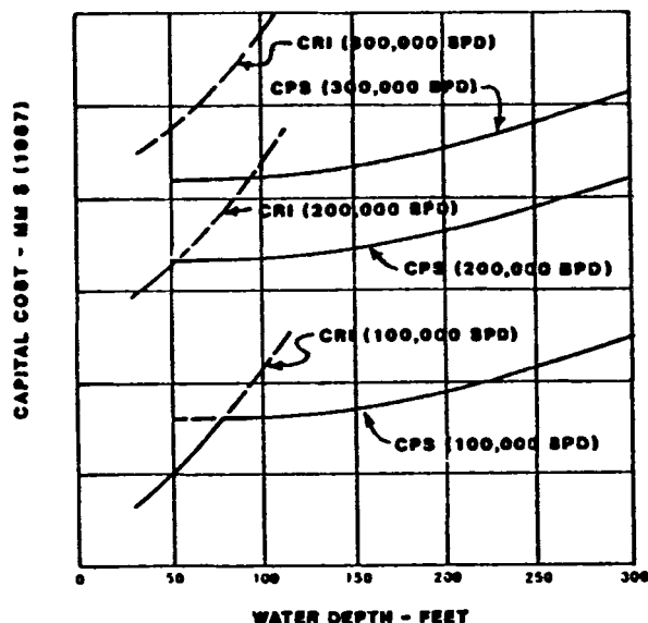
Figure 4. Production platform capital cost versus water depth - borrow source 6 mi from site.
