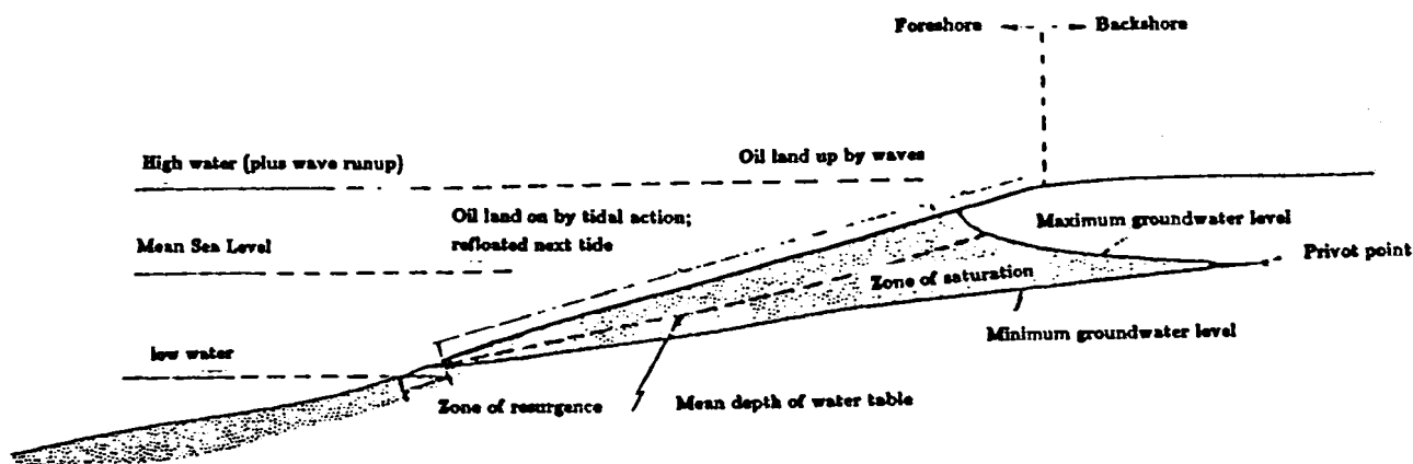
Figure 3. Schematic of beach groundwater system.
