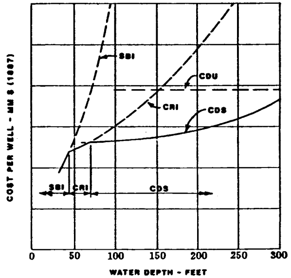
Figure 2. Per well cost versus water depth - borrow source 6 mi from site.
