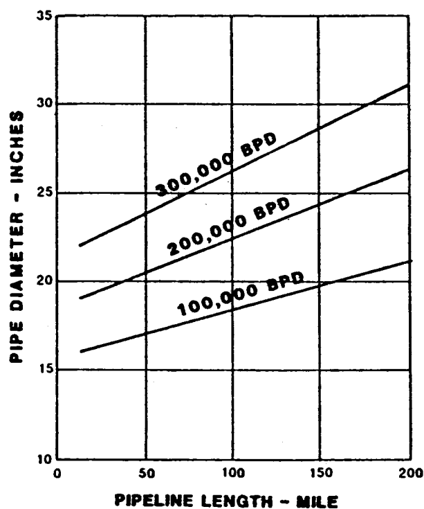
Figure 5. Marine pipeline pipe diameter versus pipeline length for various production rates.
