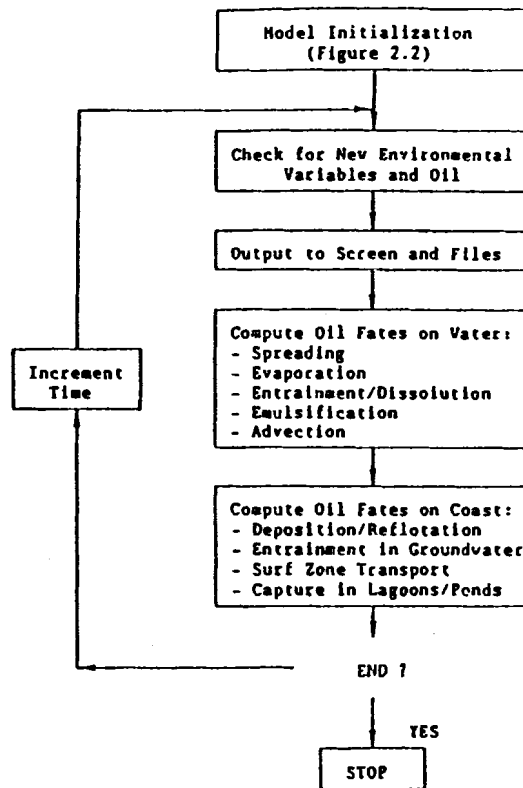
Figure 2. COZOIL model system schematic.
