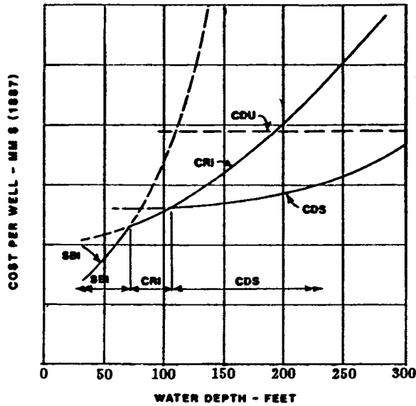
Figure 1. Per well cost versus water depth - borrow source at site.
