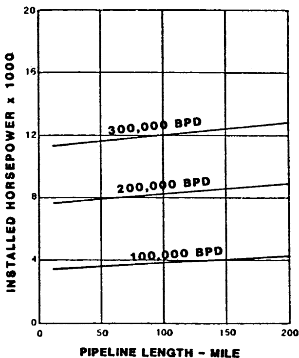
Figure 6. Marine pipeline installed horsepower versus pipeline length for various production rates.
