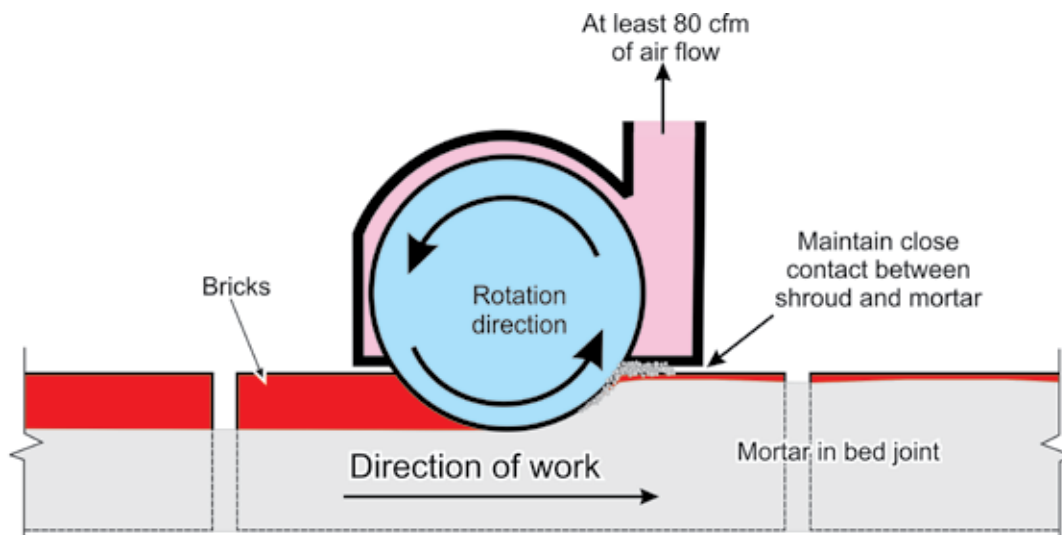
Figure 3. Diagram of mortar removal.
