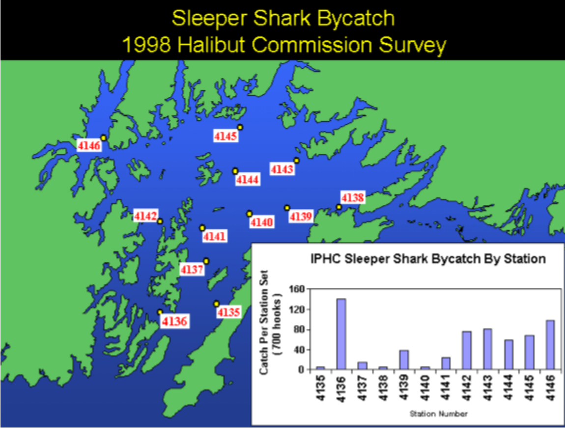
Figure 3. International Pacific Halibut Commission Pacific sleeper shark bycatch per station set (700 hooks) in Prince William Sound in 1998 (Dan Randolph, International Pacific Halibut Commission, unpublished data)
