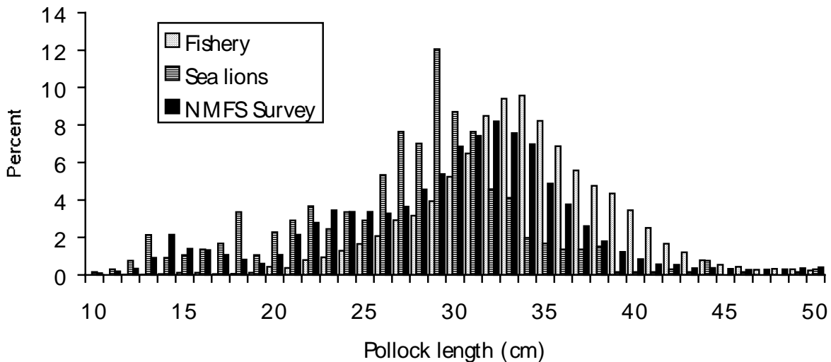
Figure.—Length frequency distributions of walleye pollock caught by the fishery, consumed by Steller sea lions, and the population based on the NMFS bottom trawl survey in spring and summer of 1981 in the Bering Sea. Fishery (April through June) and survey (July through September) length-frequencies were from collections in NMFS statistical area 521, located northwest of the Pribilof Islands. Steller sea lions (n=27) were collected pelagically in Area 521 in April. (Pollock length data computed from otoliths found in sea lion stomachs.)
