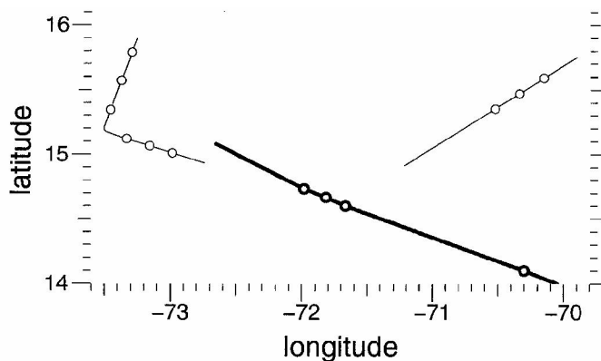
Figure 3. The thick line indicates the track of Hurricane Ivan. The three thick circles on the hurricane track line in the vicinity of 71.8^\circ\text{W} indicate the locations of the eye fixes made by the NOAA aircraft during the flight on 9 September 2004. The thin lines indicate flight segments of the NOAA aircraft and the thin circles indicate the centers of data spans used to generate the data shown in Figures 4 through 7.
