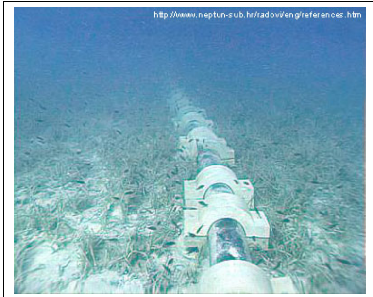
Fig.3.a Underwater sewage outlet.
