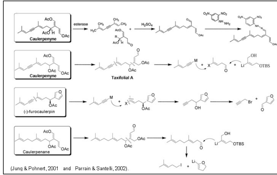
Fig.4.g Caulerpenyne reactions.
