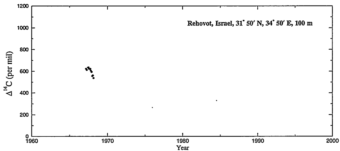
Fig. A-2. Corrected ^{14}\text{C} measurements from air samples collected at Lindesnes, Norway; Santiago de Compostela, Spain; and Rehovot, Israel
