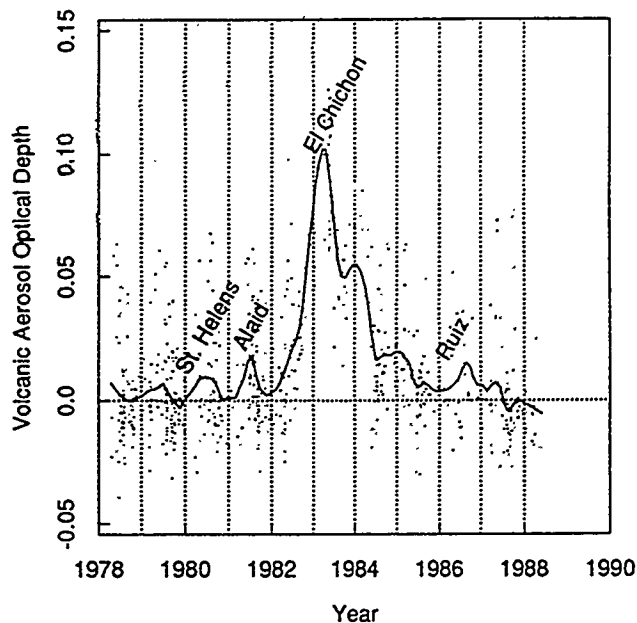
Fig. 1. Smoothed estimate of the time-dependent volcanic optical depth perturbation to the atmosphere at 785 nm. Volcano names are to be associated with their atmospheric effects.
