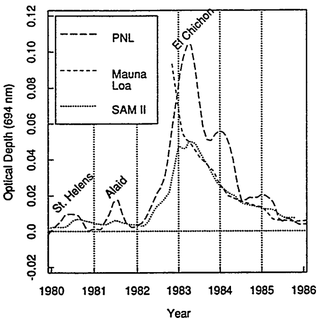
Fig. 8. Time series comparison of PNL (46.4°N), Mauna Loa (19.5°N), and SAM II (73°N) volcanic optical depths at 694.3 nm.
