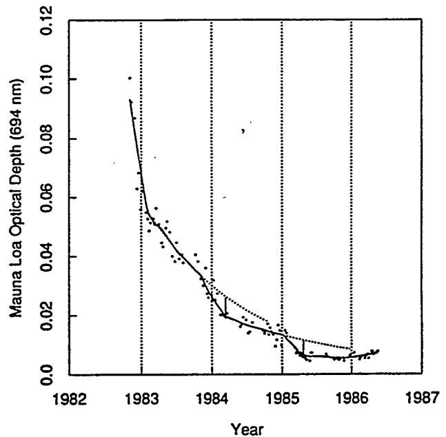
Fig. 10. The Mauna Loa data of Figure 8 expanded to define winter dips. The dotted lines are exponential fits to pre-winter data and extrapolations to expected values assuming no dips. Vertical solid lines are estimates of dip depths.
