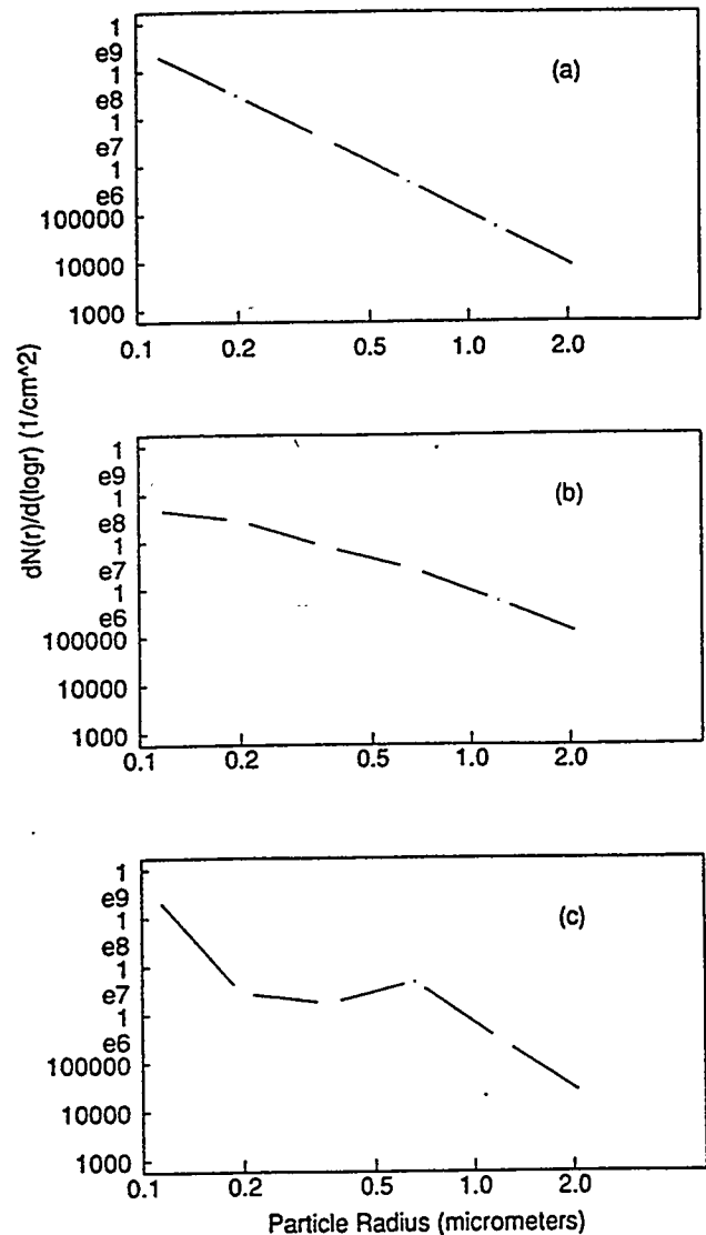
Fig. 5. Volcanic aerosol size distributions based on mathematical inversion of optical depth data (a) six months before, (b) during, and (c) six months after the peak volcanic load.
