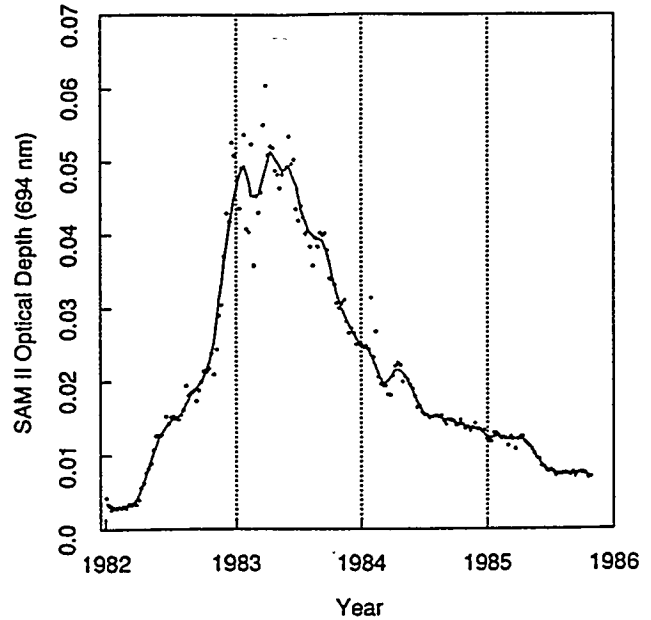
Fig. 9. Time series plot and estimate of SAM II volcanic optical depths at 694.3 nm. The time resolution of the estimate is higher here than in Figure 8, revealing more structure in the winter maxima.
