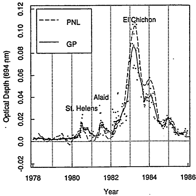
Fig. 7. Time series comparison of PNL and GP volcanic aerosol optical depths at 694.3 nm. The GP (47.5°N) data set is plotted, along with a smoothed fit to the data (solid line). The dashed line is the smoothed PNL (46.4°N) data interpolated to 694.3 nm.
