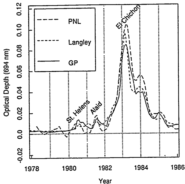
Fig. 6. Time series comparison of three distinct mid-latitude data sets of volcanic aerosol optical depth normalized to 694.3 nm.
