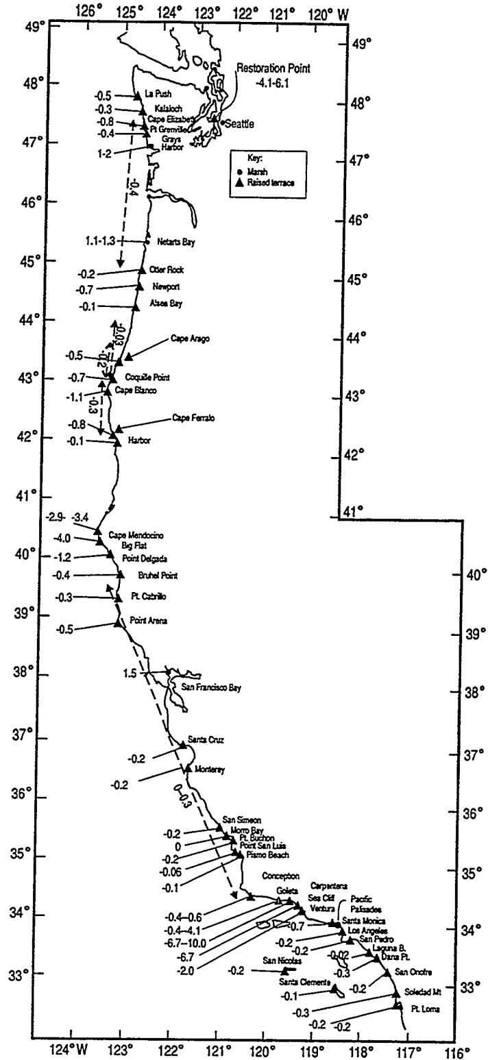
Figure 1. Information on uplift rates, in mm/yr along the West Coast from various sources listed in Table 1.
