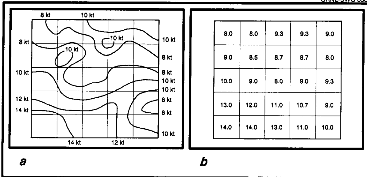
Fig. A-6. A sample conversion of a wind-speed contour map into digital data according to the derivation procedures used for data variable MONSOON. (a) Contour map of the type used for data derivation; (b) resultant digital values in knots for each 5° x 5° grid cell.
