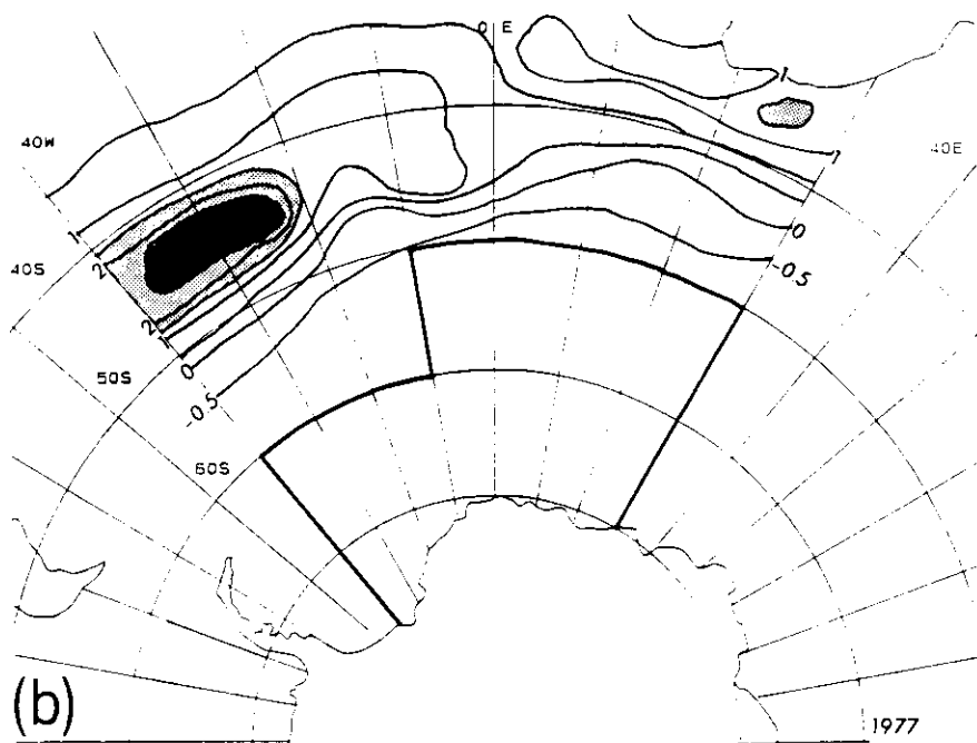
Figure 10. Similar to Figure 9, except for the South Atlantic in the (a) 1978 and (b) 1977 winters
