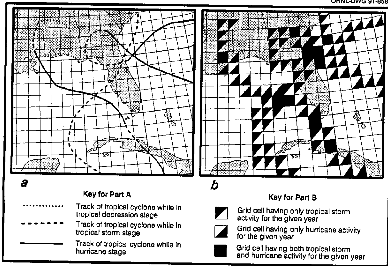
Fig. A-2. Tropical cyclone activity for a given year for 1^{\circ} \times 1^{\circ} latitude-longitude grid cells as interpreted from an annual tropical cyclone tracking chart. (a) Theoretical annual tropical cyclone tracking chart; (b) tropical cyclone activity as interpreted from (a).
