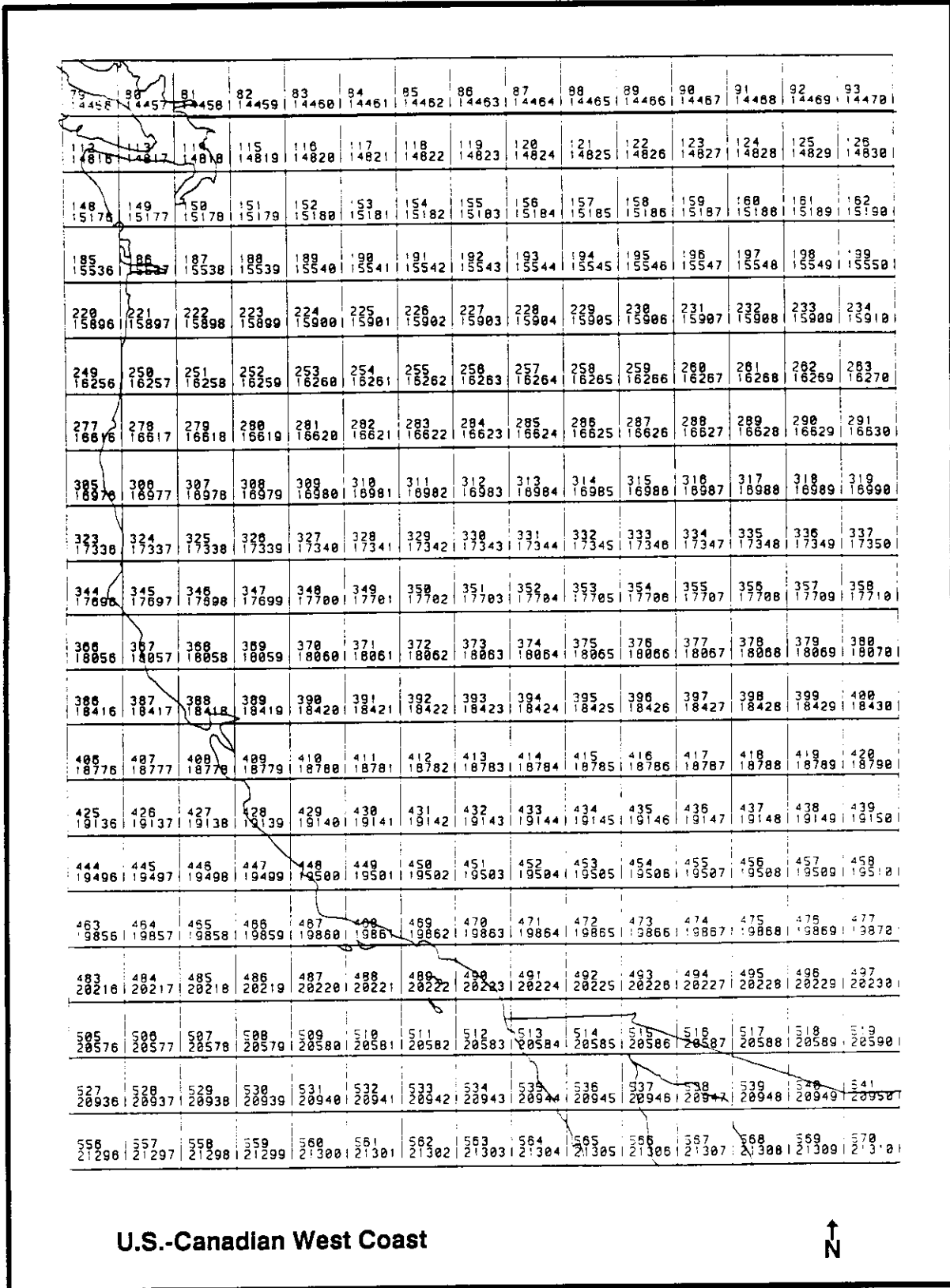
Fig. 1 (Page 2 of 6). Spatial coverage of the tropical storm and hurricane probabilities of occurrence described in Sect. 7.1 showing 1° x 1° grid cell (polygon) locations and ID numbers (top numbers refer to ARC/INFO™ coverage IDs; bottom numbers refer to flat ASCII file IDs).
