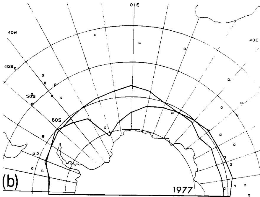
Figure 8. Similar to Figure 6, except for the South Atlantic sector in the (a) 1978 and (b) 1977 winters
