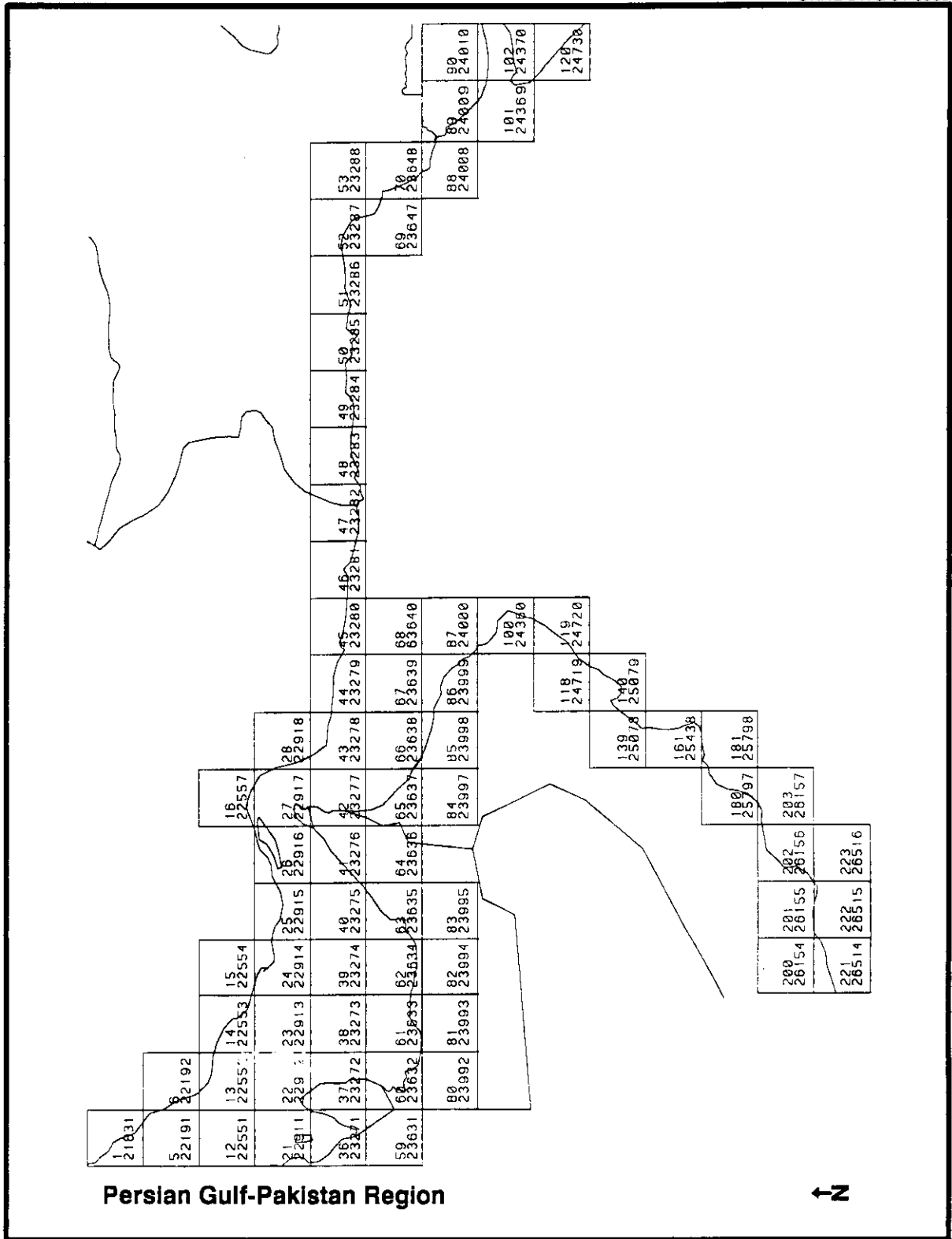
Fig. 11 (Page 4 of 12). Spatial coverage of the index of winds on coastlines in the African, Asian, and Australian monsoon regions described in Sect. 12.1 showing 1° x 1° grid cell (polygon) locations and ID numbers (top numbers refer to ARC/INFO™ coverage IDs; bottom numbers refer to flat ASCII file IDs).
