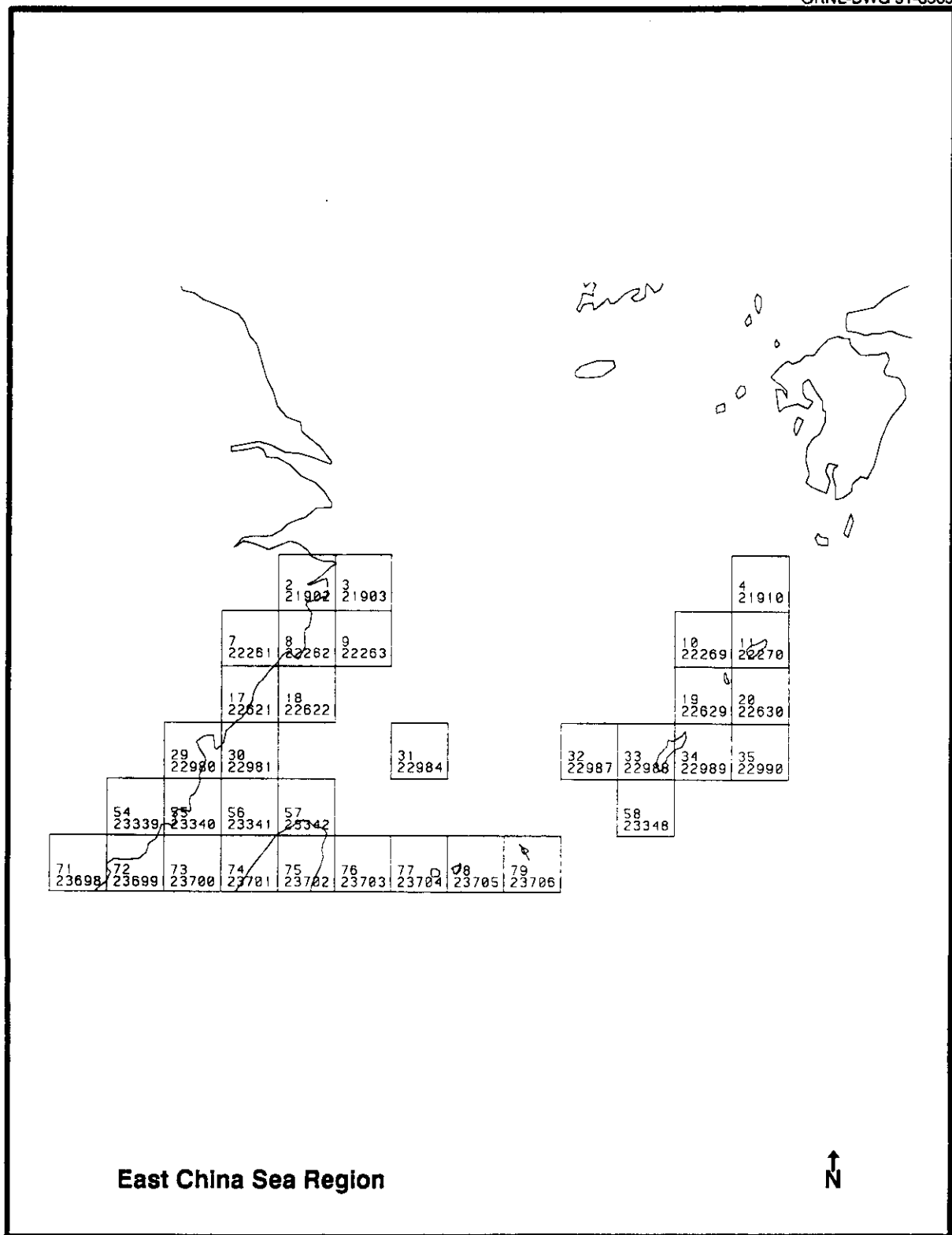
Fig. 11 (Page 8 of 12). Spatial coverage of the index of winds on coastlines in the African, Asian, and Australian monsoon regions described in Sect. 12.1 showing 1° x 1° grid cell (polygon) locations and ID numbers (top numbers refer to ARC/INFO™ coverage IDs; bottom numbers refer to flat ASCII file IDs).
