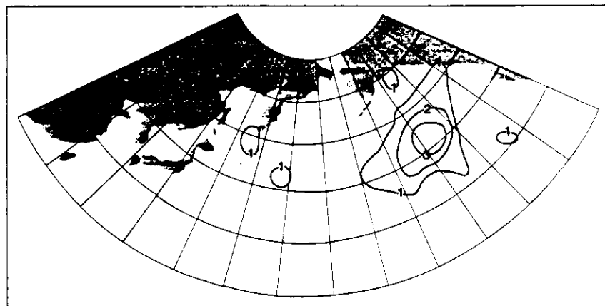
Figure 5. Observed number of instant occlusions (type 3) (contour interval = 1)
