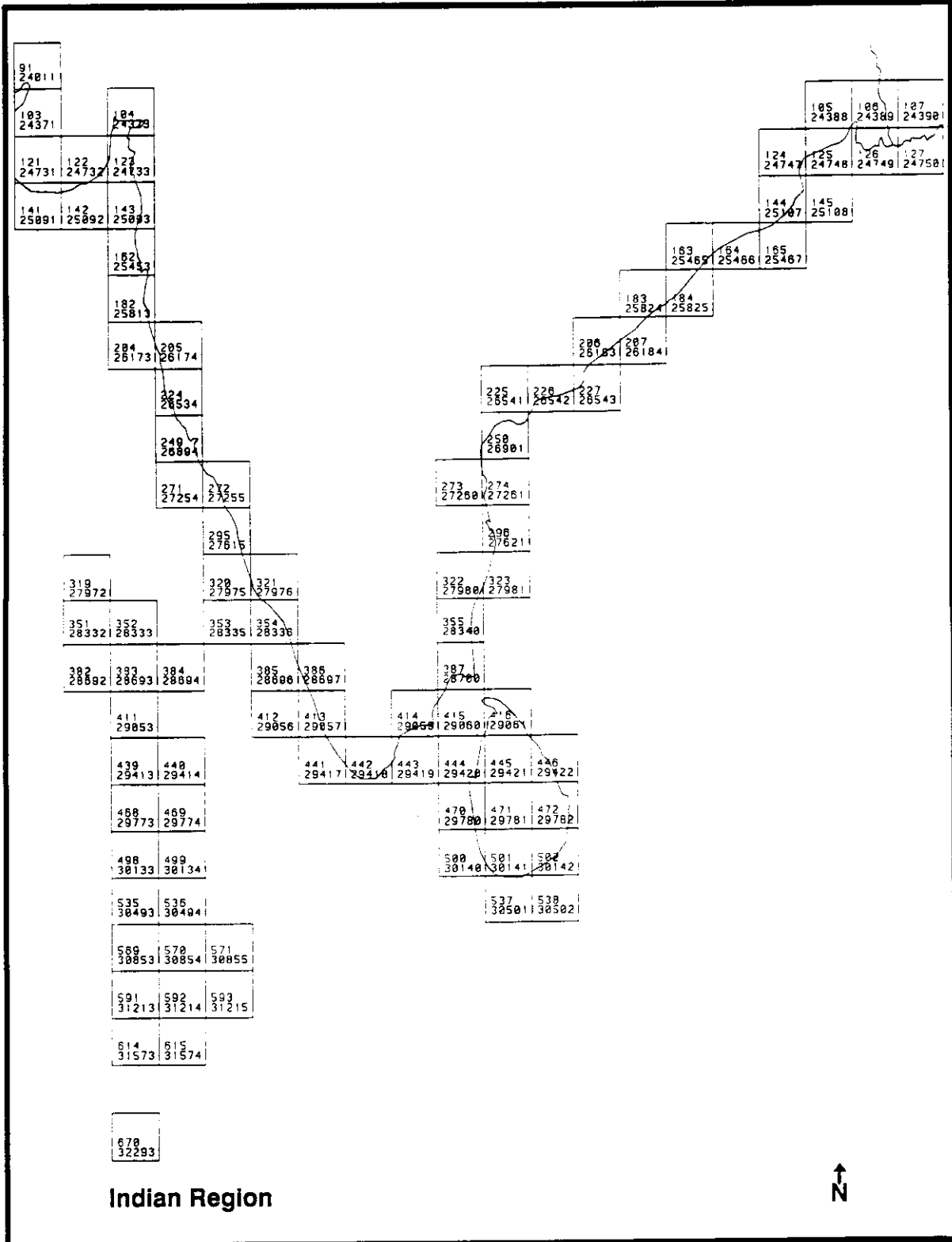
Fig. 11 (Page 5 of 12). Spatial coverage of the index of winds on coastlines in the African, Asian, and Australian monsoon regions described in Sect. 12.1 showing 1° x 1° grid cell (polygon) locations and ID numbers (top numbers refer to ARC/INFO™ coverage IDs; bottom numbers refer to flat ASCII file IDs).
