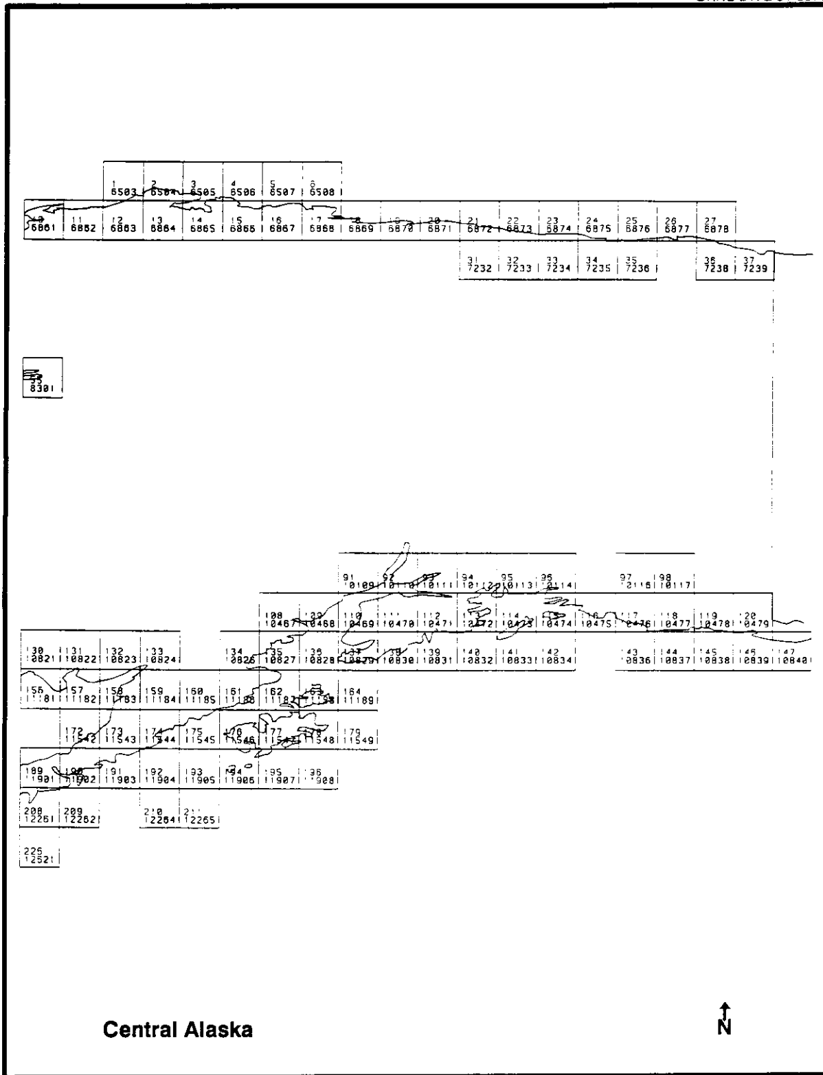
Fig. 12 (Page 3 of 5). Spatial coverage of the sea-ice concentration data values described in Sect. 13.1 showing 1° x 1° grid cell (polygon) locations and ID numbers (top numbers refer to ARC/INFO™ coverage IDs; bottom numbers refer to flat ASCII file IDs).
