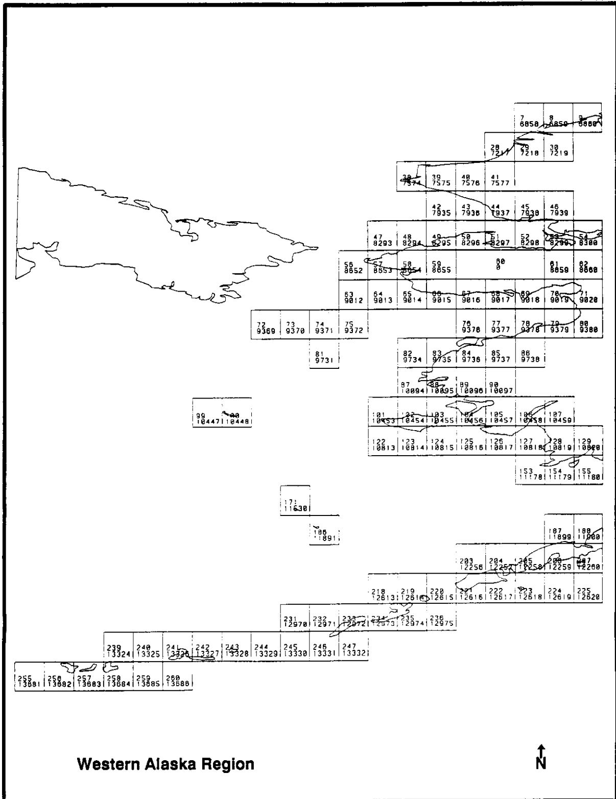
Fig. 12 (Page 2 of 5). Spatial coverage of the sea-ice concentration data values described in Sect. 13.1 showing 1° x 1° grid cell (polygon) locations and ID numbers (top numbers refer to ARC/INFO™ coverage IDs; bottom numbers refer to flat ASCII file IDs).
