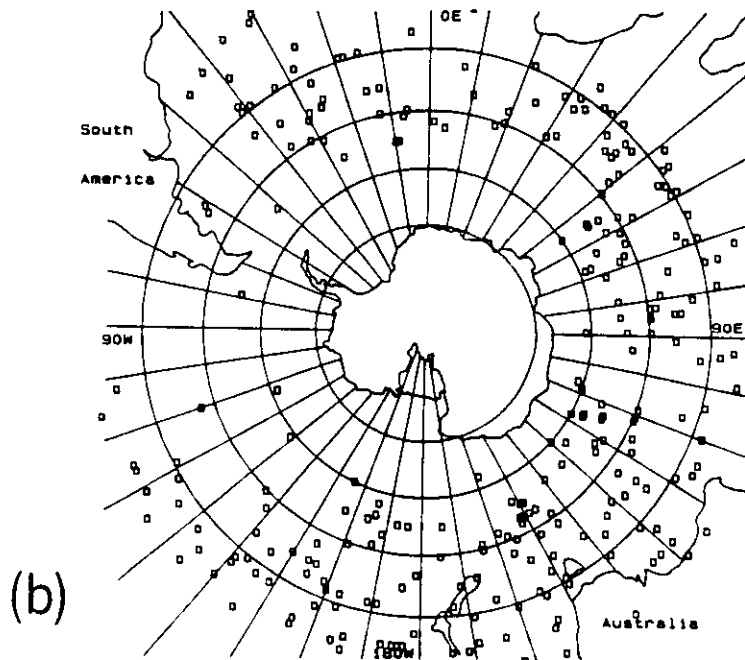
Figure 4. Locations of all frontal wave vortices in the genesis (type 1) through to mature (type 8) stages of development for (a) June and (b) September, winters 1977-1983
