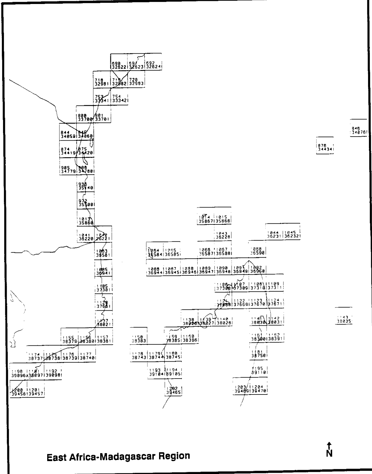
Fig. 11 (Page 3 of 12). Spatial coverage of the index of winds on coastlines in the African, Asian, and Australian monsoon regions described in Sect. 12.1 showing 1° x 1° grid cell (polygon) locations and ID numbers (top numbers refer to ARC/INFO™ coverage IDs; bottom numbers refer to flat ASCII file IDs).
