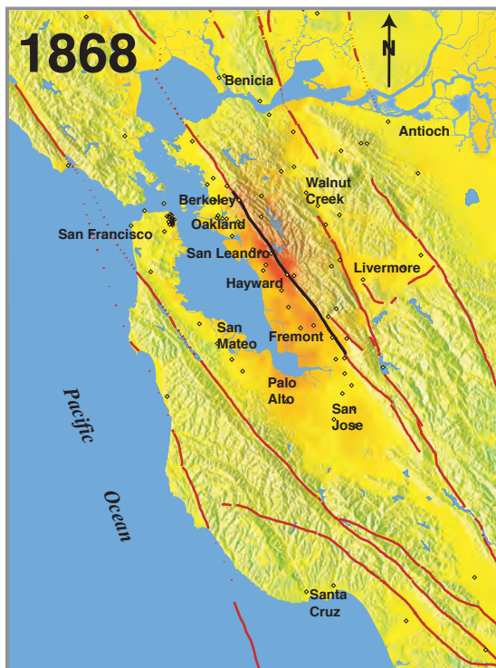
A ShakeMap showing the inferred intensity of ground shaking in the 1868 earthquake (MMI, or Modified Mercalli Intensity), compared to a ShakeMap for the 1989 magnitude 6.9 Loma Prieta earthquake. Red lines are earthquake faults; black line shows the portion of the Hayward Fault that ruptured in 1868; yellow star marks the epicenter of the 1989 quake. Diamonds show locations of damage reports (1868) and of seismic recordings (1989).
