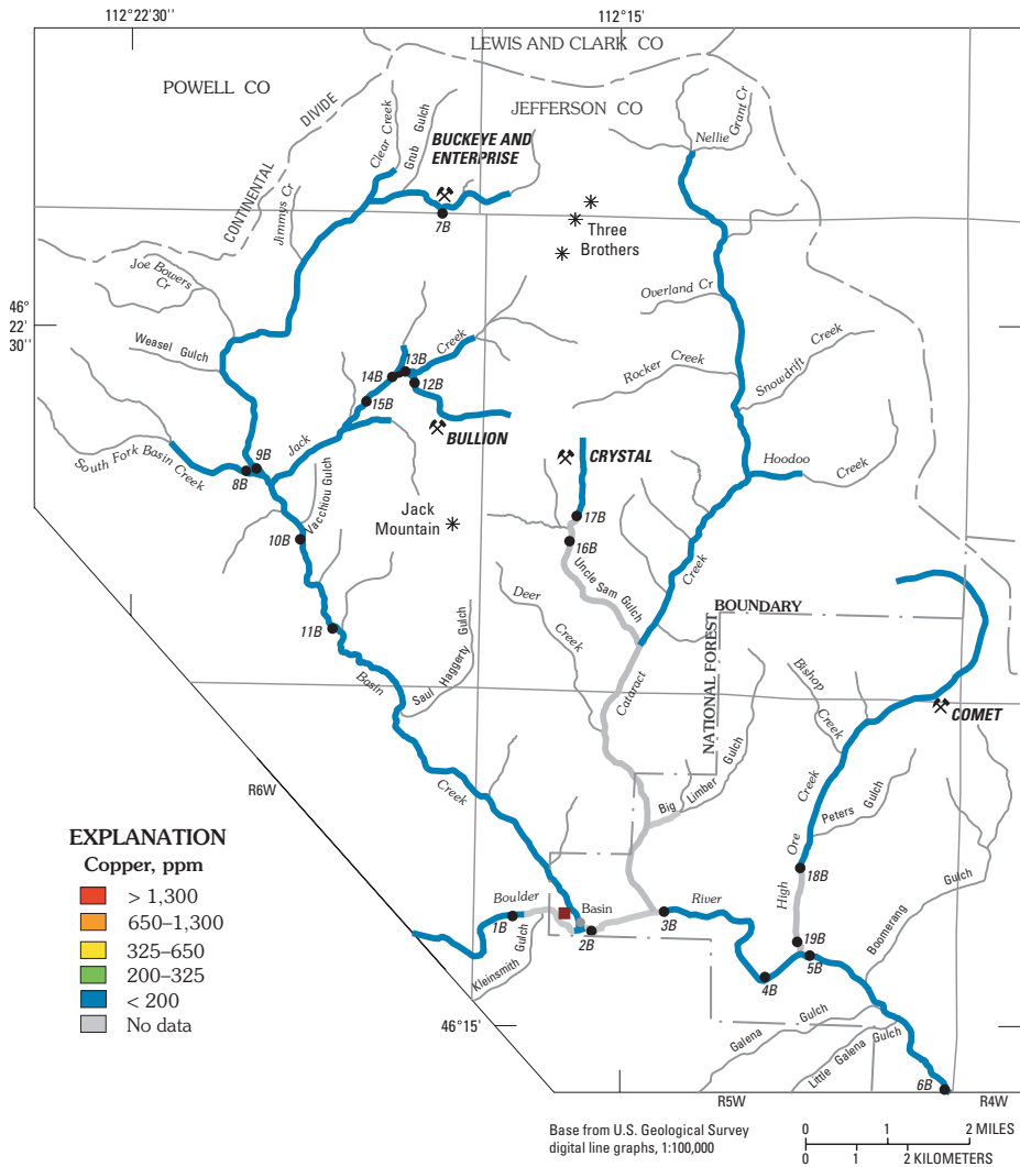
Figure 19. Concentrations of copper (ppm) in premining streambed sediment (solid dot) of Boulder River watershed study area. Stream reaches shown in gray, no data. Concentration intervals are same as in figure 4. Note that all stream reaches where we determined premining geochemical baseline have concentrations of copper below 200 ppm, that is, less than six times baseline value of 32 ppm (table 1). Dark-red square, Jib Mill site.
