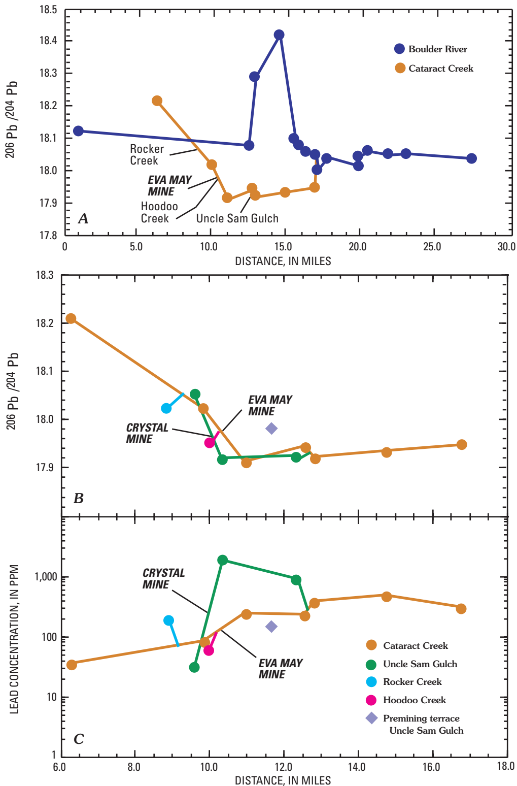
Figure 25. Profile plots of lead isotopic composition (A, B) and lead concentration (C) determined in streambed sediment. A, ^{206}\text{Pb}/^{204}\text{Pb} versus distance on Boulder River and Cataract Creek. B, ^{206}\text{Pb}/^{204}\text{Pb} versus distance on Cataract Creek and Uncle Sam Gulch. C, Concentration of lead in streambed sediment of Cataract Creek and Uncle Sam Gulch versus distance. Note small difference in lead isotopic composition versus the great difference in lead concentration in premining versus modern streambed sediment in Uncle Sam Gulch.
