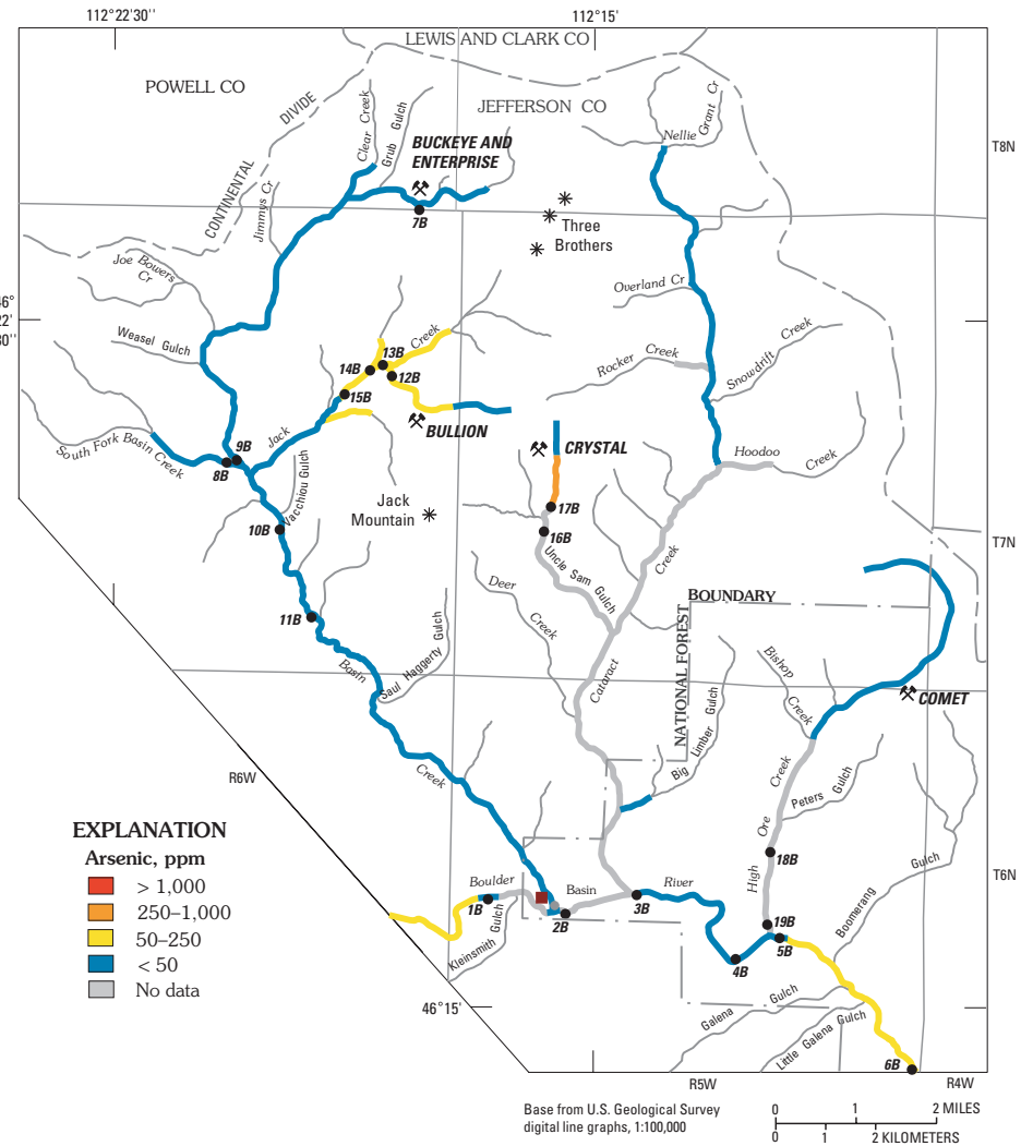
Figure 22. Concentrations of arsenic (ppm) in premining streambed sediment (solid dot) of Boulder River watershed study area. Reaches shown in gray, no data. Concentration intervals the same as in figure 7. Note that many stream reaches where we have been able to determine premining geochemical baseline have concentrations of arsenic below 50 ppm (table 1; arsenic has a median value of 35 ppm). However, downstream from Bullion and Crystal mines, arsenic concentrations were elevated. Dark-red square, Jib Mill site.
