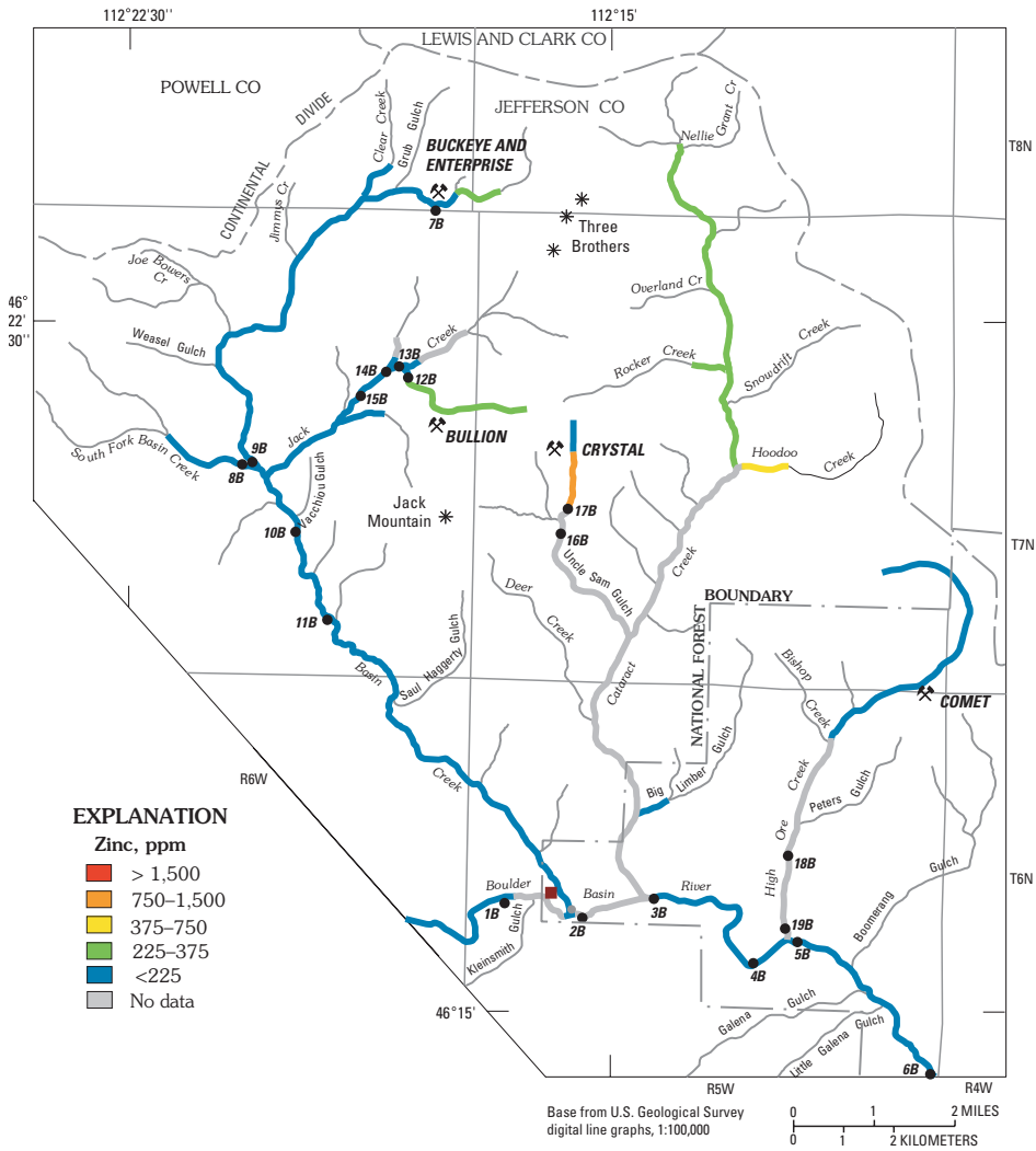
Figure 21. Concentrations of zinc (ppm) in premining streambed sediment (solid dot) of Boulder River watershed study area. Stream reaches shown in gray, no data. Concentration intervals are same as in figure 6. Note that many stream reaches where we have been able to determine premining geochemical baseline have concentrations of zinc below 200 ppm, that is, less than 1.5 times the baseline value of 150 ppm (table 1), with the exception of the reach downstream from Crystal mine in Uncle Sam Gulch at site 17B. Dark-red square, Jib Mill site.
