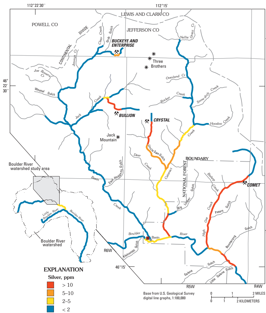
Figure 8. Concentrations of silver from total-digestion data from streambed sediment collected from major tributaries during current study. Dark-red square, Jib Mill site.
