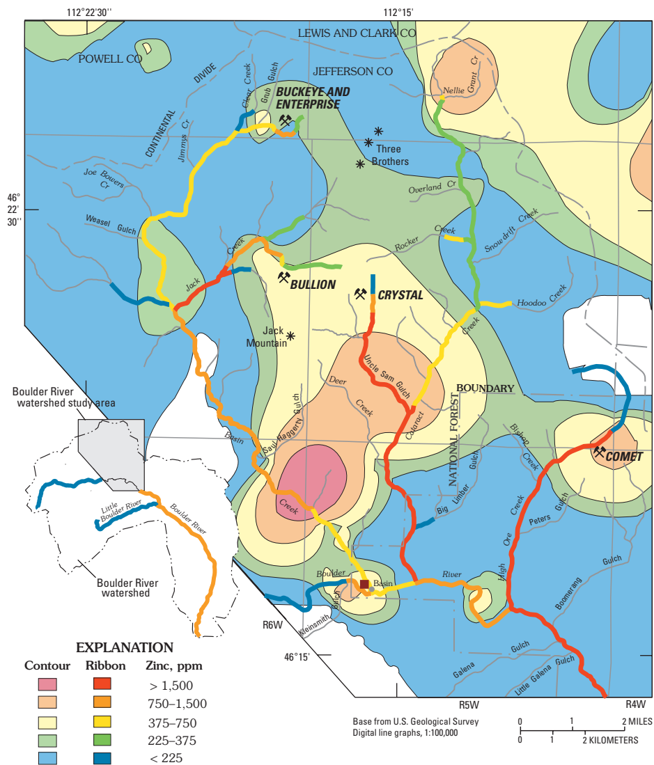
Figure 6. Regional geochemistry for zinc from total-digestion data from NURE streambed-sediment data (Broxton, 1980) showing contrast with zinc concentrations in streambed sediment from major tributaries. White, sample density insufficient to allow projection of geochemical surface using a 3,281-ft (1,000-m) grid-cell density. Dark-red square, Jib Mill site.
