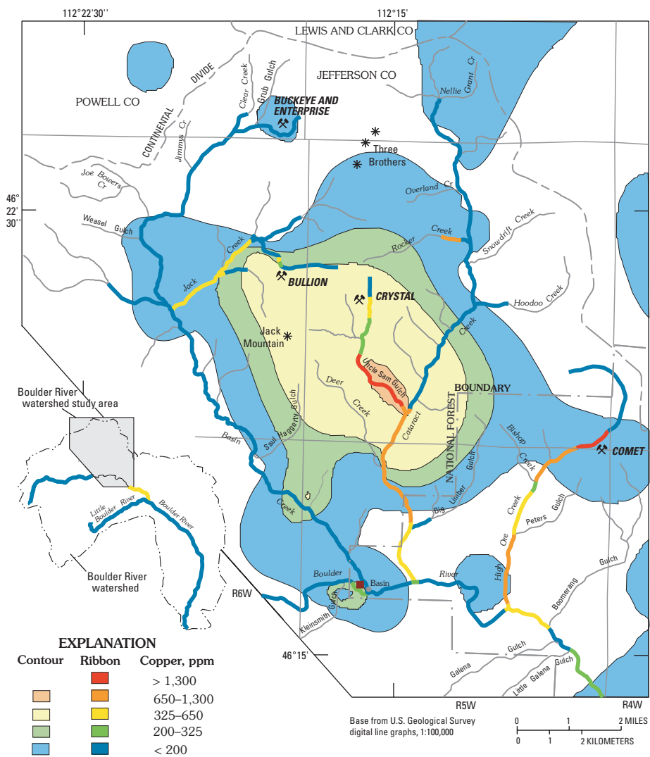
Figure 4. Regional geochemistry for copper from total-digestion data from NURE streambed-sediment data (Broxton, 1980) showing contrast with copper concentrations in streambed sediment from major tributaries. White, sample density insufficient to allow projection of geochemical surface using a 3,281-ft (1,000-m) grid-cell density. Dark-red square, Jib Mill site.
