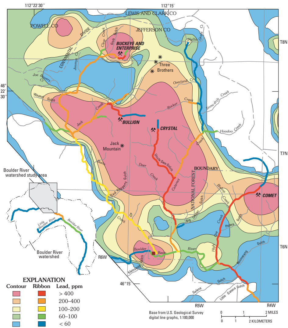
Figure 5. Regional geochemistry for lead from total-digestion data from NURE streambed-sediment data (Broxton, 1980) showing contrast with lead concentrations in streambed sediment from major tributaries. White, sample density insufficient to allow projection of geochemical surface using a 3,281-ft (1,000-m) grid-cell density. Dark-red square, Jib Mill site.
