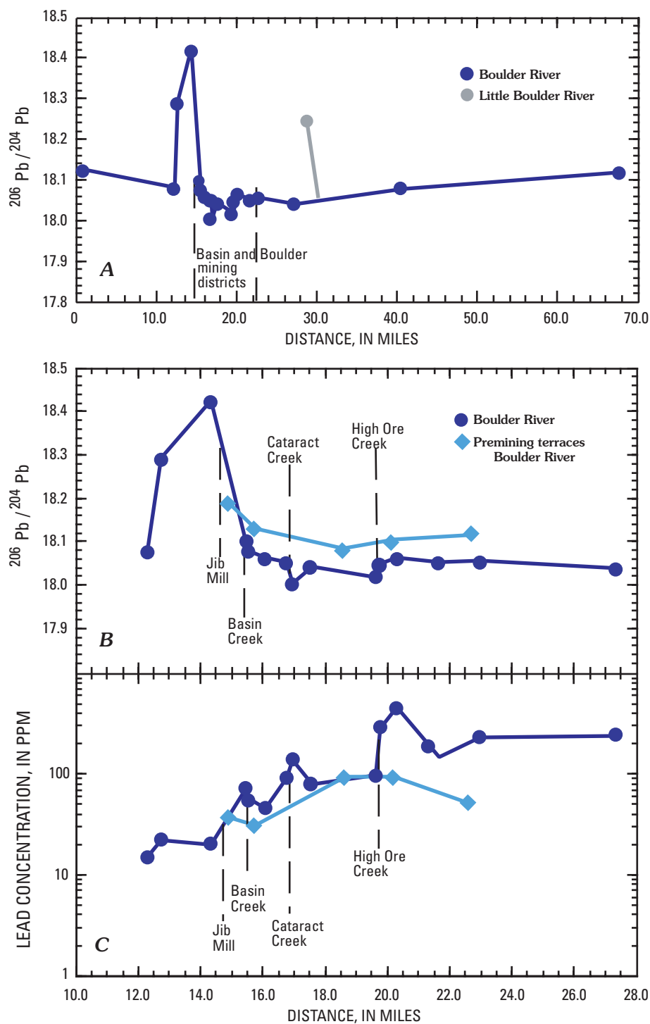
Figure 27. Profile plots of lead isotopic composition ( A , B ) and lead concentration ( C ) determined in streambed sediment. A , ^{206}\text{Pb}/^{204}\text{Pb} versus distance on Boulder River. B , ^{206}\text{Pb}/^{204}\text{Pb} at larger-scale intervals for streambed sediment on Boulder River and premining terrace deposits (sites in fig. 18). C , Concentration of lead in streambed sediment today and in streambed sediment from premining terrace samples versus distance on Boulder River.
