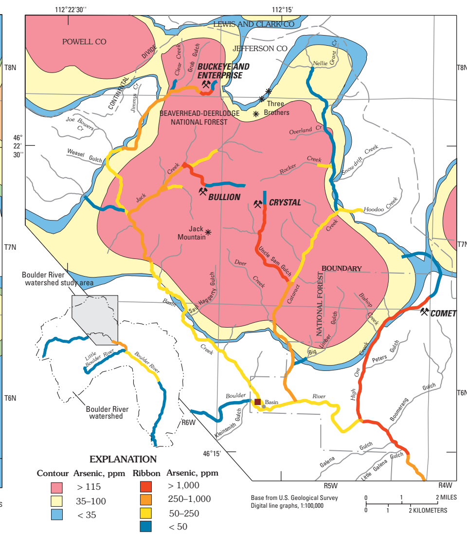
Figure 7. Regional geochemistry for total arsenic from analysis of streambed sediment from Butte 1° x 2° study (McDanal and others, 1985) showing contrast with arsenic concentrations in streambed sediment from major tributaries. White, sample density insufficient to allow projection of geochemical surface using a 3,281-ft (1,000-m) grid-cell density. Dark-red square, Jib Mill site.
