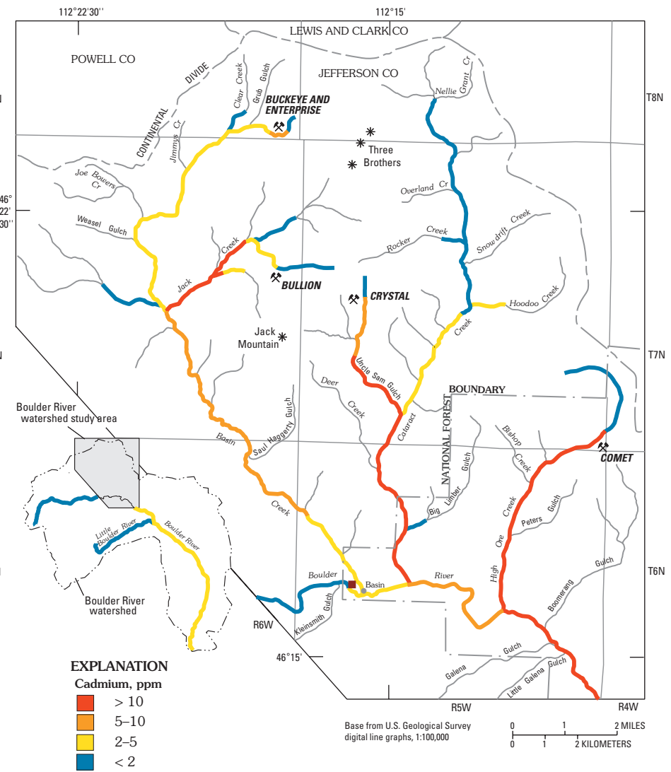
Figure 9. Concentrations of cadmium from total-digestion data from streambed sediment collected from major tributaries during current study. Dark-red square, Jib Mill site.
