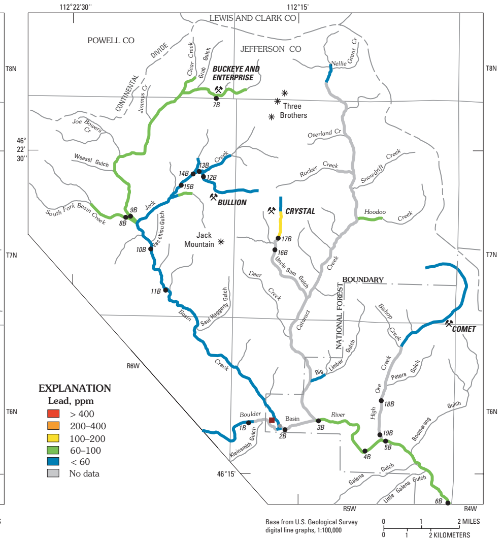
Figure 20. Concentrations of lead (ppm) in premining streambed sediment (solid dot) of Boulder River watershed study area. Stream reaches shown in gray, no data. Concentration intervals are same as in figure 5. Note that many stream reaches where we have been able to determine premining geochemical baseline have concentrations of lead below 80 ppm, that is, about twice the baseline value of 35 ppm (table 1), with the exception of the reach downstream from Crystal mine in Uncle Sam Gulch at site 17B. Dark-red square, Jib Mill site.
