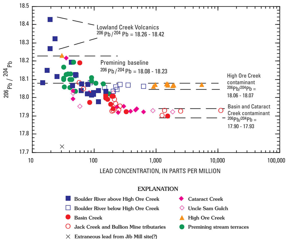
Figure 23. Plot of concentration of lead versus isotopic composition of lead ( ^{206}\text{Pb}/^{204}\text{Pb} ) showing the dominant effect of mixing of contaminant lead derived from mining on isotopic composition of leachable lead in streambed sediment. Analytical error for lead isotopic data is smaller than the symbol. Note limited range in lead isotopic compositions.
