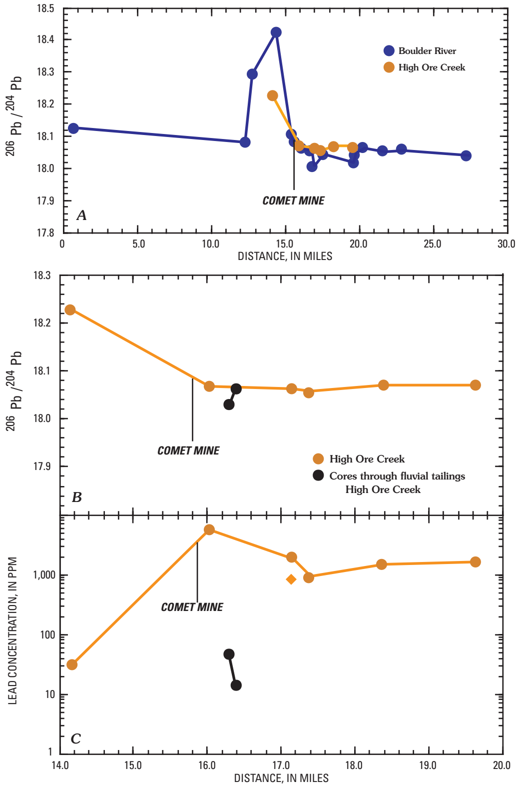
Figure 26. Profile plots of lead isotopic composition ( A , B ) and lead concentration ( C ) determined in streambed sediment. A , ^{206}\text{Pb}/^{204}\text{Pb} versus distance on Boulder River and High Ore Creek. B , ^{206}\text{Pb}/^{204}\text{Pb} versus distance on High Ore Creek. C , Concentration of lead in streambed sediment from High Ore Creek versus distance. Note small difference in lead isotopic composition relative to the large difference in lead concentration in premining versus modern streambed sediment in High Ore Creek.
