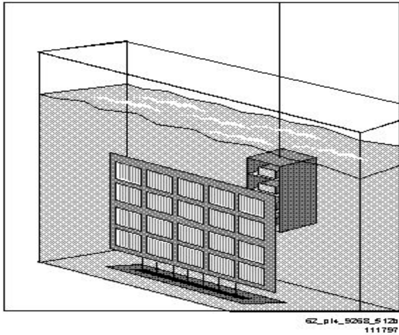
Figure 1 Underwater Irradiator. The sealed sources remain in the water at all times. The product to be irradiated is placed in a water-tight container and lowered into the water.
