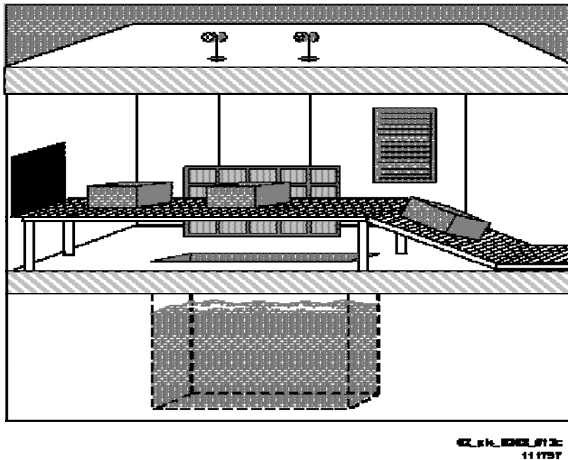
Figure 2 Commercial Wet-Source-Storage Irradiator. The sealed sources are stored in water and raised into the air to irradiate a product that may be moved into the irradiation room on a conveyor system. This is an example of a panoramic wet-source-storage irradiator.
