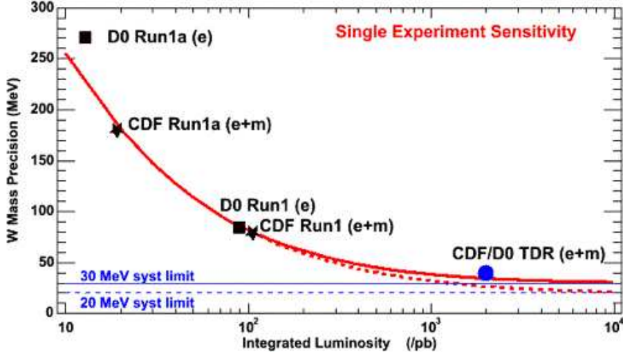
Figure 1: Projection for the expected precision of a single experiment W mass measurement as a function of integrated luminosity based on Run I Tevatron measurements.
