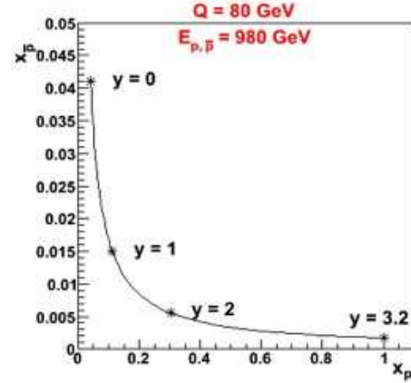
Figure 21: The interacting partons' momentum fractions required to produce a W boson ( Q = 80 \text{ GeV} ). The larger the difference between x_p and x_{\bar{p}} , the greater the rapidity of the produced boson.
