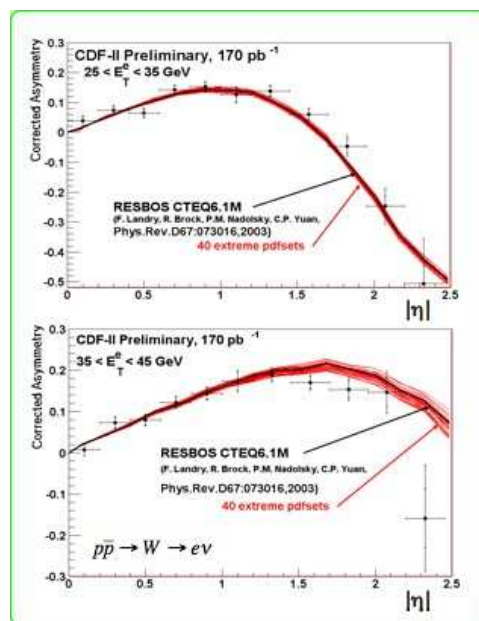
Figure 25: CDF lepton charge asymmetry measurement based on W \rightarrow e\nu events. The measurement is compared to a theoretical calculation based on the CTEQ PDF model.
