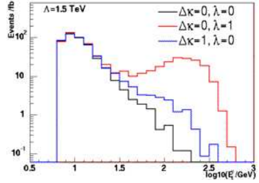
Figure 13: The predicted shape of a generic diboson cross section as a function of E_T for different values of \lambda and \Delta\kappa .
