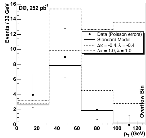
Figure 14: Comparison of leading lepton p_T distribution for D\bar{0} WW candidate events observed in the dilepton final state with SM and non-SM expectations.
