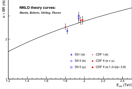
Figure 17: Summary of Tevatron inclusive W boson cross section measurements as a function of E_{CM} compared to a NNLO theoretical calculation (solid black line).
