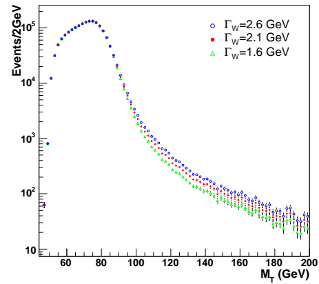
Figure 3: D\bar{O} simulation of the M_T distribution for W \rightarrow e\nu events as a function of W boson width.
