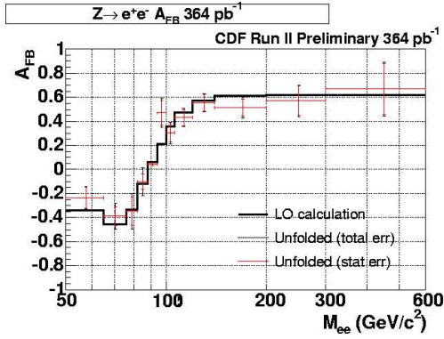
Figure 7: CDF Measurement of the forward-backward asymmetry in \gamma^*/Z \rightarrow ee events as a function of the di-electron invariant mass.
