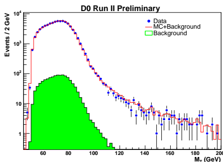
Figure 4: D\bar{O} fit to the M_T distribution of W \rightarrow e\nu events used to measure the W width.
