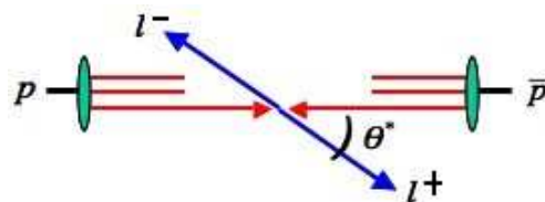
Figure 6: Illustration of \gamma^*/Z decay in the parton-parton center of mass frame. Forward (backward) events are defined as those with positive (negative) \cos(\theta^*) .
