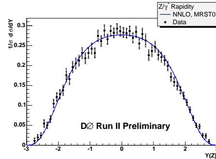
Figure 22: Differential Z boson cross section measured by DØ as a function of boson rapidity. The measured cross section is in good agreement with a NNLO theoretical prediction based on MRST PDFs (solid line).
