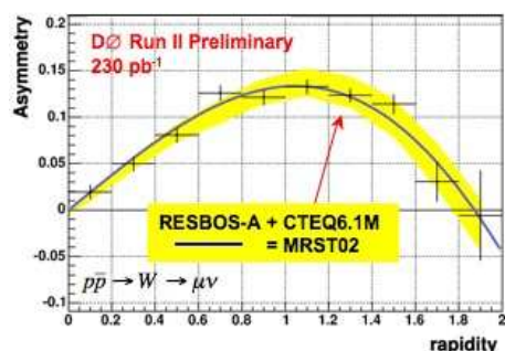
Figure 24: D0 lepton charge asymmetry measurement based on W \rightarrow \mu\nu events. The measurement is compared to a theoretical calculation based on the CTEQ and MRST PDF models.
