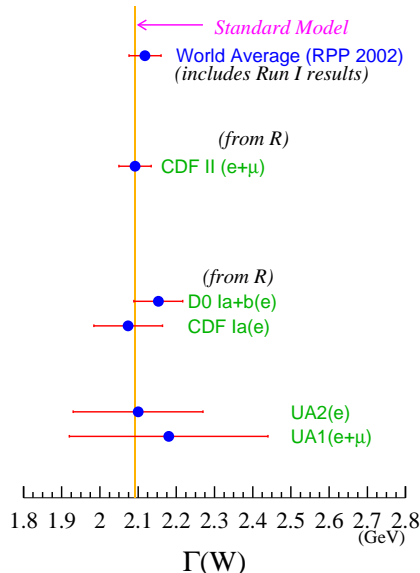
Figure 5: Comparison of the CDF indirect width measurement with previous results and the SM prediction.
