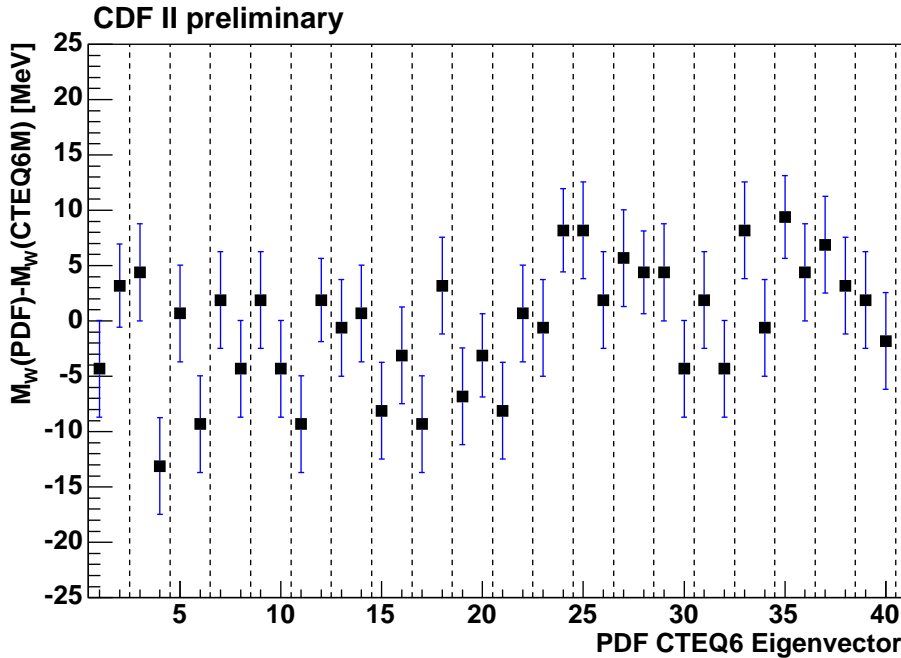
Figure 16: An example of how CTEQ “error” PDF sets are used to determine an overall PDF uncertainty. The shift in the measured W boson mass from its central value is obtained for Monte Carlo templates generated with each of the 40 error PDF sets. The observed shifts associated with each of the twenty orthogonal eigenvectors are added in quadrature to determine the total uncertainty.
