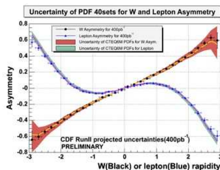
Figure 26: Comparison of the potential PDF sensitivities for lepton charge asymmetry and W boson production asymmetry measurements made with a common set of simulated candidate events corresponding to a luminosity of 400 \text{ pb}^{-1} .
