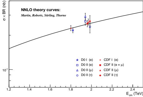
Figure 18: Summary of Tevatron inclusive Z boson cross section measurements as a function of E_{CM} compared to a NNLO theoretical calculation (solid black line).
