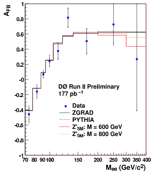
Figure 8: D0 Measurement of the forward-backward asymmetry in \gamma^*/Z \rightarrow ee events as a function of the di-electron invariant mass.
