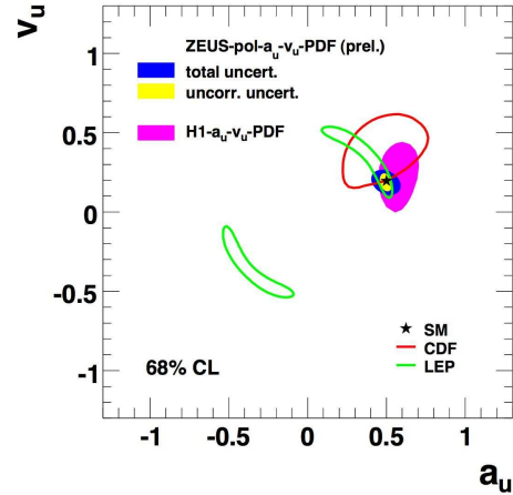
Figure 9: Comparison of the limits on the allowed range of values for the up quark axial and vector neutral current couplings obtained from Tevatron ( 72 \text{ pb}^{-1} ), HERA, and LEP measurements.
