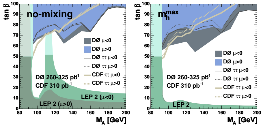
FIGURE 4. Excluded parameter space for the m_h^{\max} and no-mixing benchmark scenarios from the searches for neutral MSSM bosons. The lines show the exclusions from the D\emptyset and CDF searches for \phi \rightarrow \tau\tau . The excluded regions from combining the D\emptyset results in the \phi \rightarrow \tau\tau and the \phi b\bar{b} \rightarrow b\bar{b}b(\bar{b}) channels are shown as shaded areas.
