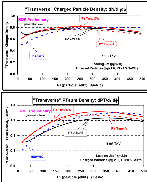
Fig. 7. Predictions at 1.96 TeV of PYTHIA Tune DW (DWT), HERWIG, and the ATLAS Tune for the density of charged particles, dN/d\eta d\phi ( top ), and the charged PTsum density, dPT/d\eta d\phi ( bottom ), with p_T > 0.5 GeV/c and |\eta| < 1 in the “transverse” region for “leading jet” events as a function of the leading jet P_T . Tune DW and DWT are identical at 1.96 TeV.
