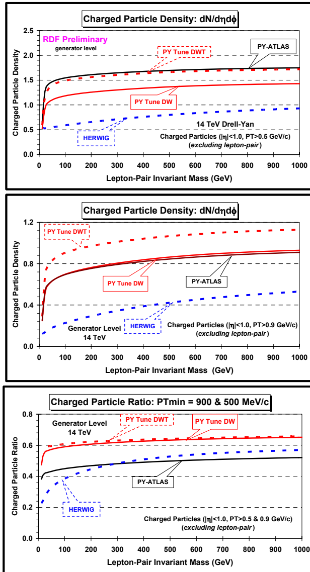
Fig. 13. Predictions at 14 TeV of PYTHIA Tune DW, Tune DWT, HERWIG, and the ATLAS Tune for the density of charged particles, dN/d\eta d\phi , with |\eta| < 1 and p_T > 0.5 \text{ GeV/c} (top) and p_T > 0.9 \text{ GeV/c} (middle) for Drell-Yan lepton-pair production (excluding the lepton-pair) as a function of the lepton-pair invariant mass. (bottom) The ratio of the charged particle density with p_T > 0.9 \text{ GeV/c} and p_T > 0.5 \text{ GeV/c} .
