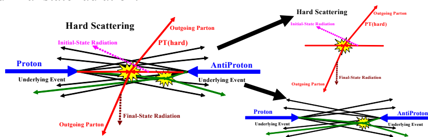
Fig. 1. Illustration of the way QCD Monte-Carlo models simulate a proton-antiproton collision in which a “hard” 2-to-2 parton scattering with transverse momentum, P_T(\text{hard}) , has occurred. The “hard scattering” component of the event consists of particles that result from the hadronization of the two outgoing partons ( i.e. the initial two “jets”) plus the particles that arise from initial and final state radiation ( i.e. multijets). The “underlying event” consists of particles that arise from the “beam-beam remnants” and from multiple parton interactions.
