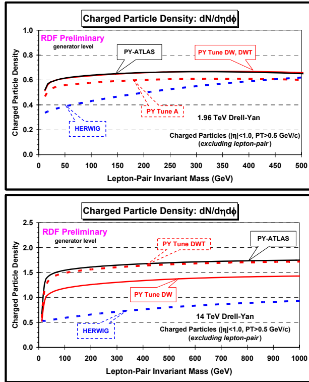
Fig. 10. Predictions of PYTHIA Tune A, Tune DW, Tune DWT, HERWIG, and the ATLAS PYTHIA Tune for the density of charged particles, dN/d\eta d\phi , with p_T > 0.5 GeV/c and |\eta| < 1 in Drell-Yan lepton-pair production (excluding the lepton-pair) at 1.96 TeV ( top ) and 14 TeV ( bottom ) as a function of the invariant mass of the lepton pair. Tune DW and Tune DWT are identical at 1.96 TeV.
