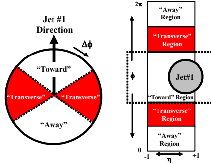
Fig. 2. Illustration of correlations in azimuthal angle \Delta\phi relative to the direction of the leading jet (MidPoint, R = 0.7 , f_{\text{merge}} = 0.75 ) in the event, jet#1. The angle \Delta\phi = \phi - \phi_{\text{jet}\#1} is the relative azimuthal angle between charged particles and the direction of jet#1. The “transverse” region is defined by 60^\circ < |\Delta\phi| < 120^\circ and |\eta| < 1 . The “transverse” region has an overall area in \eta - \phi space of \Delta\eta\Delta\phi = 4\pi/3 . We examine charged particles in the range p_T > 0.5 GeV/c and |\eta| < 1 , but allow the leading jet to be in the region |\eta(\text{jet}\#1)| < 2 .
