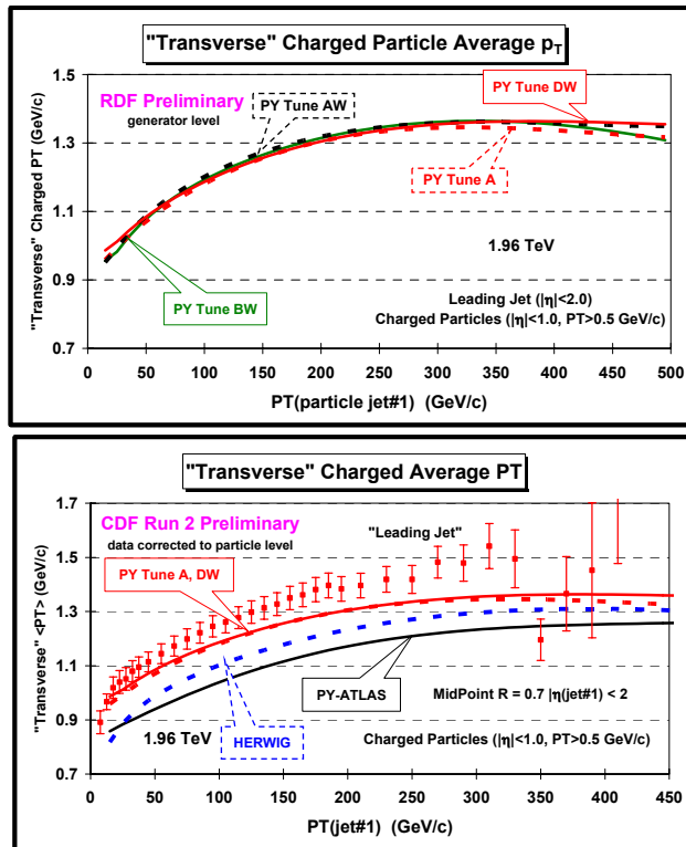
Fig. 9. ( top ) Predictions of PYTHIA Tune A, Tune AW, Tune BW, and Tune DW for average p_T of charged particles with p_T > 0.5 GeV/c and |\eta| < 1 in the “transverse” region for “leading jet” events at 1.96 TeV as a function of the leading jet P_T . ( bottom ) CDF Run 2 data at 1.96 TeV on the average p_T of charged particles with p_T
