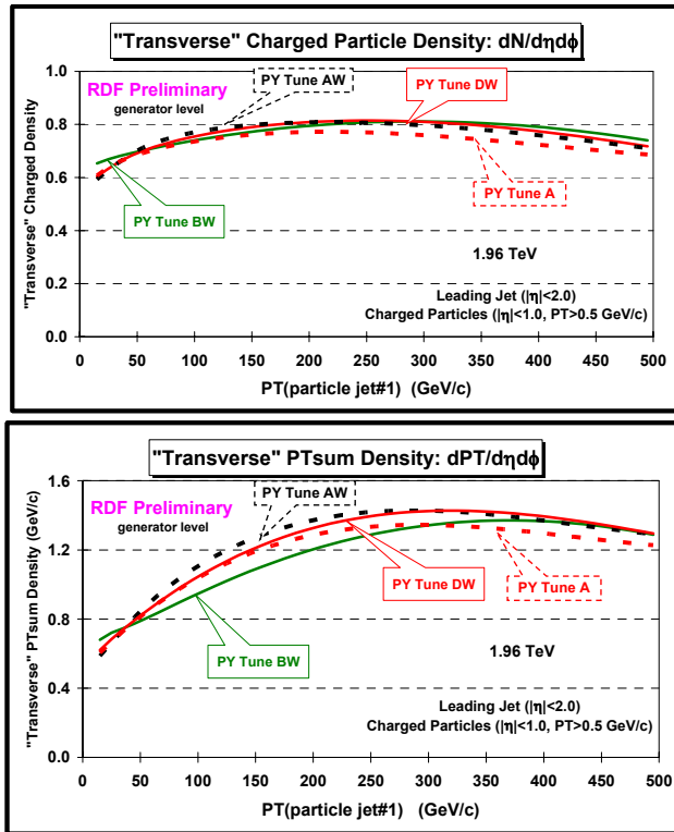
Fig. 6. Predictions at 1.96 TeV of PYTHIA Tune A, Tune AW, Tune BW, and Tune DW for the density of charged particles, dN/d\eta d\phi ( top ), and the charged PTsum density, dPT/d\eta d\phi ( bottom ), with p_T > 0.5 GeV/c and |\eta| < 1 in the “transverse” region for “leading jet” events as a function of the leading jet P_T .
