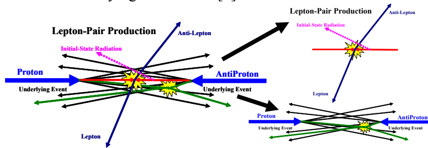
Fig. 4. Illustration of the way QCD Monte-Carlo models simulate Drell-Yan lepton-pair production. The “hard scattering” component of the event consists of the two outgoing leptons plus particles that result from initial-state radiation. The “underlying event” consists of particles that arise from the “beam-beam remnants” and from multiple parton interactions.
