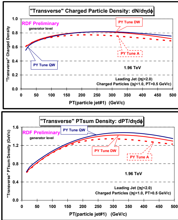
Fig. 8. Predictions at 1.96 TeV of PYTHIA Tune A, Tune DW, and Tune QW for the density of charged particles, dN/d\eta d\phi ( top ), and the charged PTsum density, dPT/d\eta d\phi ( bottom ), with p_T > 0.5 GeV/c and |\eta| < 1 in the “transverse” region for “leading jet” events as a function of the leading jet P_T .
