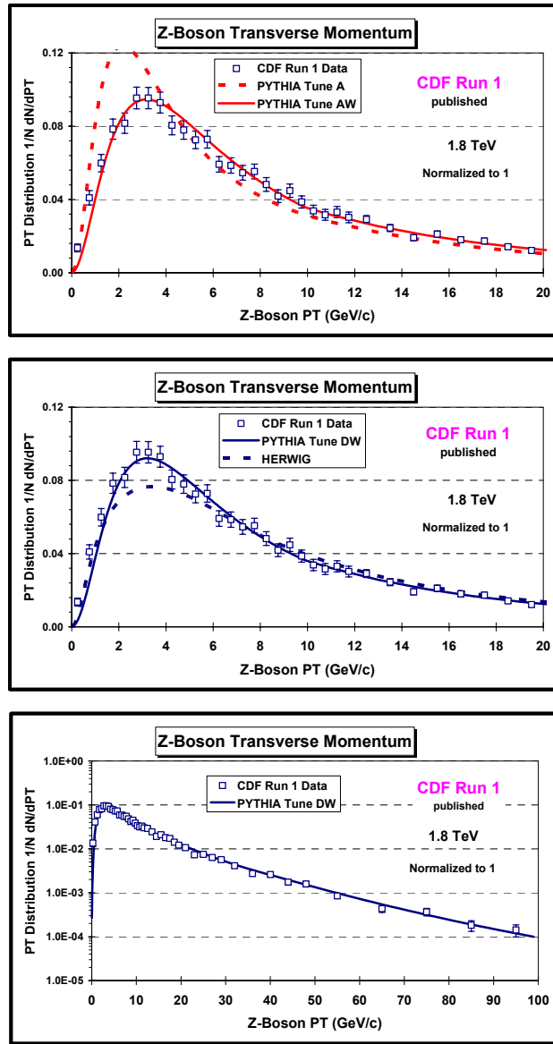
Fig. 5. CDF Run 1 data on the Z-boson p_T distribution compared with PYTHIA Tune A, Tune AW, Tune DW, and HERWIG.
