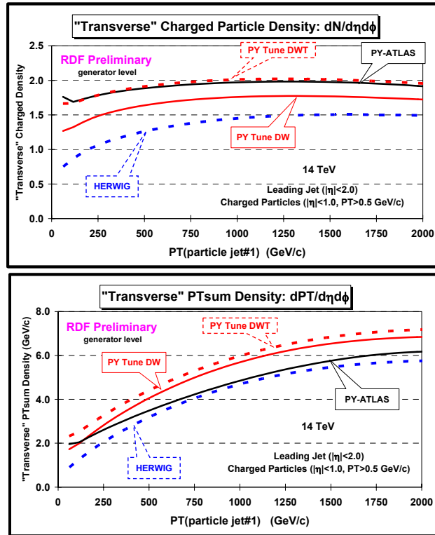
Fig. 11. Predictions at 14 TeV of PYTHIA Tune DW, Tune DWT, HERWIG, and the ATLAS Tune for the density of charged particles, dN/d\eta d\phi (top), and the charged PTsum density, dPT/d\eta d\phi (bottom), with p_T > 0.5 GeV/c and |\eta| < 1 in the “transverse” region for “leading jet” events as a function of the leading jet P_T .
