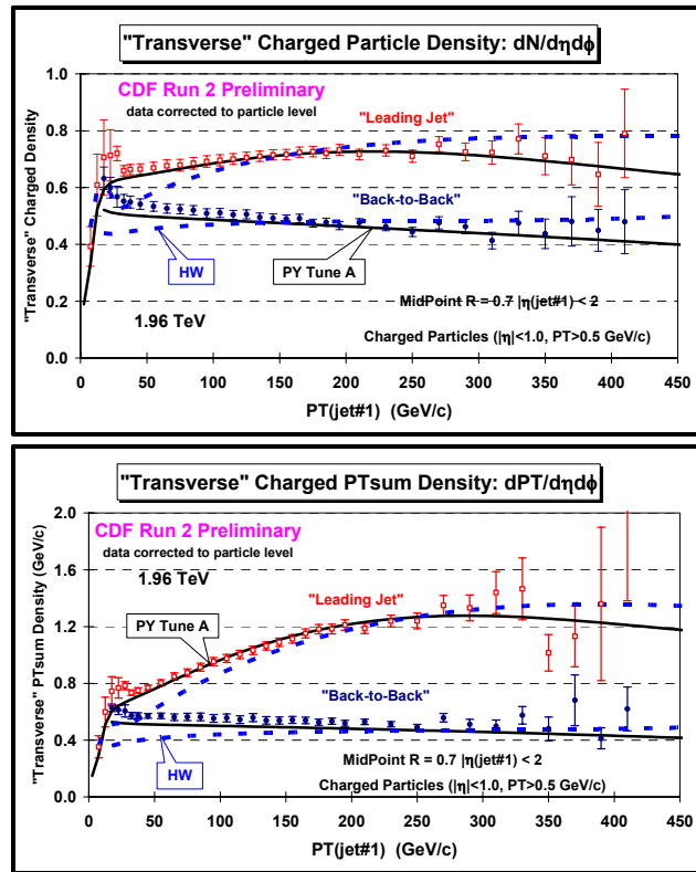
Fig. 3. CDF Run 2 data at 1.96 TeV on the density of charged particles, dN/d\eta d\phi (top), and the charged PTsum density, dPT/d\eta d\phi (bottom), with p_T > 0.5 GeV/c and |\eta| < 1 in the “transverse” region for “leading jet” and “back-to-back” events as a function of the leading jet P_T compared with PYTHIA Tune A and HERWIG. The data are corrected to the particle level (with errors that include both the statistical error and the systematic uncertainty) and compared with the theory at the particle level ( i.e. generator level).
