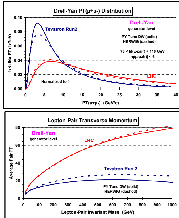
Fig. 12. Predictions at 1.96 TeV (Tevatron Run 2) and 14 TeV (LHC) of PYTHIA Tune DW and HERWIG for (top) the lepton-pair p_T distribution at the Z-boson mass and (bottom) the average lepton-pair p_T versus the lepton pair invariant mass.
