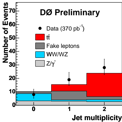
Figure 2: DØ t t cross section measurement in the dilepton channel. Observed and predicted number of events with 0, 1 and 2 or more jets.
