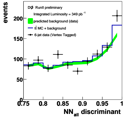
Figure 8: DØ all-hadronic analysis. Output of the NN. The last four bins include all the data that pass all the cuts included the D_{NN} > 0.9 cut. Shown is the tagged data (points), the prediction for the background (green band) and the background+ t\bar{t} to all-hadronic Monte Carlo added to it (blue histogram, a cross section of 6.5 pb is assumed).
