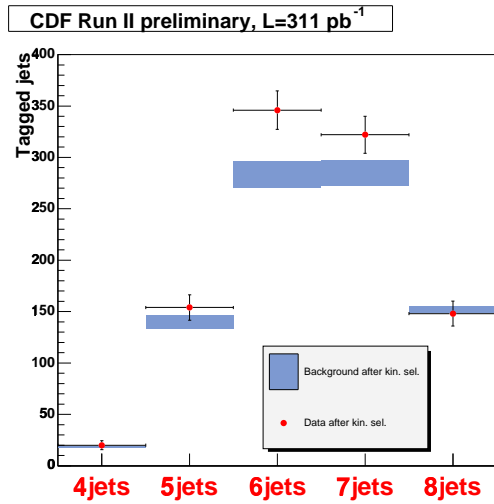
Figure 7: CDF all-hadronic analysis. Comparison between tags expected from background contributions and observed tags in each multiplicity bins.
