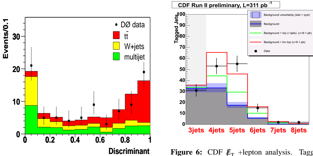
Figure 5: D\phi t\bar{t} cross section measurement in the \ell +jets channel. Likelihood discriminant distribution for data overlaid with the result of the fit of t\bar{t} , W +jets and multijet backgrounds.
