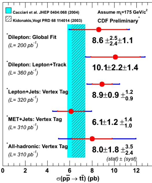
Figure 9: Summary of top pair production experimental results from CDF (left) and DØ (right) experiments. The bands represent the NLO theory calculation for a 175 GeV/c 2 top mass.
