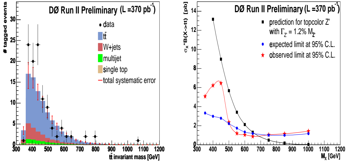
Figure 11: D0 resonant t\bar{t} search. Left: resulting mass distribution for the combined \ell+jets channels. The error bars on top of the Standard Model background indicate the total systematic uncertainty, which has significant bin-to-bin correlations. Right: Expected and observed 95% C.L. upper limits on \sigma_X \cdot Br(X \rightarrow t\bar{t}) compared with the predicted topcolor-assisted technicolor cross section for a Z' boson with a width of \Gamma_{Z'} = 0.012 M_{Z'} as a function of resonance mass M_X .
