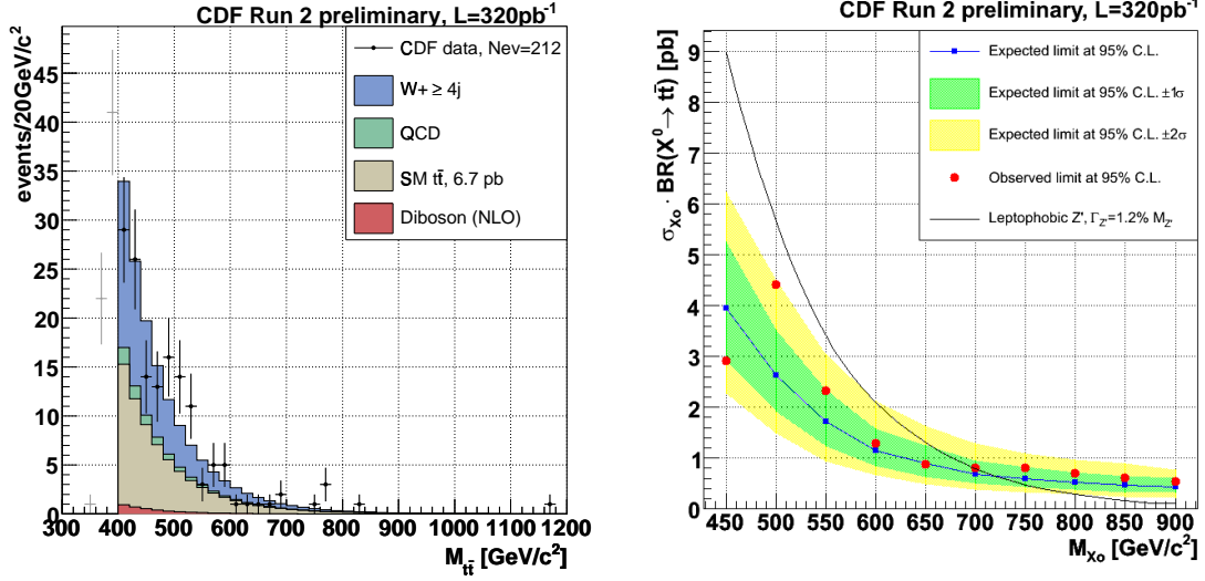
Figure 10: CDF resonant t\bar{t} search. Left: reconstructed M_{t\bar{t}} spectrum vs the standard model expectation in the search region above the 400 \text{ GeV}/c^2 cut. Grey points show data distribution below 400 \text{ GeV}/c^2 . Right: expected and experimental upper limits for a resonance in 320 \text{ pb}^{-1} of CDF data together with leptophobic topcolor Z' cross section prediction. Green and yellow areas define the central 68% and 95% frequentistic bands for the expected limits.
