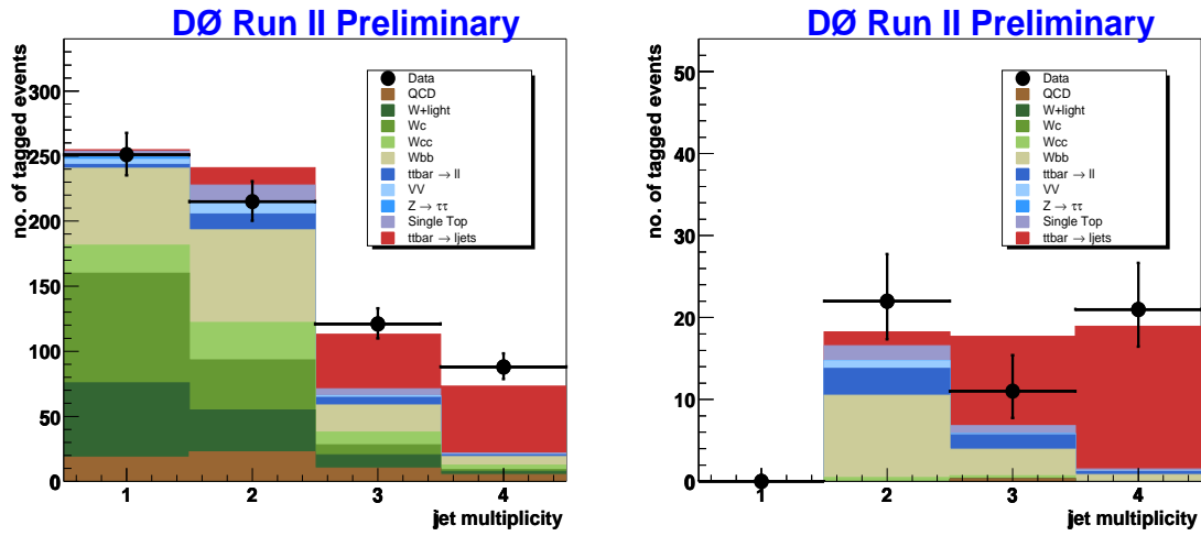
Figure 4: D\phi t\bar{t} cross section measurement using b -tagging in the lepton+jets channel. Predicted and observed tagged events in 365\text{pb}^{-1} of data: single tags (left) and double tags (right).
