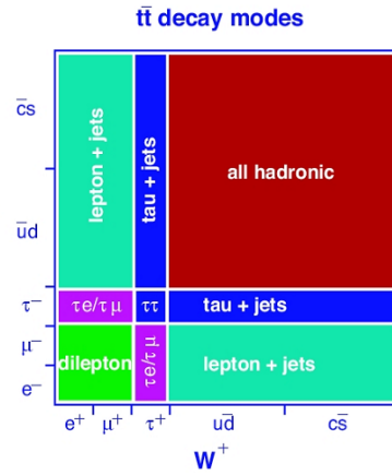
Figure 1: t\bar{t} decay channels.
