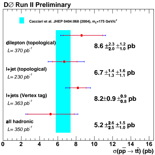
Figure 9: Summary of top pair production experimental results from CDF (left) and DØ (right) experiments. The bands represent the NLO theory calculation for a 175 GeV/c 2 top mass.
