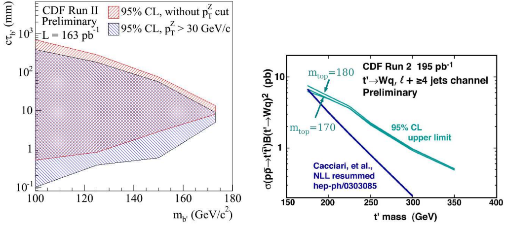
Figure 2: Results of 4th generation quark searches. Excluded region in decay length versus b' mass (left) and cross section times branching ratio as a function of t' mass (right).
