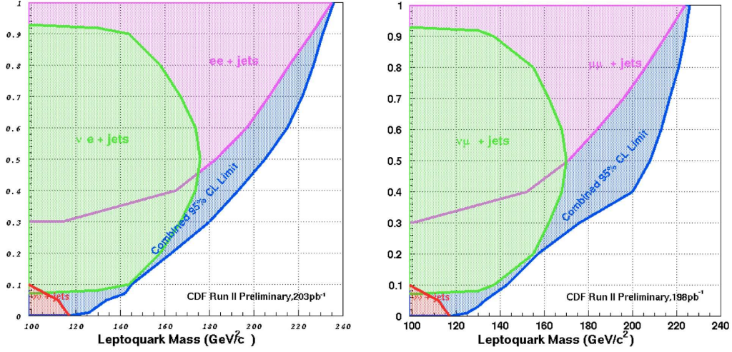
Figure 1: Combined mass limits as functions of \beta for LQ1 (left) and LQ2 (right).
