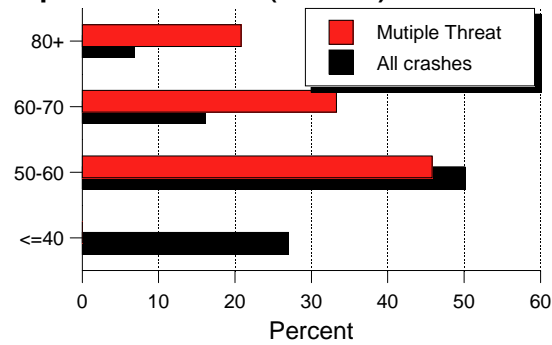
Figure 55. Light condition, number of lanes, and speed limit in “Multiple Threat.”
