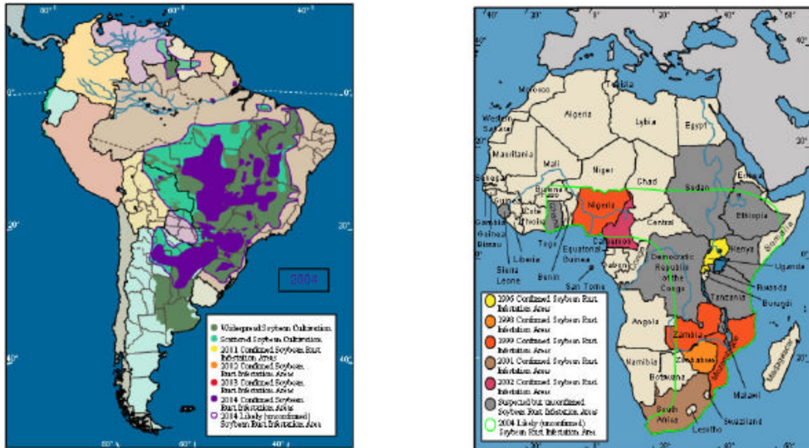
Figure 1. Soybean rust source area maps for South America and Africa. Maps can be accessed on the project's web site at http://soybeanrust.zedxinc.com/ . Detailed description of the information sources used to compile the maps is provided. The South American source area map is animated.
