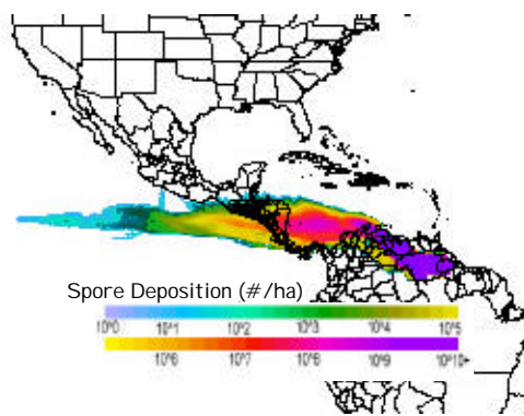
Figure 11. Cumulative wet deposition of P. pachyrhizi spores from northern South America soybean-growing region for a hypothetical 10 July 2003 release
