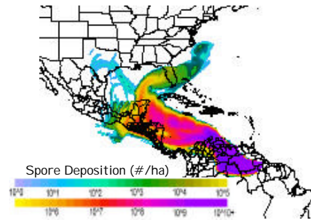
Figure 14. Cumulative wet deposition of P. pachyrhizi spores from northern South America soybean-growing region for a hypothetical 22-29 August 2003 release.
