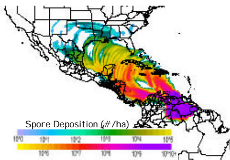
Figure 13. Cumulative wet deposition of P. pachyrhizi spores from northern South America soybean-growing region for a hypothetical 21-27 August 1999 release.
