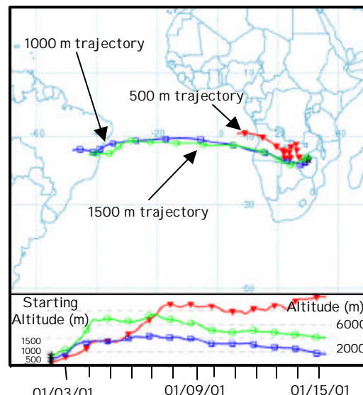
Figure 3. Forward trajectories from Zimbabwe on 2 January 2001. The trajectories begin at heights of 500 m (red triangles), 1000 m (blue squares), and 1500 m (green circles).
