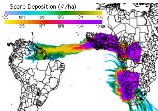
Figure 8. Cumulative wet deposition of P. pachyrhizi spores from African soybean-growing region for a hypothetical December 1999 release.
