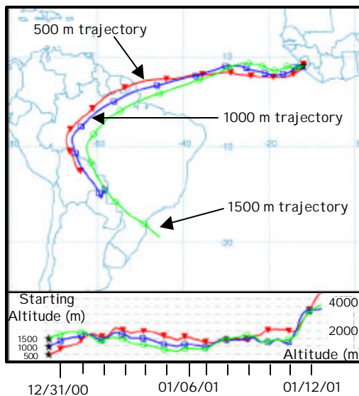
Figure 2. Forward trajectories from Sierra Leone on 30 December 2000. The trajectories begin at heights of 500 m (red triangles), 1000 m (blue squares), and 1500 m (green circles).
