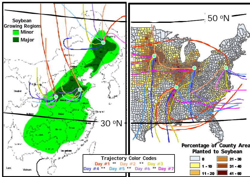
Figure 6. Backward trajectories initialized at a 500 m altitude for soybean growing regions in China and U.S. for individual days during the 4 th week of May 2002. The winds in the China soybean growing region were generally from the northwest while southerly airflow was present on many of the days in the U.S. soybean growing region.
