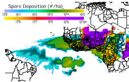
Figure 10. Cumulative wet deposition of P. pachyrhizi spores from Nigerian soybean-growing region for a hypothetical 07-22 July 2003 release.
