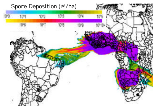
Figure 9. Cumulative wet deposition of P. pachyrhizi spores from African soybean-growing region for a hypothetical January 2000 release.
