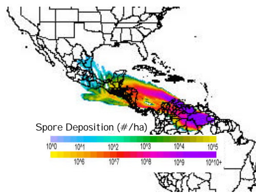
Figure 12. Cumulative wet deposition of P. pachyrhizi spores from northern South America soybean-growing region for a hypothetical 19 August 2001 release
