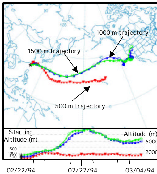
Figure 5. Forward trajectories from Taiwan on 22 Feb 1994. The trajectories begin at heights of 500 m (red triangles), 1000 m (blue squares), and 1500 m (green circles).
