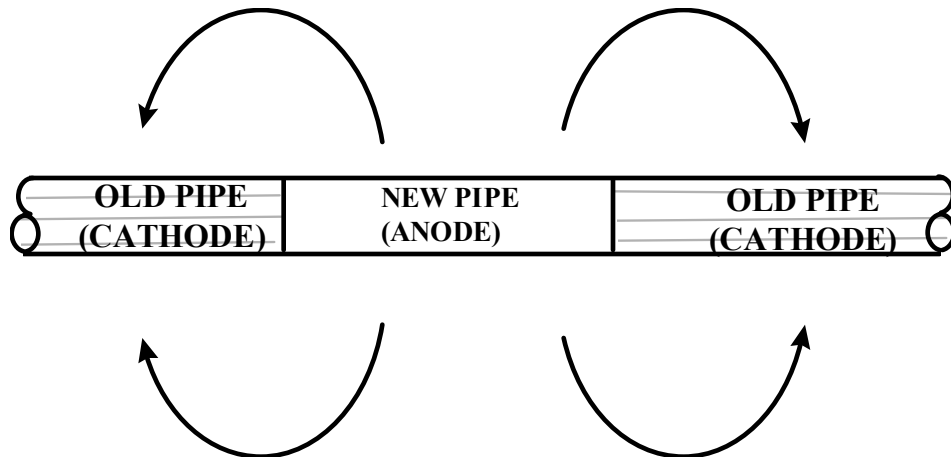
FIGURE III-19 GALVANIC CORROSION
