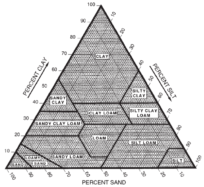
Figure 21.—Percentages of clay, silt, and sand in the basic USDA texture classes.
