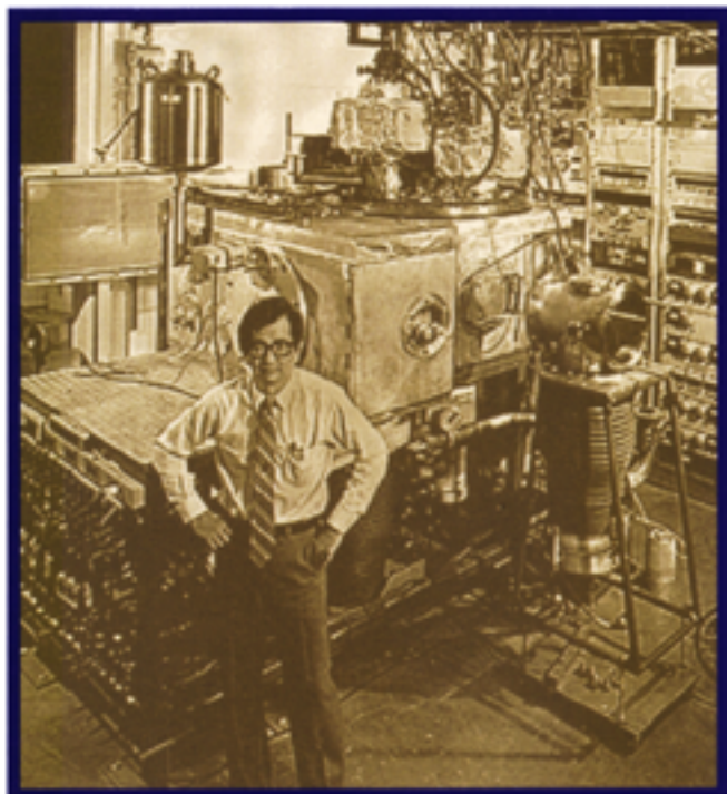
Nobel Laureate Y. T. Lee's crossed molecular beam experiments revolutionized the fundamental understanding of chemical reactions.
