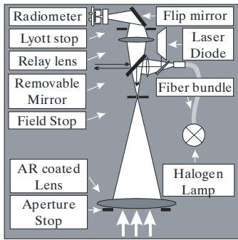
Figure 7. Principal components of the pyrometer
