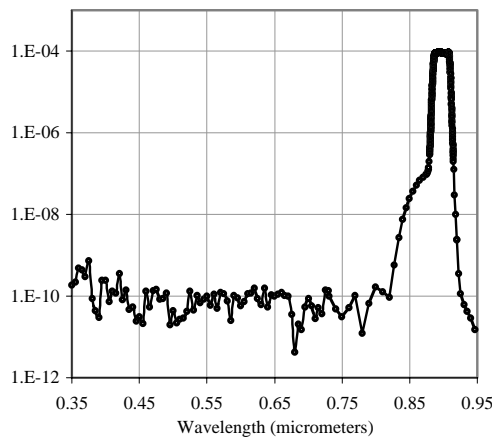
Figure 13. Typical pyrometer absolute responsivity curve, measured using relative responsivity and fixed point calibrations
