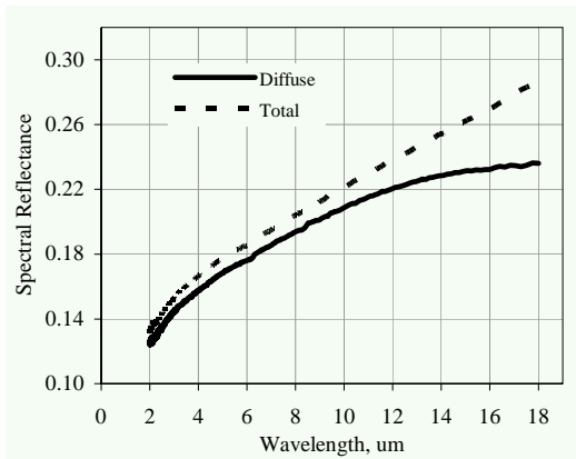
Figure 3. Flat graphite sample spectral directional-hemispherical reflectance and its diffuse component measured for incidence angle of 8°.
