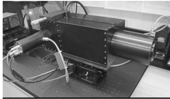
Figure 8. Picture of the assembled transfer standard pyrometer
