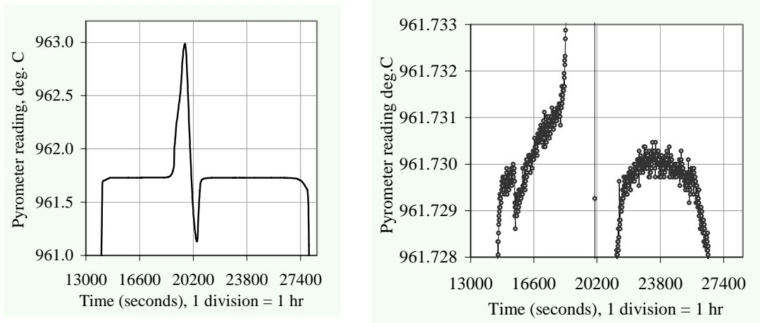
Figure 12. Transfer pyrometer readings during silver freezing and melting plateau after calibration using aluminum fixed point results. The standard deviation of the temperature reading during the freeze is 0.1 mK
