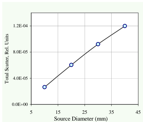
Figure 11. Total out of field scatter (SSE) performance of the NIST transfer standard pyrometer
