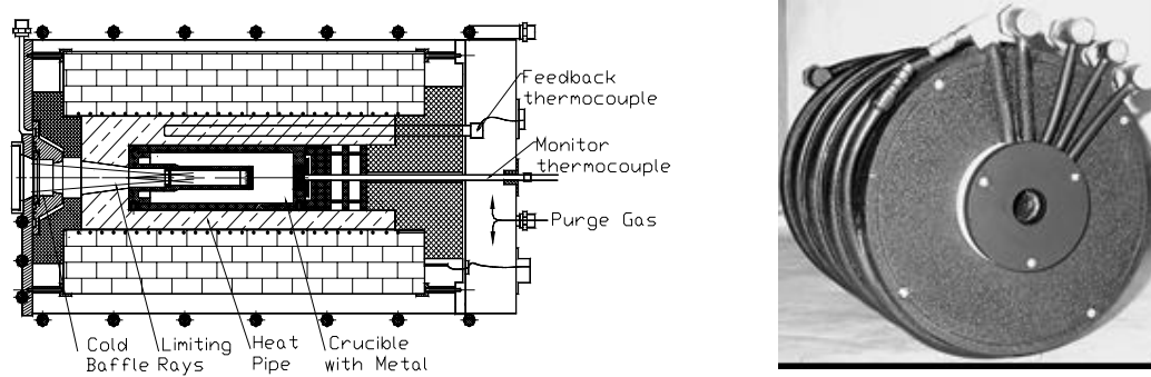
Figure 1. Design of the fixed point blackbody
