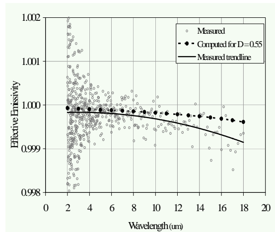
Figure 6. Measured and computed spectral effective emissivity of a cavity with V-grooved bottom
