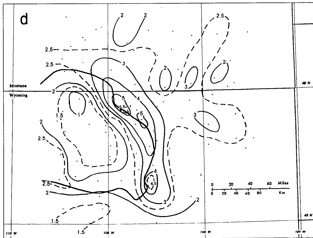
Figure 4. Average seasonal precipitation (inches) over the Big Horn mountains: c) summer, and d) fall.
