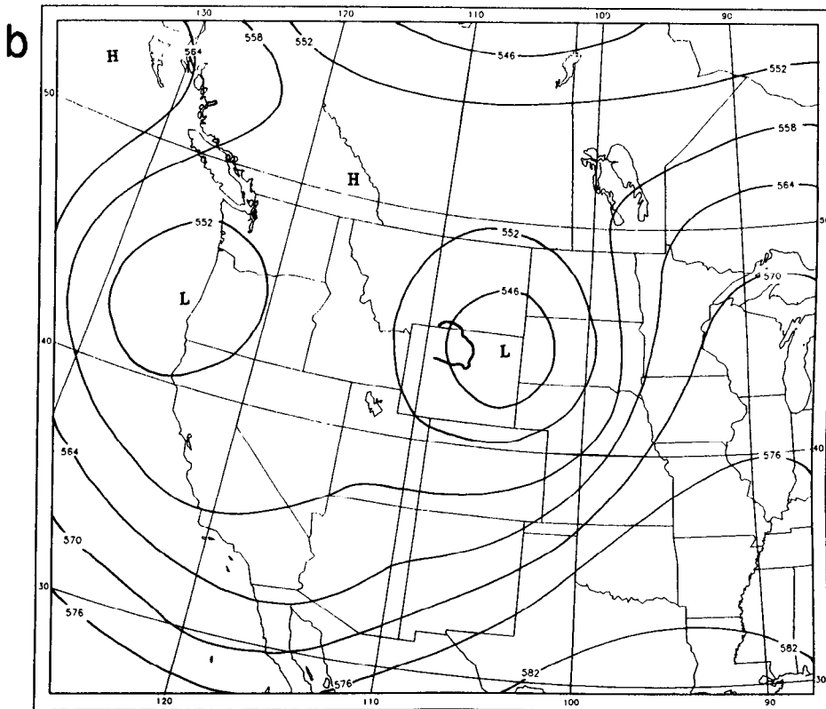
Figure 26. Type 6: a) typical surface and b) 500-mb maps (12Z May 7, 1988).
