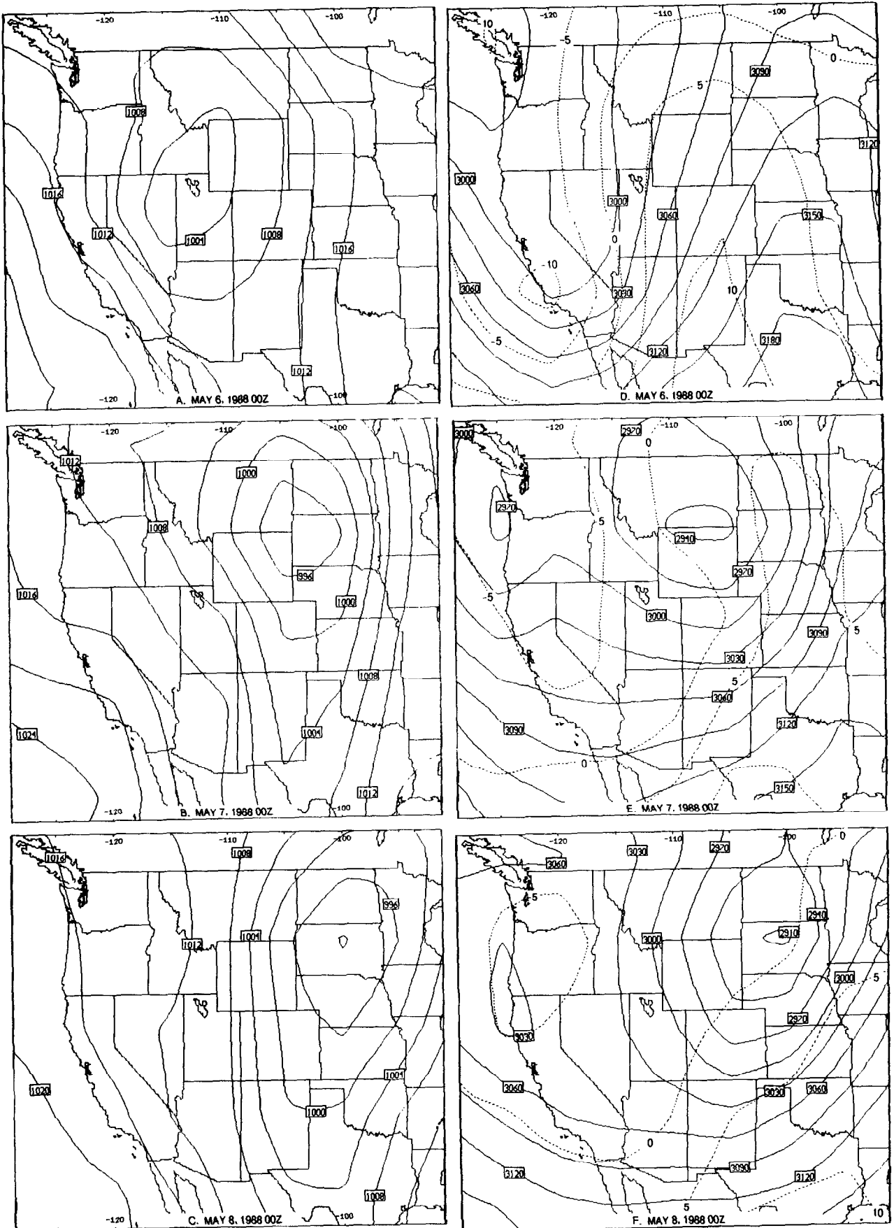
Figure 9. Surface (a-c) and 700-mb (d-f) maps for OOZ from May 6 through 8, 1988.
