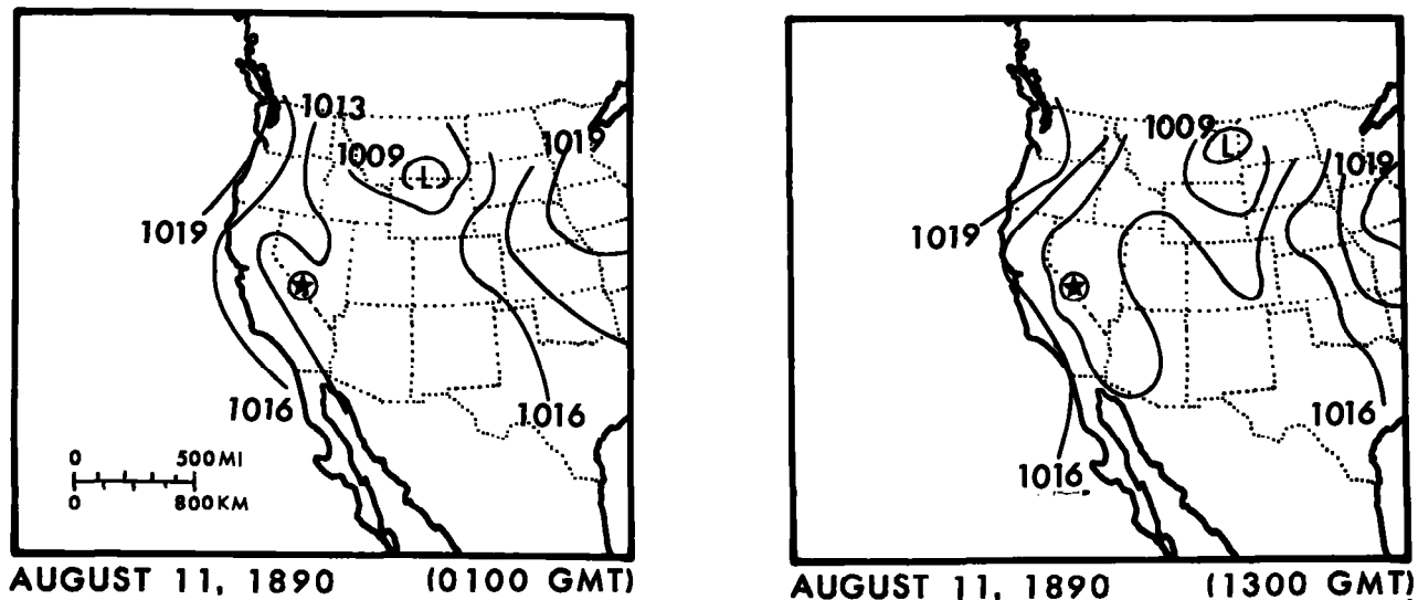
Figure 3.19.--Surface weather maps for August 11, 1890.
