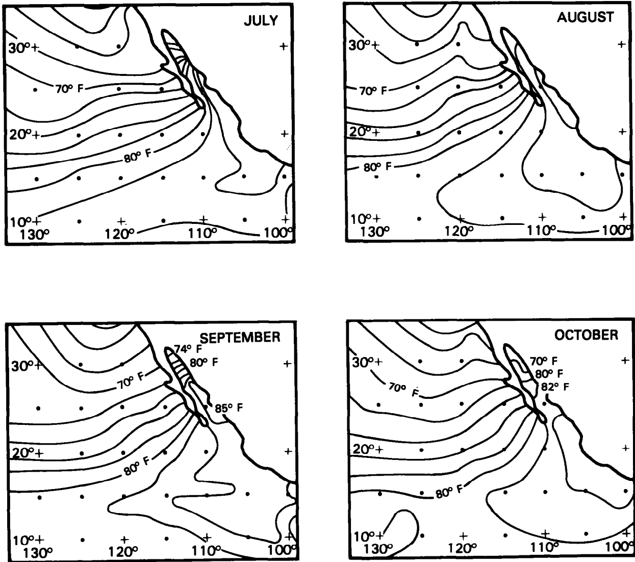
Figure 2.45.--Mean sea-surface temperature charts for the tropical Pacific for July, August, September and October (Laviolette and Seim 1969).
