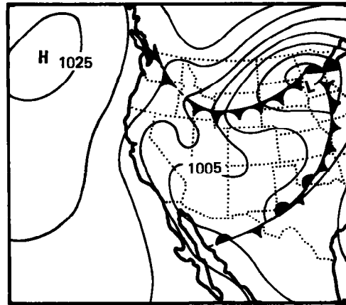
June 3, 1943 (1230 GMT)
