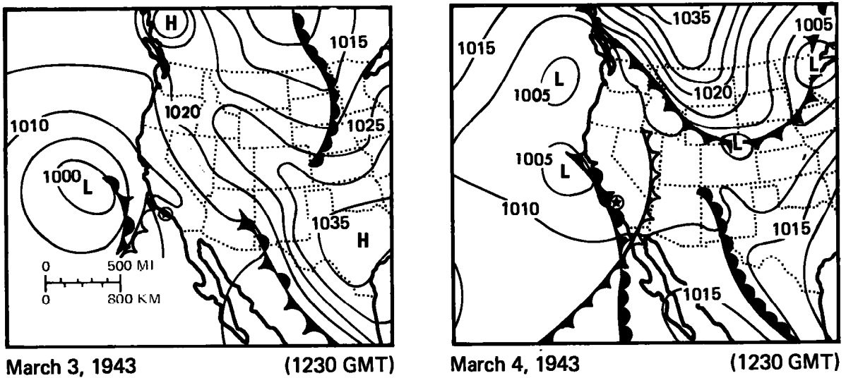
Figure 3.40.--Surface weather maps for March 3-4, 1934.
