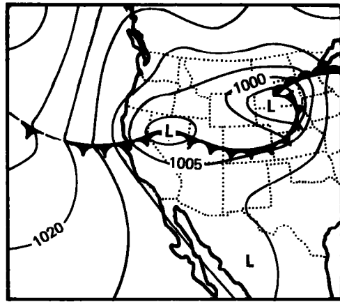
November 13, 1930 (1300 GMT)
