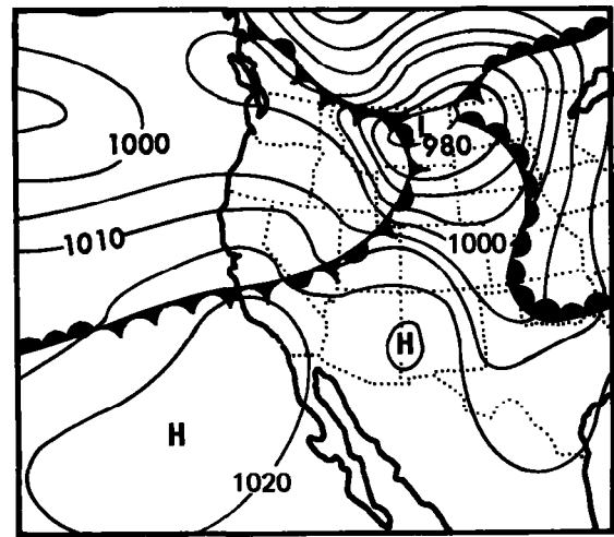
February 1, 1963 (1200 GMT)
