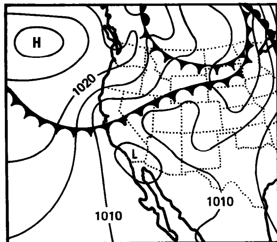
September 6, 1939 (1230 GMT)
