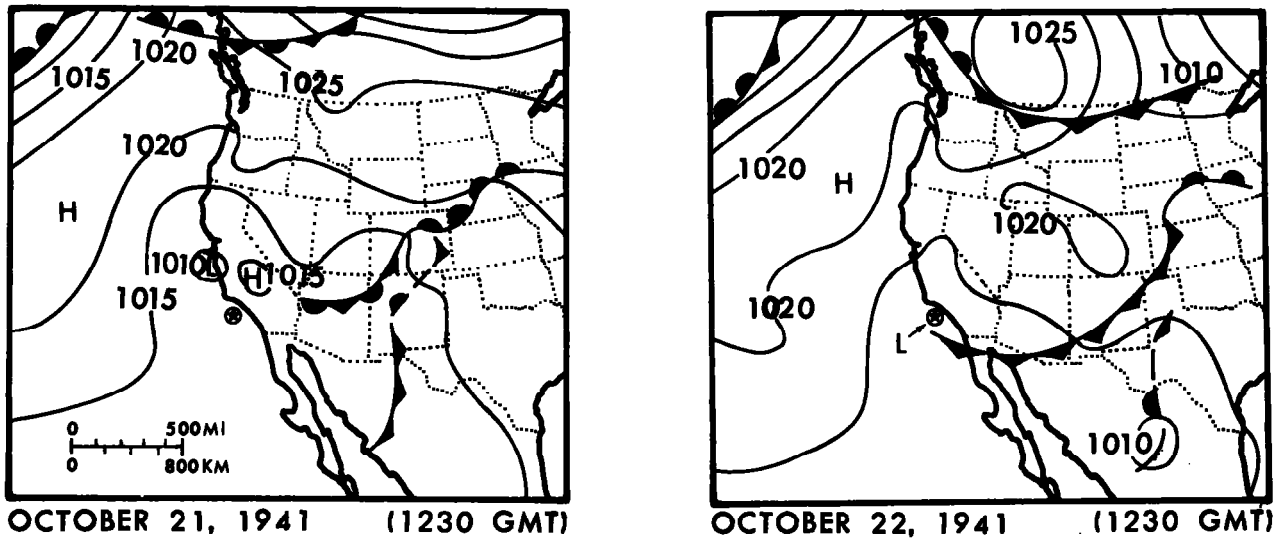
Figure 3.37.--Surface weather maps for October 20-23, 1941.
