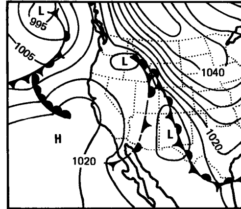
February 3, 1907 (1300 GMT)
