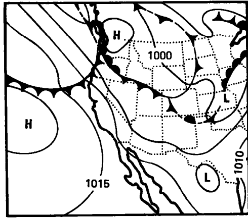
June 1, 1943 (1230 GMT)
