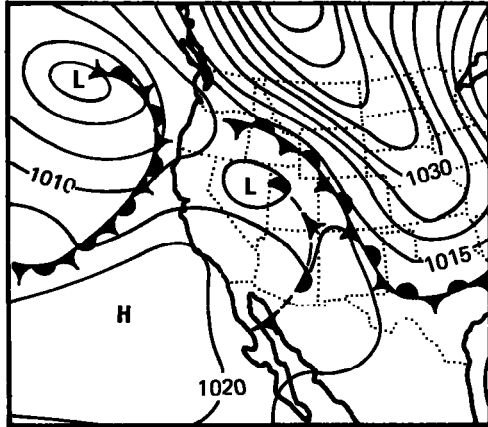
February 2, 1907 (1300 GMT)
