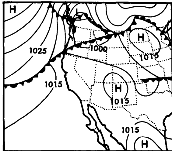
November 26, 1905 (1300 GMT)
