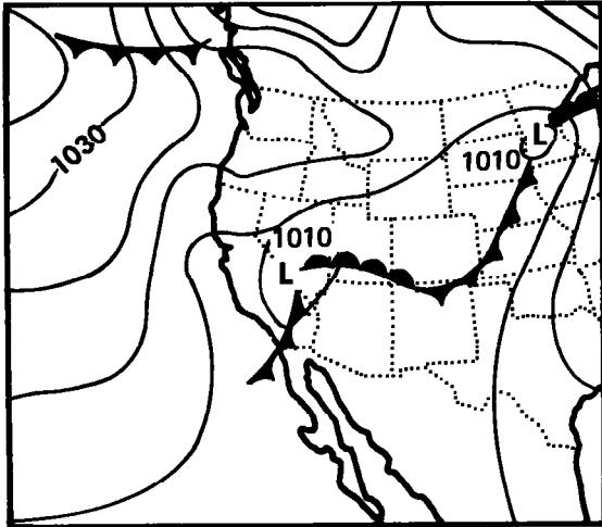
October 28, 1946 (1230 GMT)
