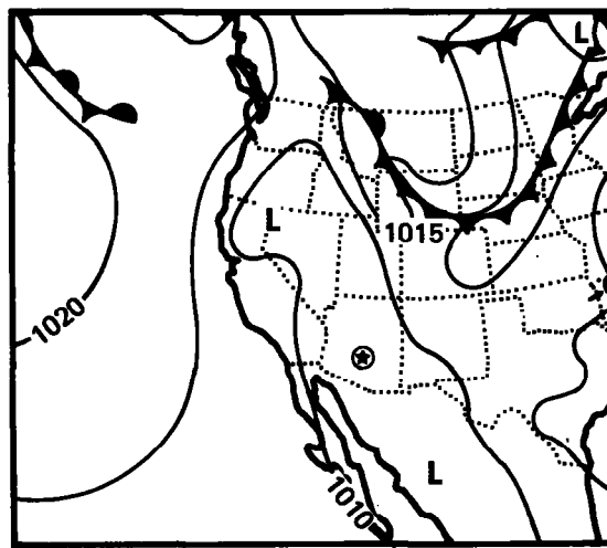
August 2, 1951 (1230 GMT)
