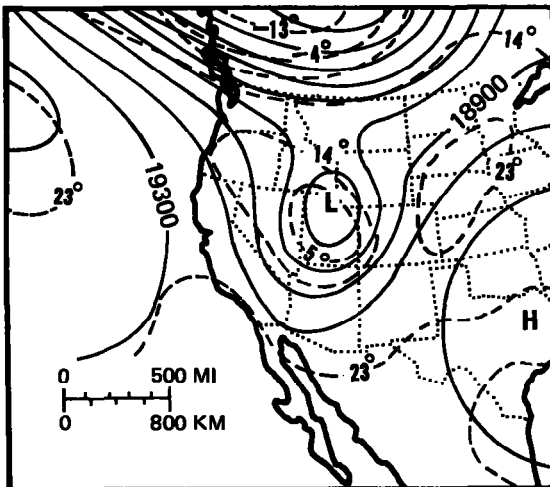
September 6, 1970 (1200 GMT)
