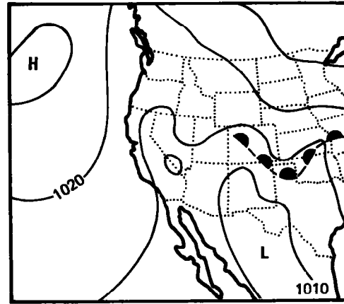
June 5, 1943 (1230 GMT)
