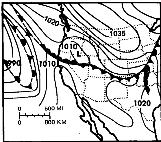
January 29, 1963 (1200 GMT)
