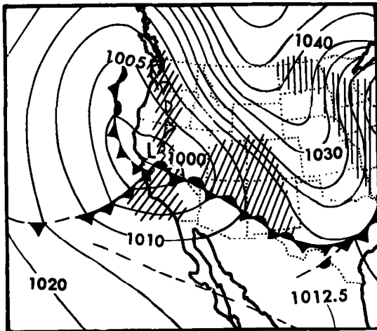
January 27, 1916 (1300 GMT)
