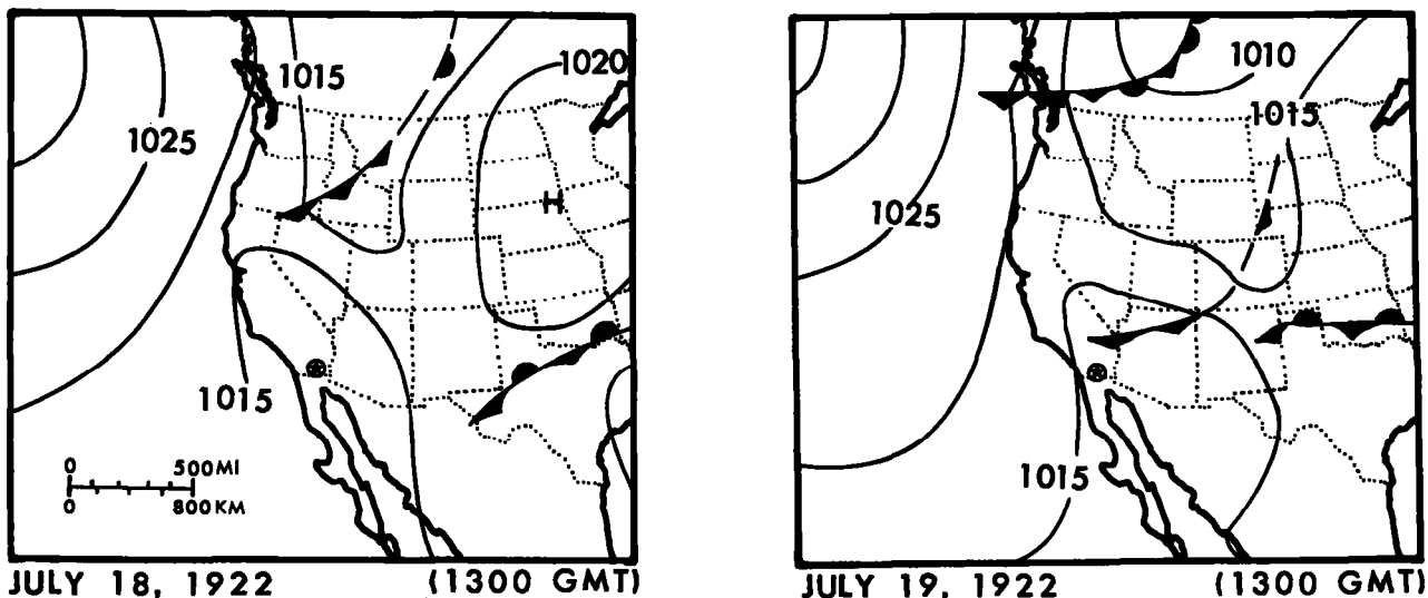
Figure 3.10.--Surface weather maps for July 18-19, 1922.
