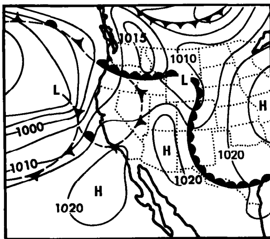
January 31, 1963 (1200 GMT)
