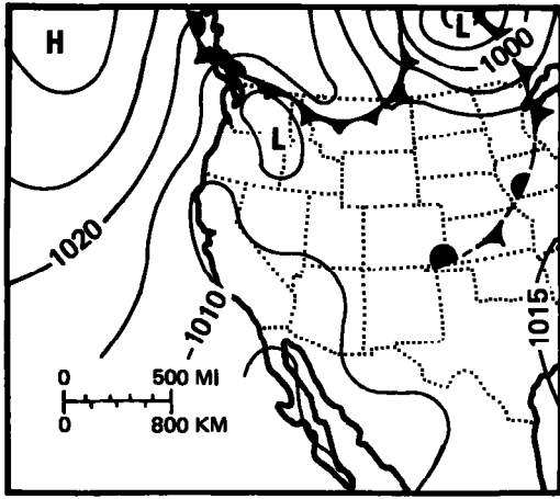
August 26, 1951 (1230 GMT)
