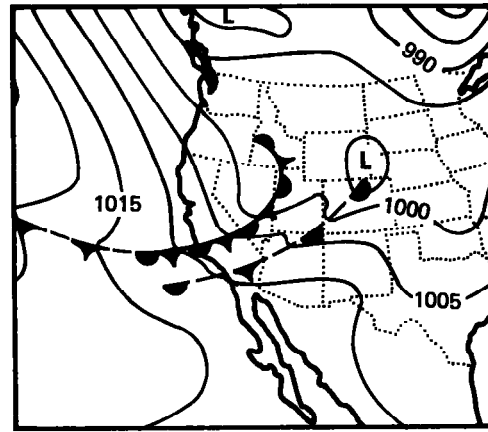
November 17, 1930 (1300 GMT)
