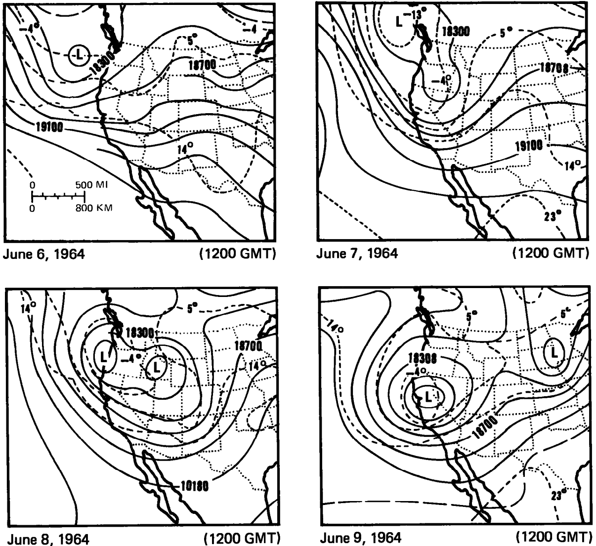
Figure 2.44.--500-mb charts for June 6-9, 1964.
