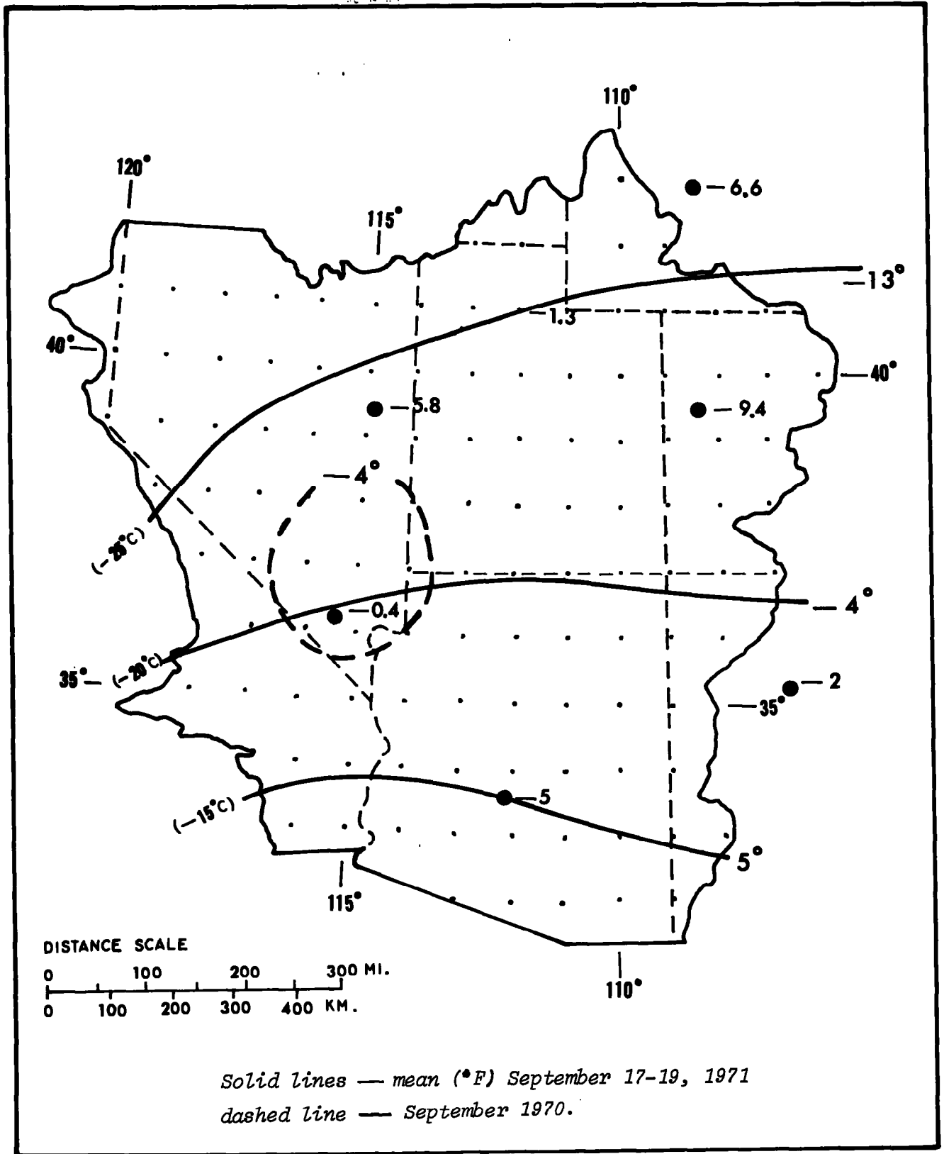
Figure 2.8.--Record 500-mb low temperatures for September.
