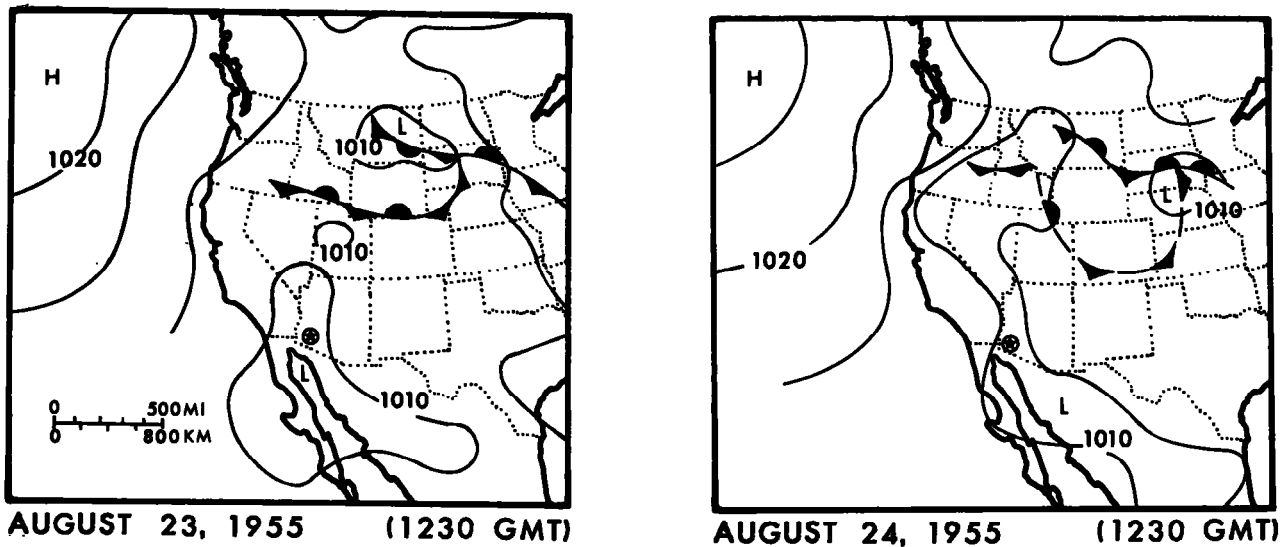
Figure 3.4.--Surface weather maps for August 23 and 24, 1955.
