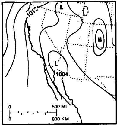
September 2, 1970 (1200 GMT)
