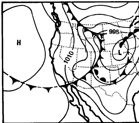
June 2, 1943 (1230 GMT)
