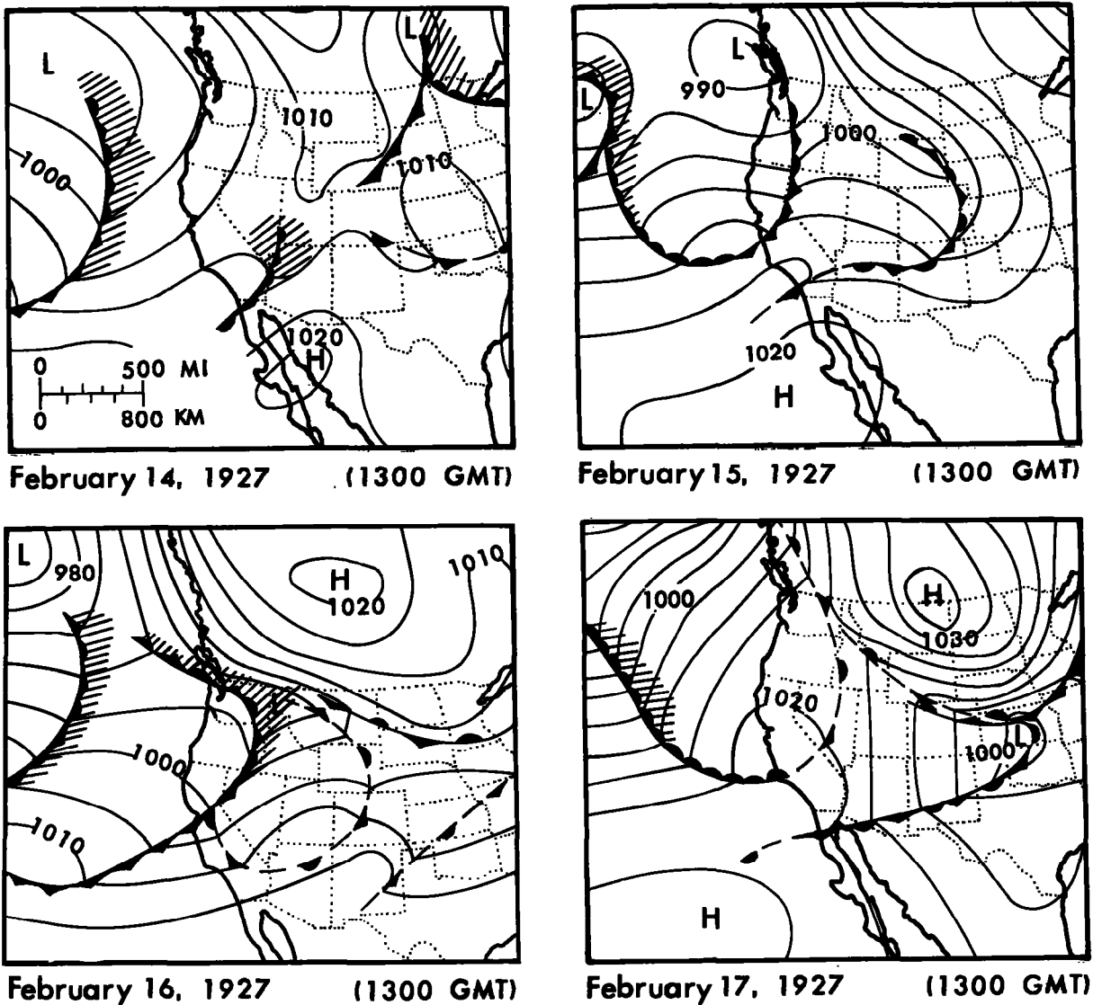
Figure 2.40.--Surface weather maps for February 14-17, 1927.
