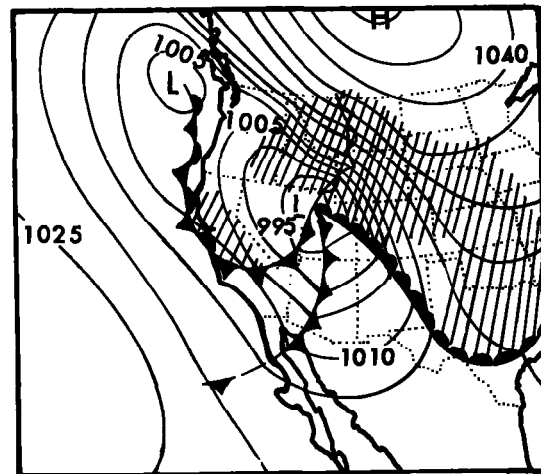
January 28, 1916 (1300 GMT)
