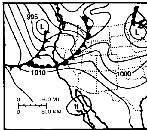
November 16, 1930 (1300 GMT)
