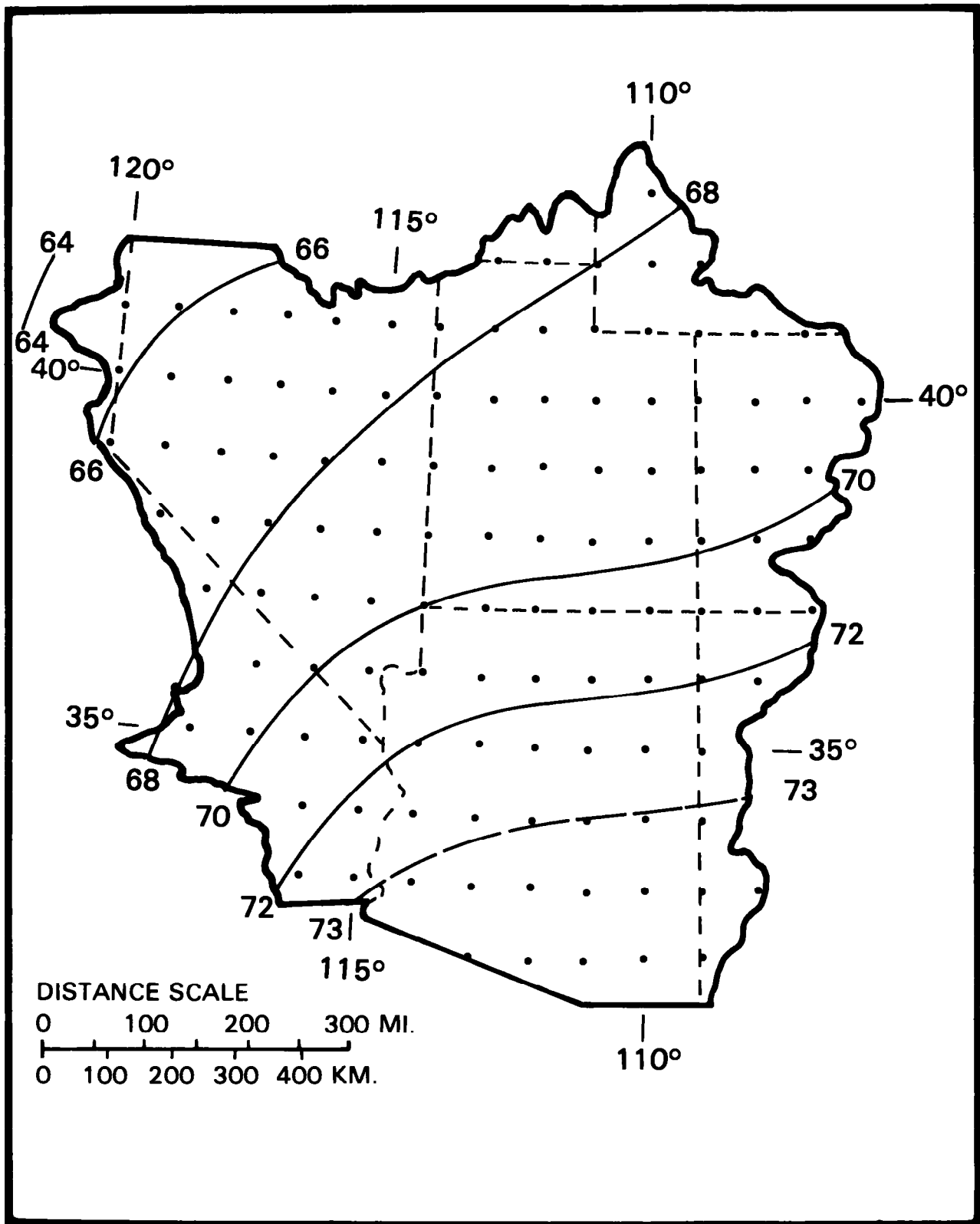
Figure 4.27.--1000-mb 12-hr persisting general storm dew point for mid-September.
