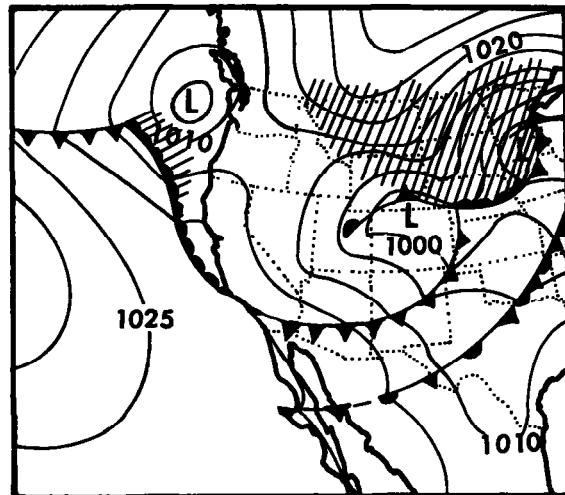
November 28, 1905 (1300 GMT)
