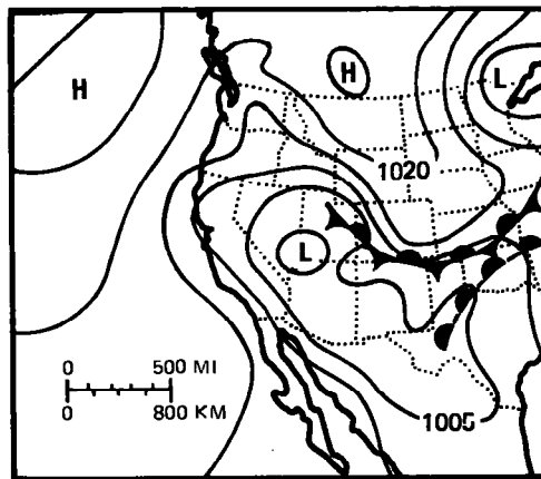
June 4, 1943 (1230 GMT)
