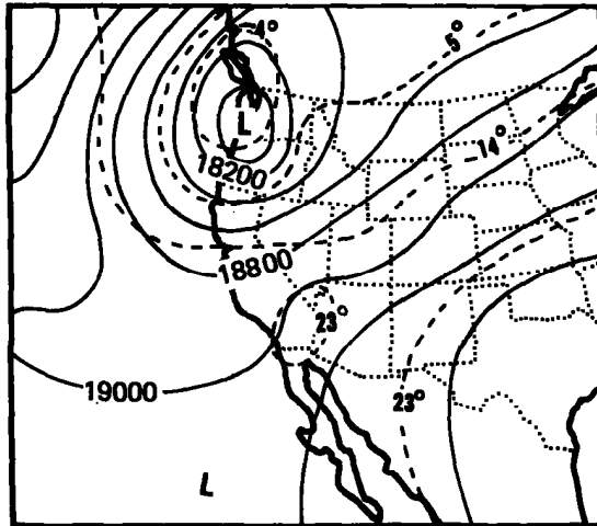
August 28, 1951 (1500 GMT)
