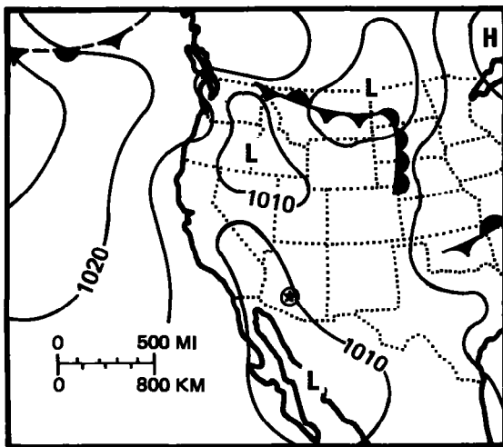
August 1, 1951 (1230 GMT)
