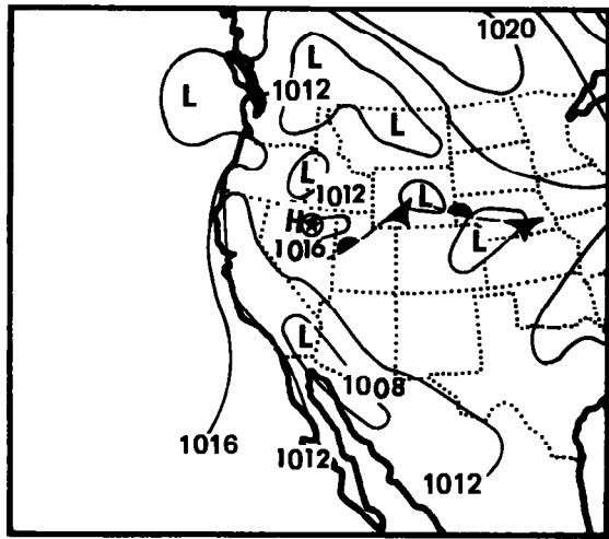
August 28, 1970 (1200 GMT)
