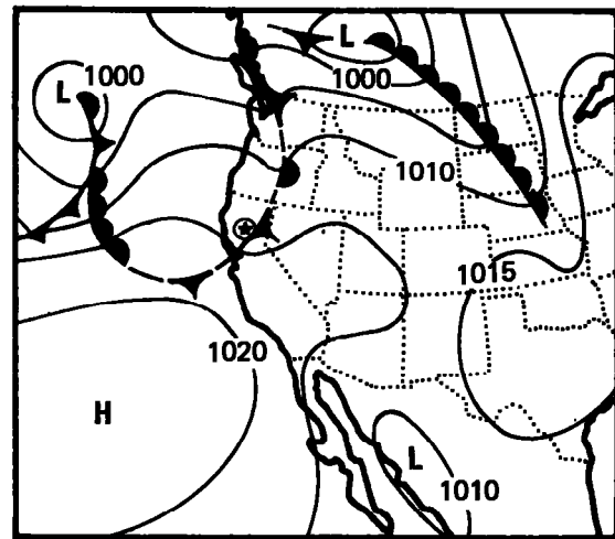
May 10, 1915 (1300 GMT)
