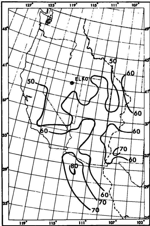
AUGUST 25, 1970 (1000 GMT)
