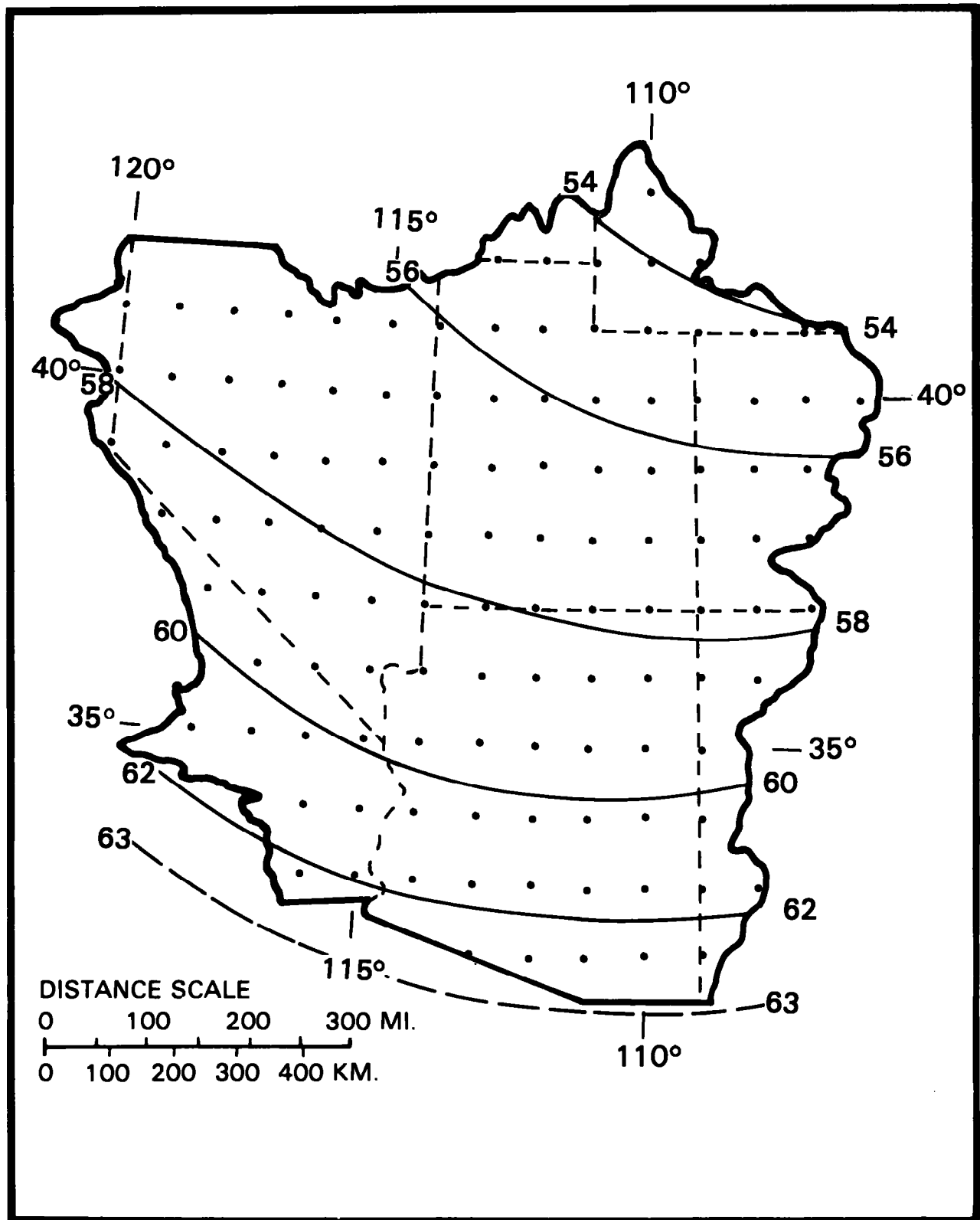
Figure 4.14.--1000-mb 12-hr persisting dew point for mid-February.
