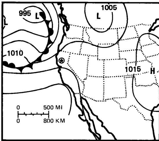
May 9, 1915 (1300 GMT)
