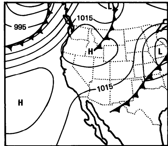
October 6, 1911 (1300 GMT)
