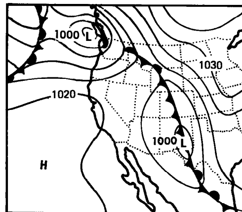
February 5, 1907 (1300 GMT)
