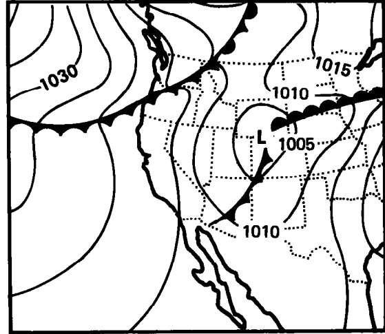
October 29, 1946 (1230 GMT)
