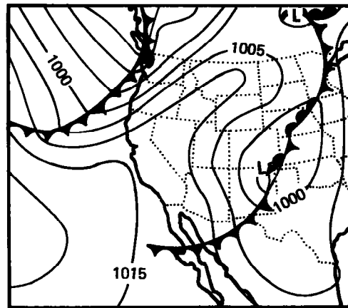
November 15, 1930 (1300 GMT)
