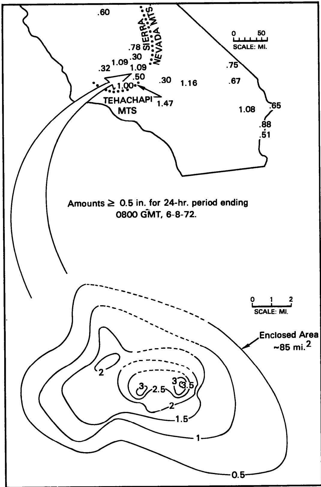
Figure 3.15.--Isohyetal analysis for storm of June 7, 1972.
