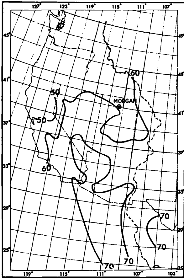
AUGUST 13, 1958 (1200 GMT)
