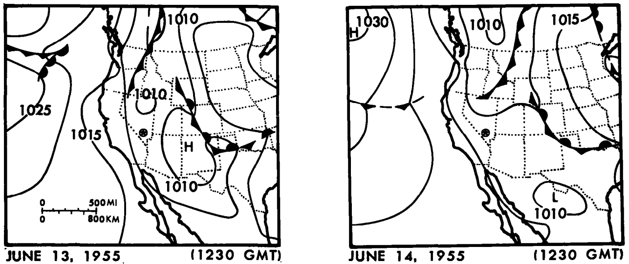
Figure 3.21. Surface weather maps for June 13-14, 1955.
