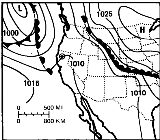
September 17, 1959 (1230 GMT)
