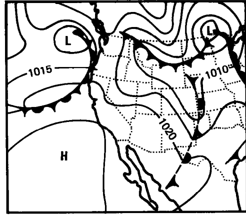
February 1, 1907 (1300 GMT)
