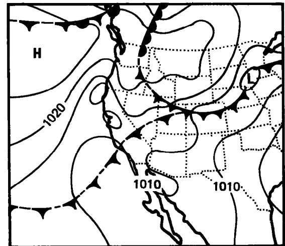
September 7, 1939 (1230 GMT)
