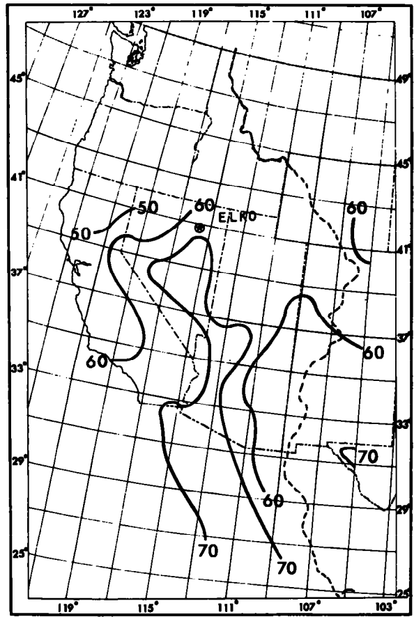
AUGUST 27, 1970 (2100 GMT)
