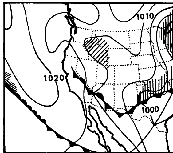
February 8, 1937 (1300 GMT)
