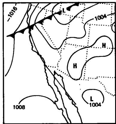
September 4, 1970 (1200 GMT)
