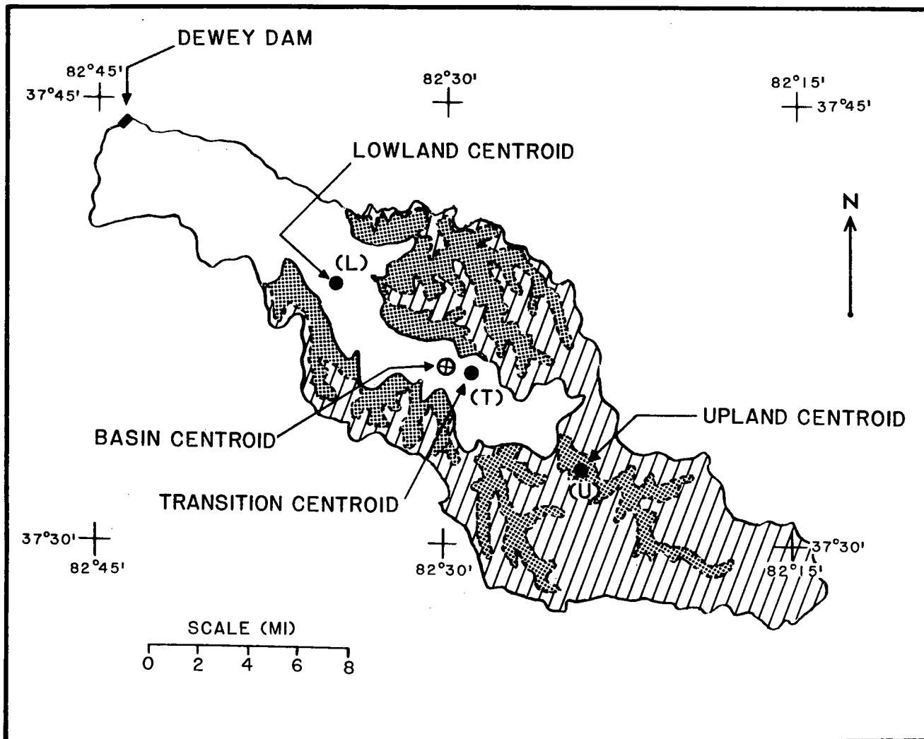
Figure 3-4.--Topographic subdivisions for DDKY with locations of centroids (filled circles) for each subdivision and for the drainage as a whole (open circle). Lowlands are unshaded; uplands are hatched; and transition areas are stippled.
