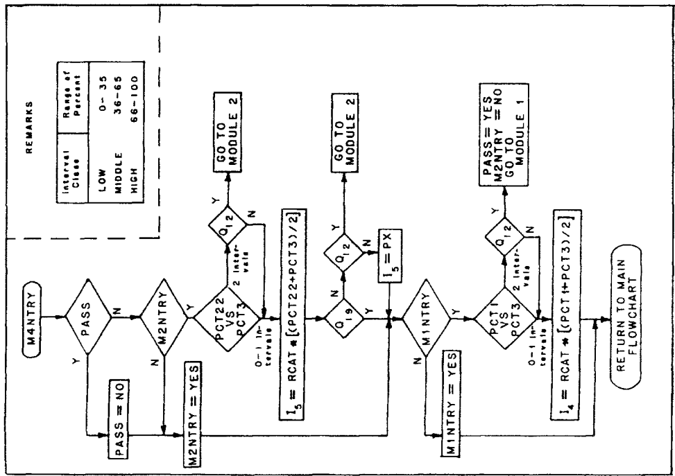
Figure 7.7.—Flowchart for module 4, SSH.
