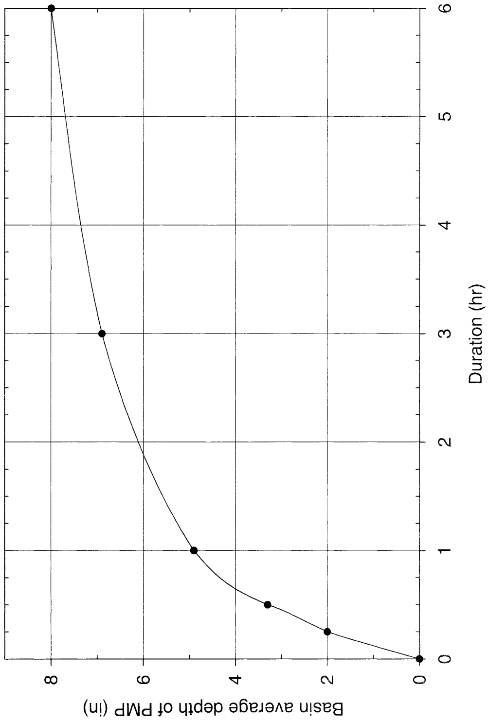
Figure 13.30. Average depth of local-storm PMP for the 167-mi 2 McCoy Wash, California.
