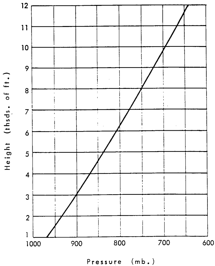
Figure 15.33.--Pressure-height relation (HMR 43).
