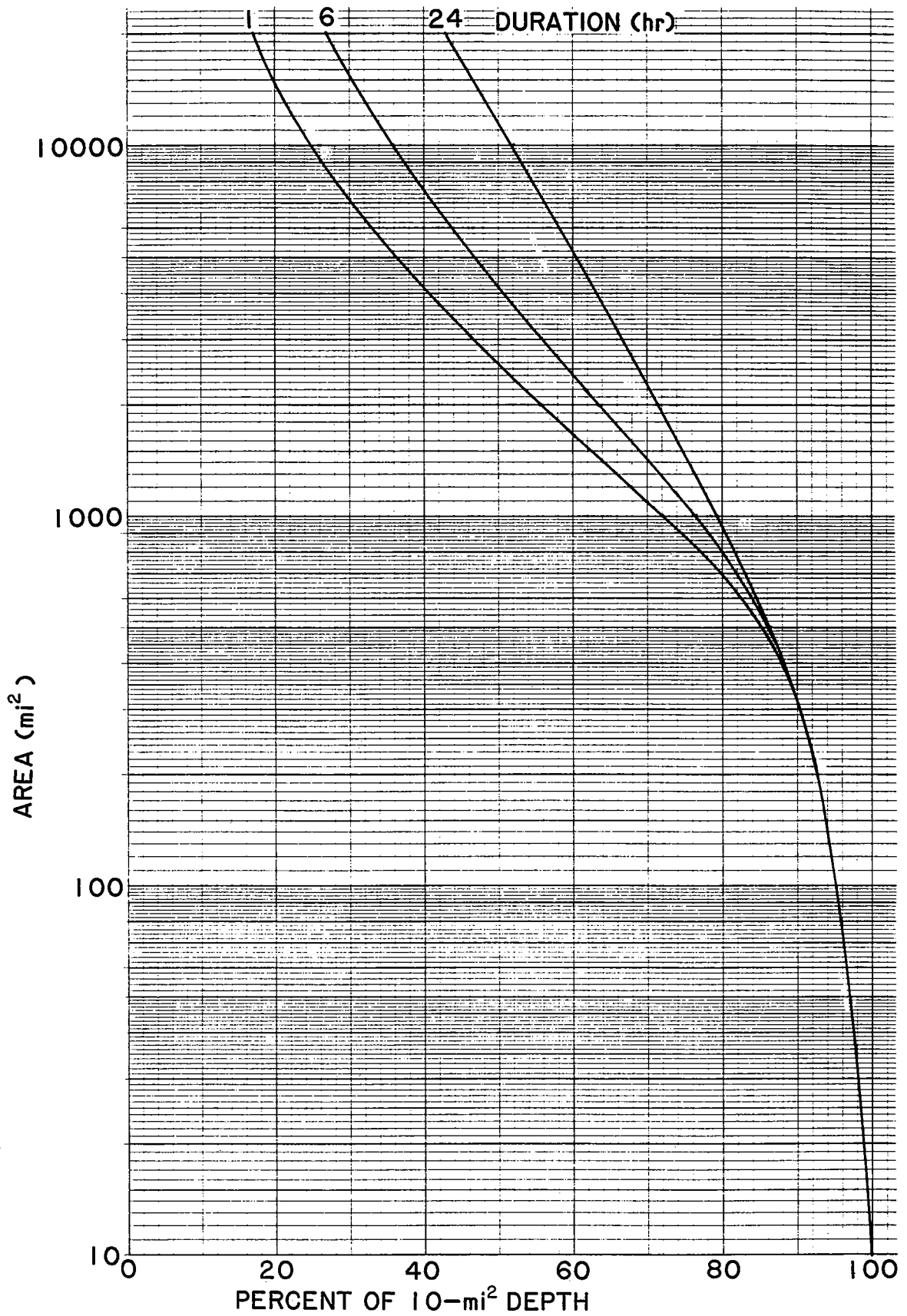
Figure 10.3.--Depth-area relations based on average of two storms (106 and 143). Not adopted for least orographic subregions in this study.
