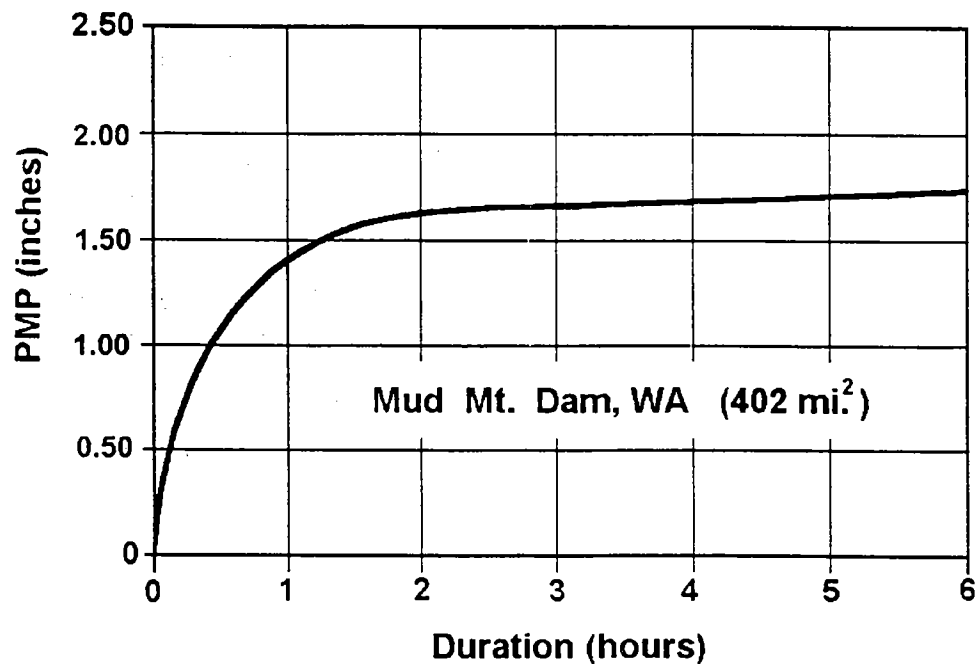
Figure 15.41.--Temporal distribution relation for Mud Mountain Dam.
