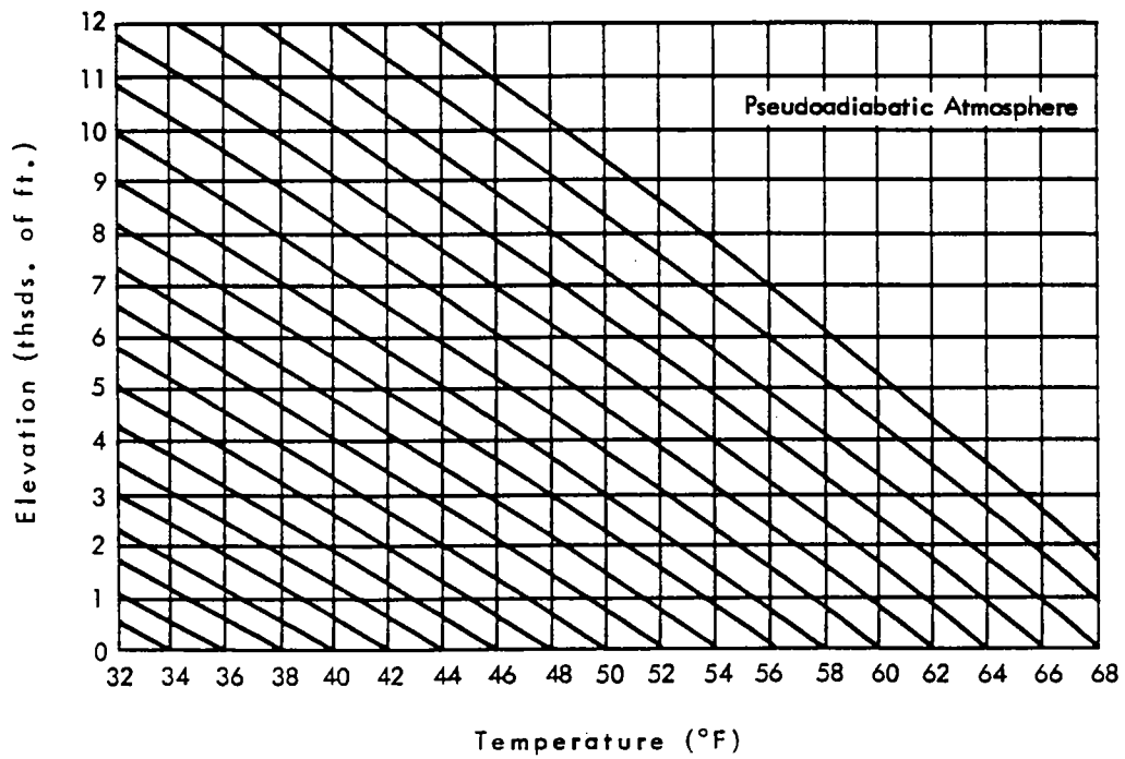
Figure 15.32.--Decrease of temperature with elevation (HMR 43).
