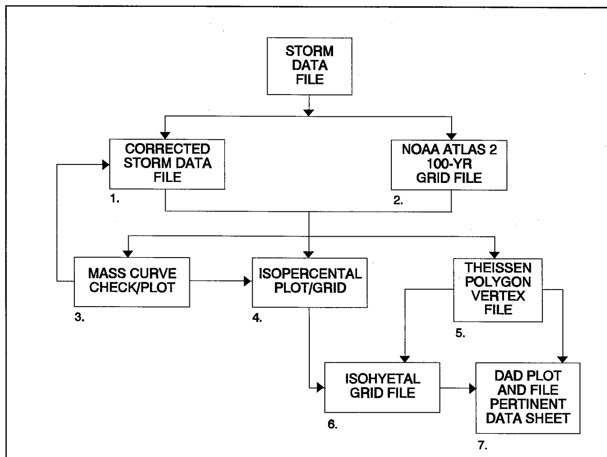
Figure 5.1.--Schematic flow diagram of modules created in processing storm rainfall data by the automated ministorm program. Modules are numbered and referenced in text.
