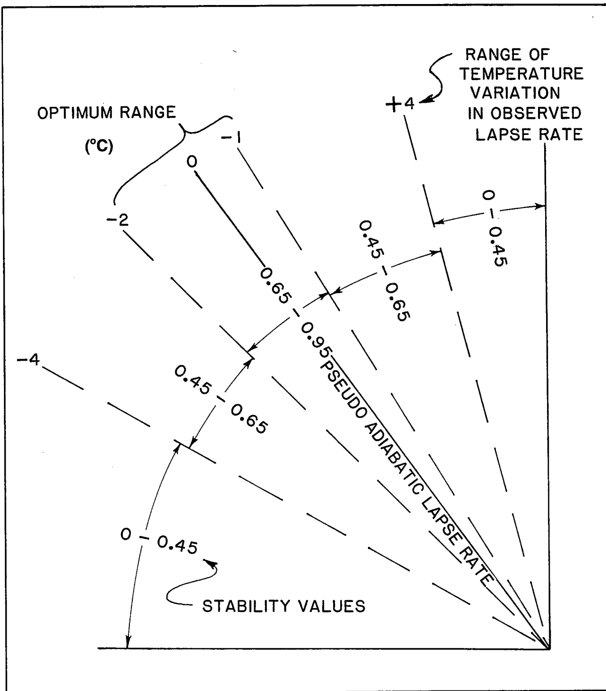
Figure 6.4--Schematic diagram to show relative range of stability values compared to the pseudo-adiabatic lapse rate.
