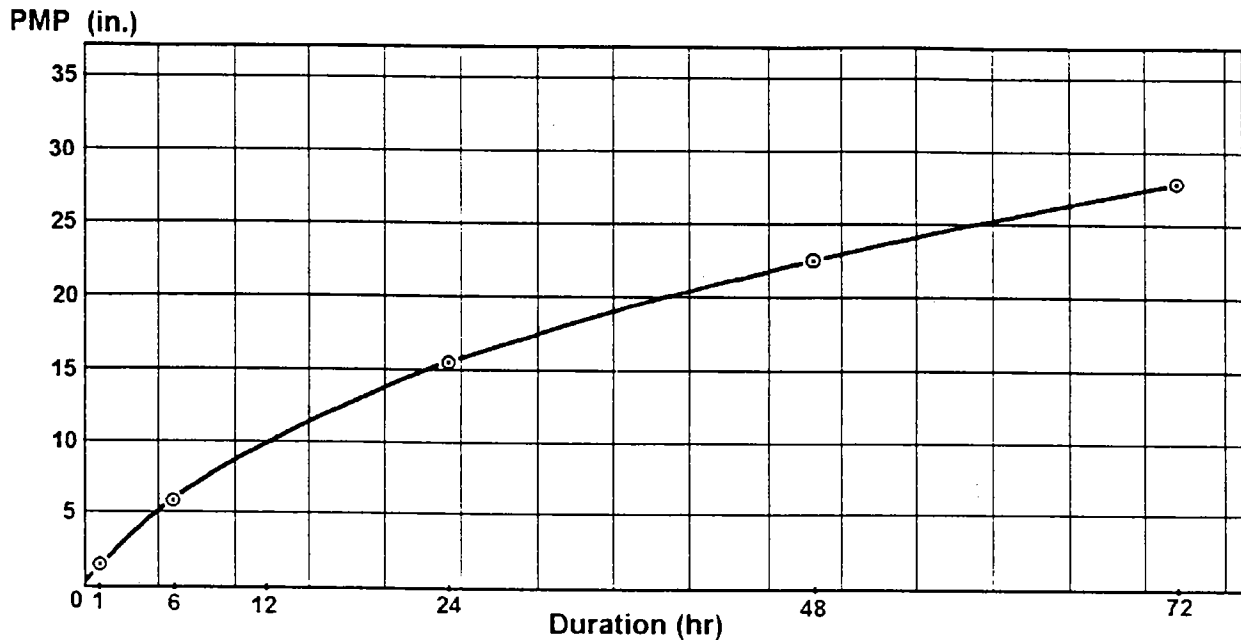
Figure 15.35.--Depth-duration curve for basin-averaged PMP for Mud Mountain dam basin (402-mi 2 ), Washington.
