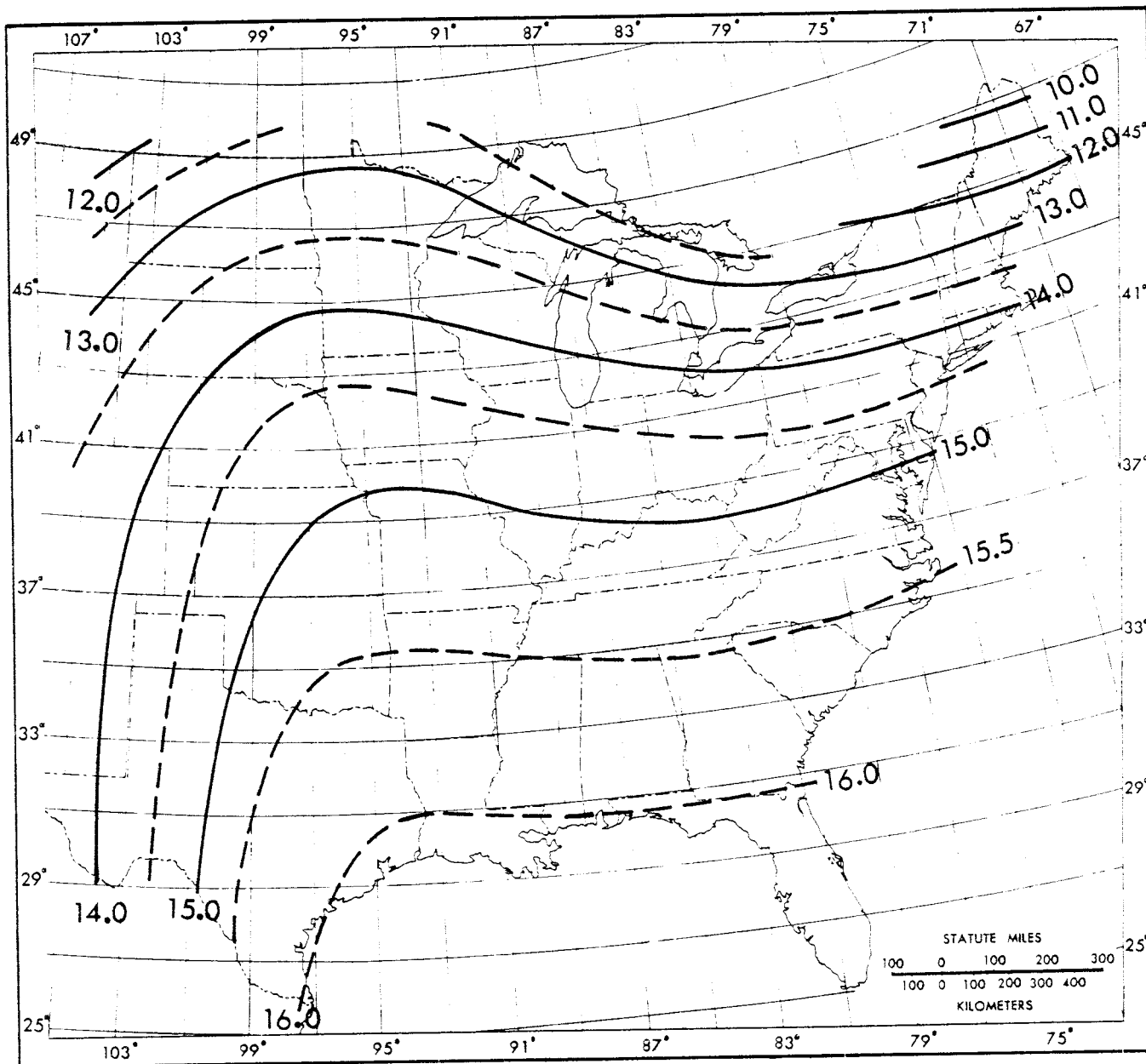
Figure 29.—1-hr 10-mi 2 PMP analysis for the eastern United States.
