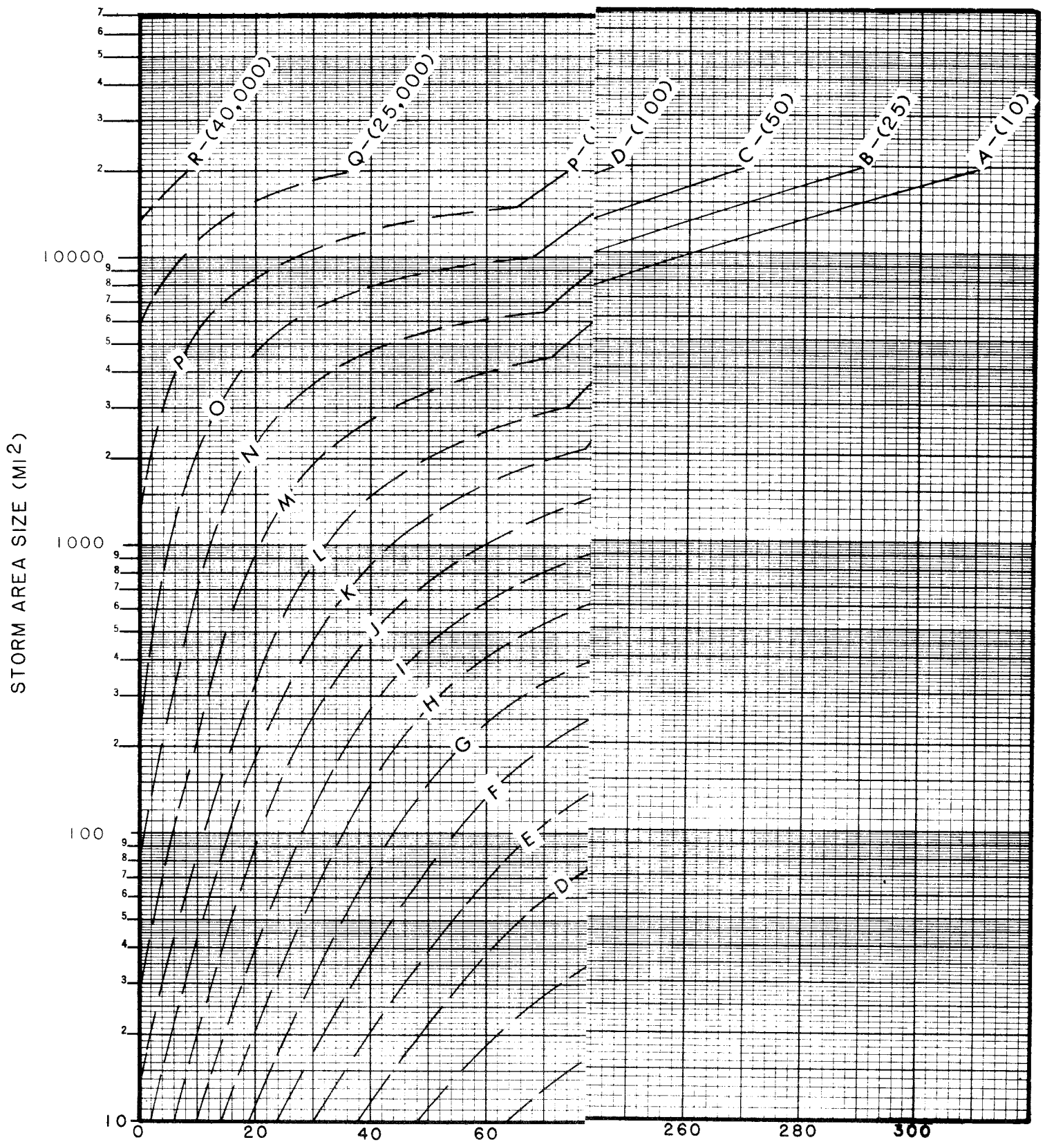
Figure 16.--Nomogram for the 1st 6-hr PM
