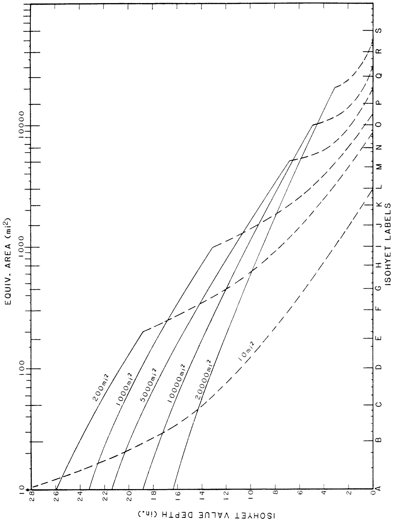
Figure 15.—Isohyetal profiles for standard area sizes at 37°N, 89°W.
