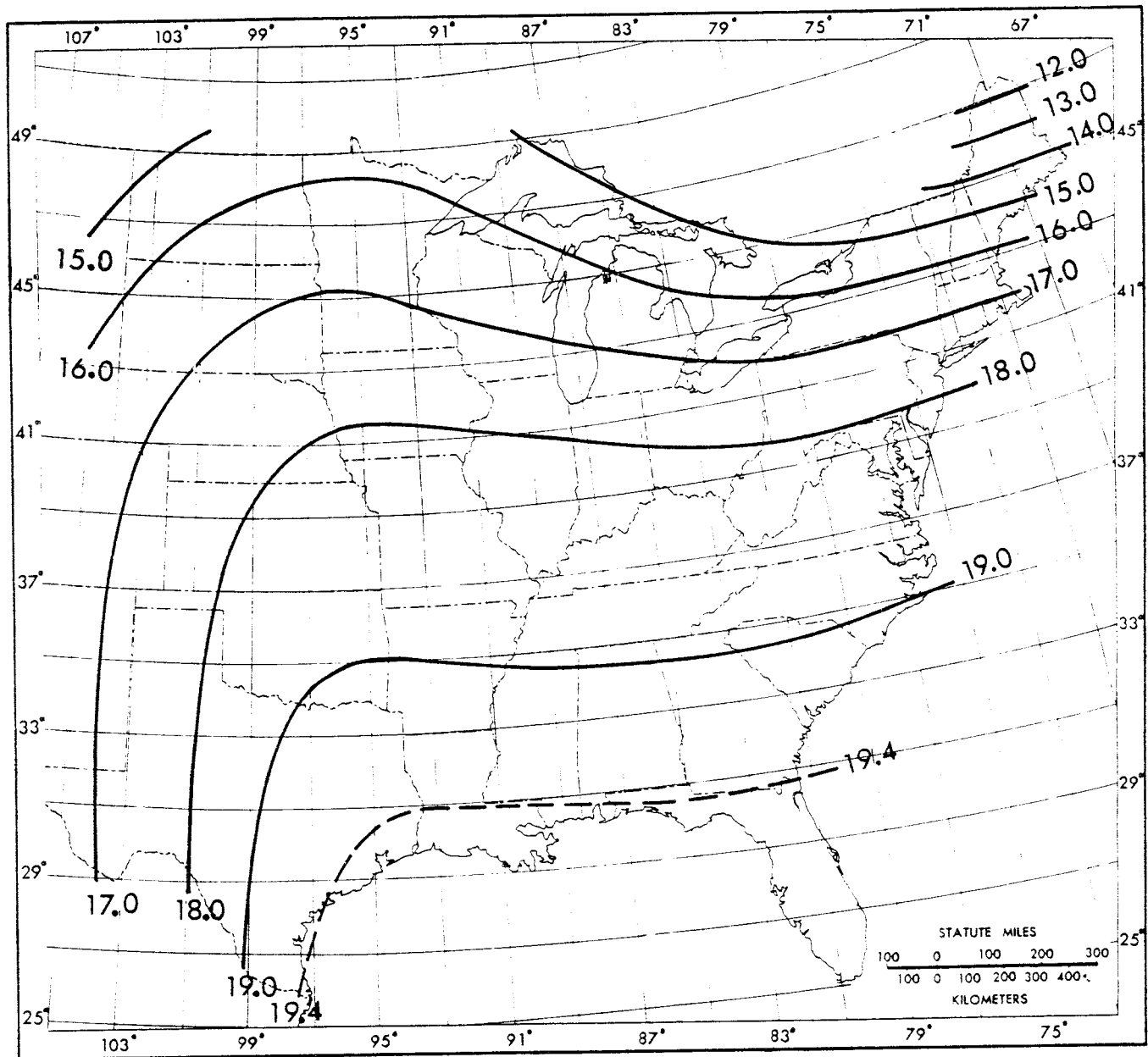
Figure 24.—1-hr 1-mi 2 FMP analysis based on figure 23 and 6-hr 10-mi 2 precipitation from BMR No. 51.
