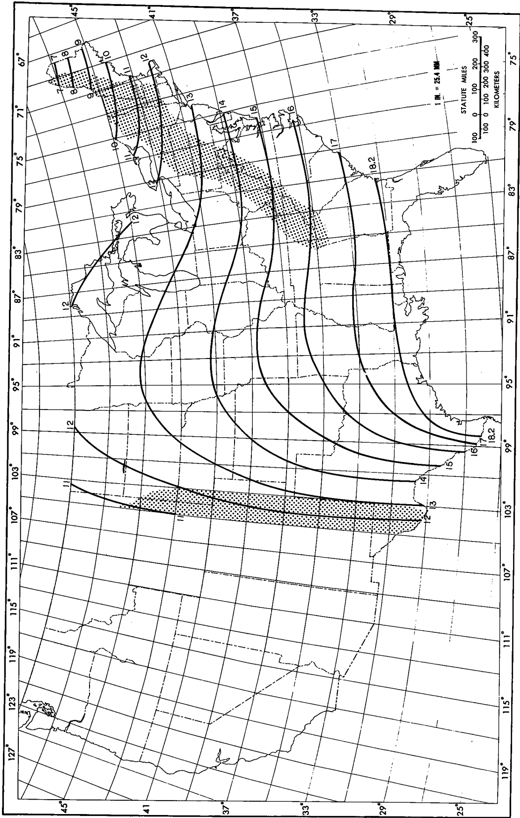
Figure 28. ---All-season PMF (in.) for 6 hr 1,000 mi 2 (2,590 km 2 ).
