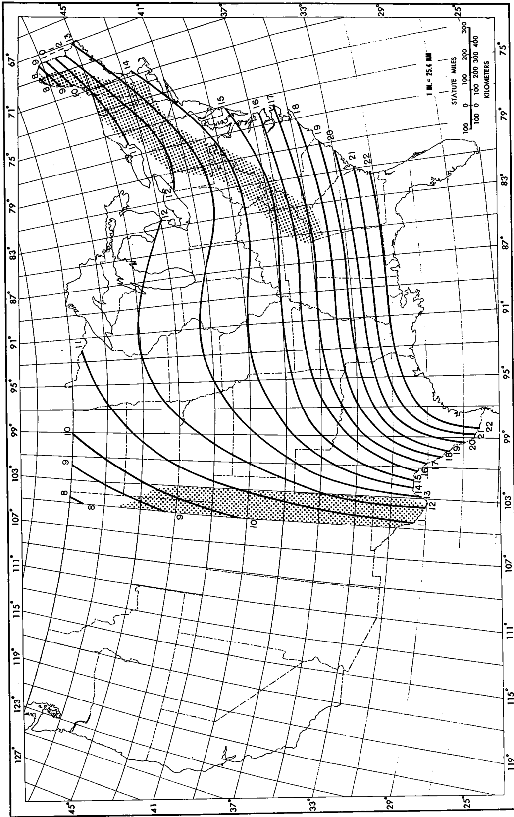
Figure 47. ---All-season PMP (in.) for 72 hr 20,000 mi 2 (51,800 km 2 ).
