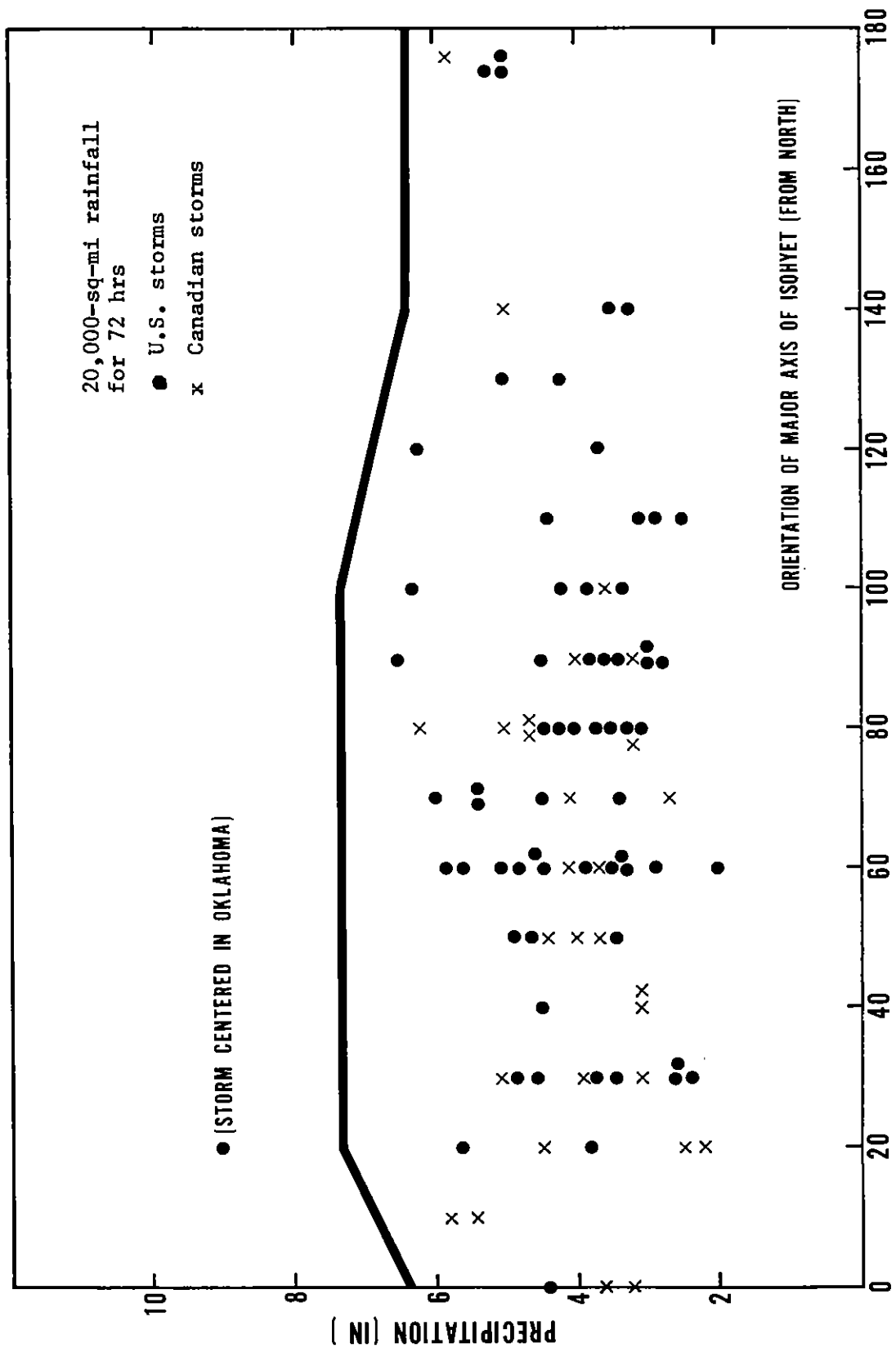
Figure 5-2.--Example of variation in rainfall with isohyetal orientation.
