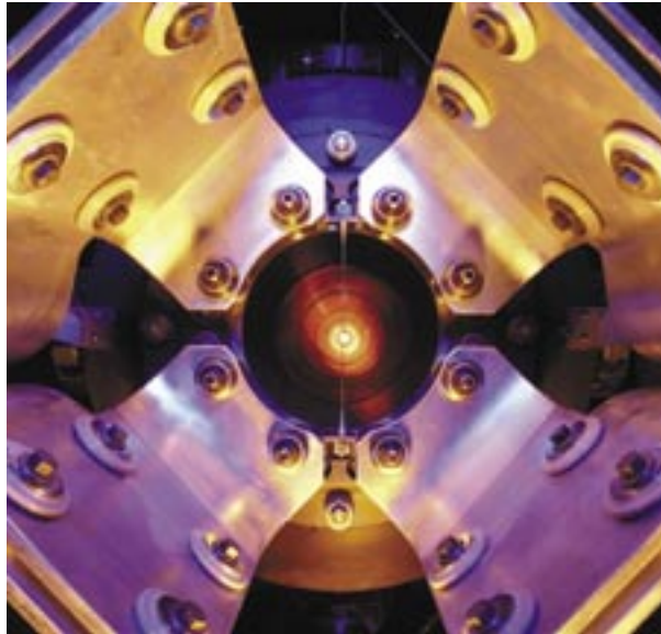
NuMI Horn for focusing particles at the NuMI experiment. Credit: Fermilab
