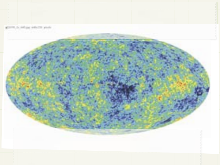
WMAP: DETAILED FULL-SKY MAP OF THE OLDEST LIGHT IN THE UNIVERSE!
