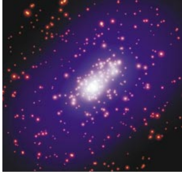
DARK MATTER MAP The total mass within giant galaxy cluster CL0025+1654 is the sum of the galaxies themselves, seen in yellow as ordinary luminous matter, plus the cluster's invisible dark matter shown in blue. The cluster's dark matter is not evenly distributed, but follows the clumps of luminous matter closely. Credit: J.-P. Kneib Observatoire Midi-Pyrenees, Caltech. ESA, NASA
