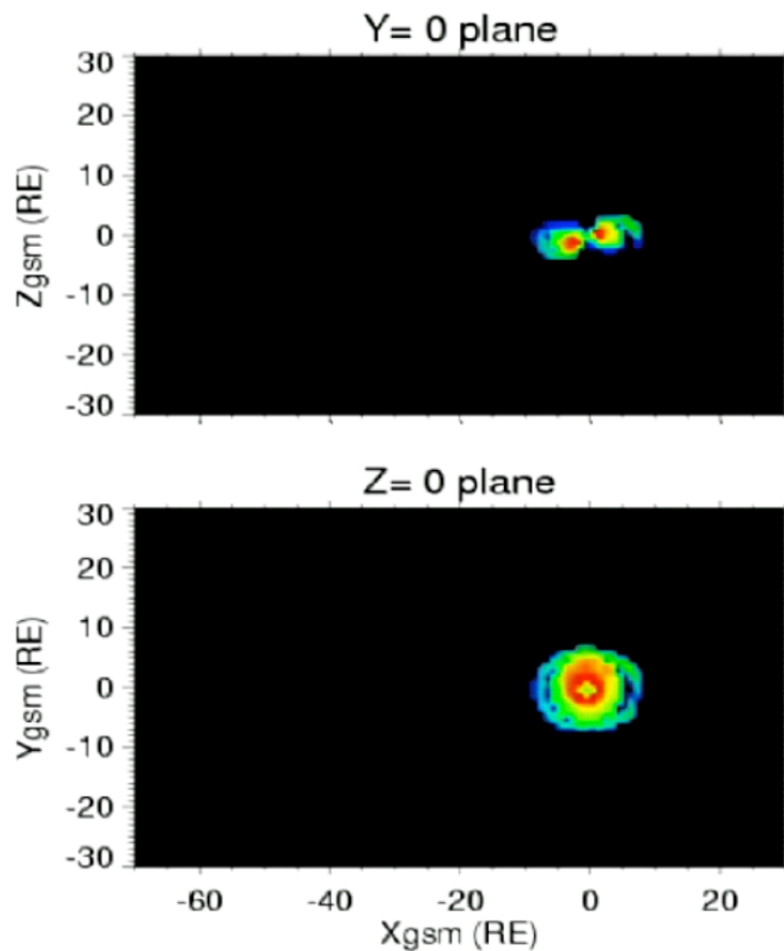
Normal Plasmasphere
