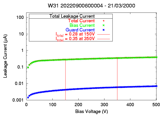
Figure 4.4: Bulk and surface currents in log scale.
