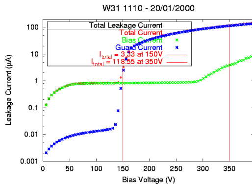
Figure 4.5: Current breakdown.
