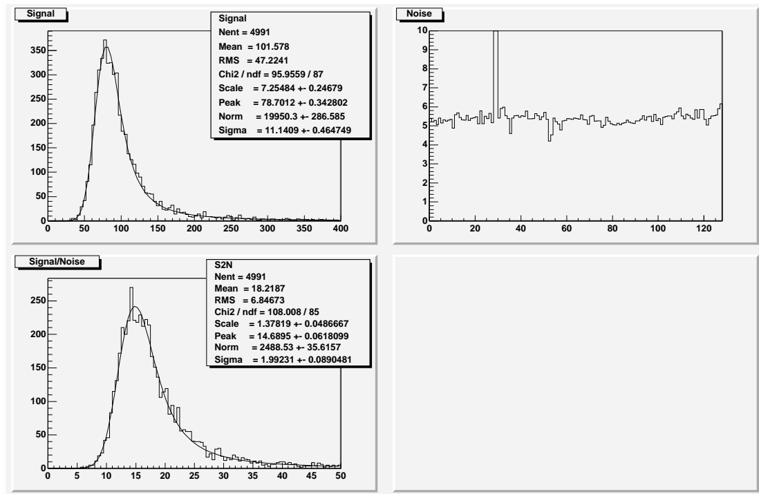
Figure 6.10: Signal, S/N and noise distribution at 350 V bias.
