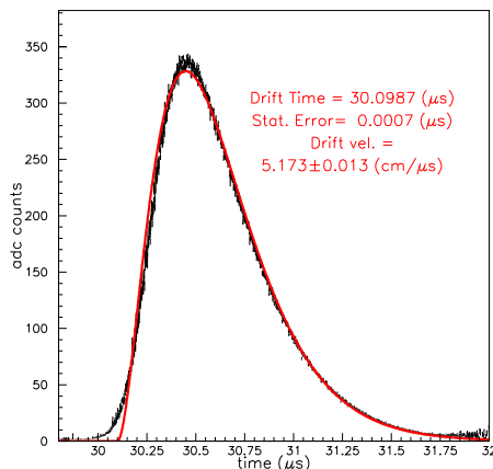
Figure 10.8: Pulse amplitude vs time of laser signals.
