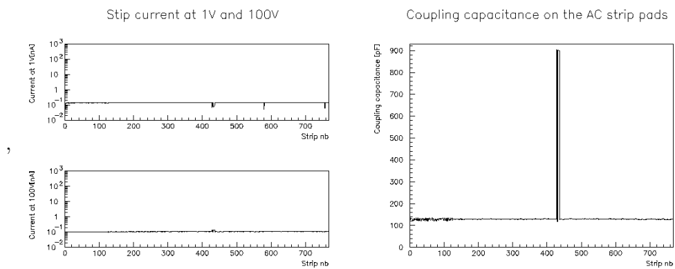
Figure 4.9: Strip integrity test: 7 shorts are present.
