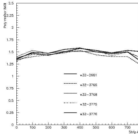
Figure 4.2: Polysilicon resistor value versus strip number.
