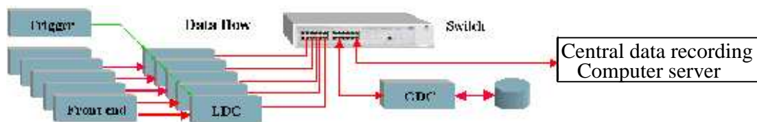
Figure 9.12: Layout of the HARP data flow.
