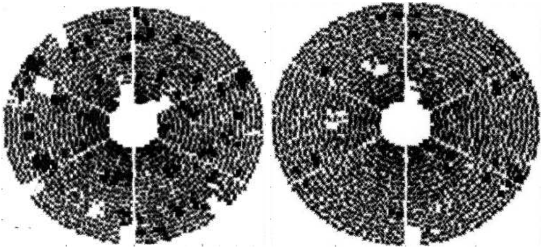
Figure 10.6: TPC active pads in 2001 (left) and 2002 (right).
