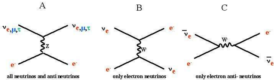
Figure 8.1: The amplitudes leading to matter effects on oscillations.
