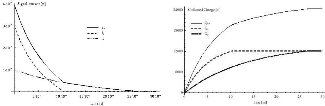
Figure 2.10: Current as a function of time (left) and its integral (right) for a 300\mu\text{m} thick detector, doped at 10^{12}/\text{cm}^3 , and overdepleted of 20\text{V} .
