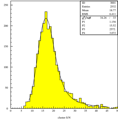
Figure 2.9: Typical signal to noise ratio distribution, measured in a silicon detector 300 \mu\text{m} thick. This quantity is proportional to the energy loss.
