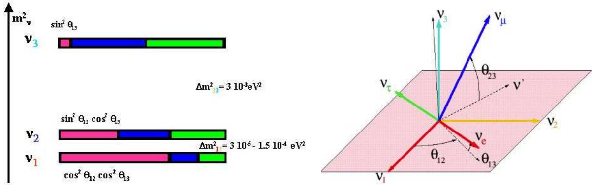
Figure 8.4: Three-neutrino (Mass) 2 spectrum (left plot) that accounts for the flavour changes of the solar and atmospheric neutrinos: the \nu_e fraction of each mass eigenstate is red, the one of \nu_\mu is blue and the one of \nu_\tau green, and scheme of the mixing angles (right plot).
