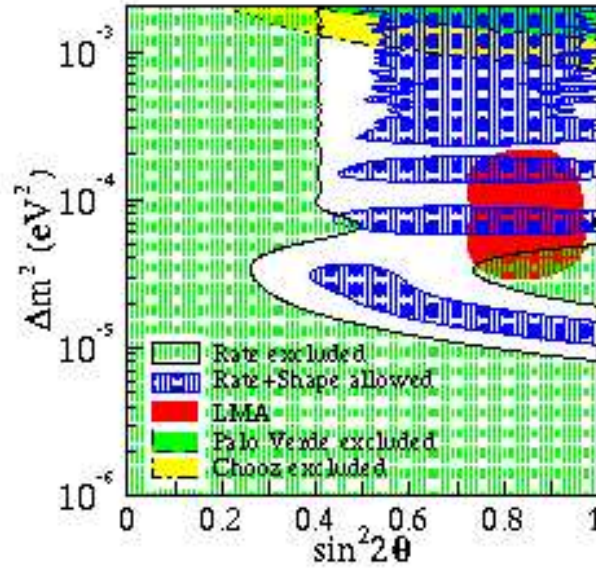
Figure 8.3: Excluded regions of neutrino oscillation parameters for the rateanalysis and allowed regions for the combined rate and shape analysis from KamLAND at 95% C.L. At the top are the 95% C.L. excluded region from CHOOZ [53] and Palo Verde [54] experiments and the 95% C.L. allowed region of “Large Mixing Angle” solution of solar neutrino experiments [55]. The thick dot indicates the best fit to the KamLAND data in the physical region: \sin^2 2\theta=1.0 and \Delta m^2 = 6.9 \times 10^{-5} eV^2 .
