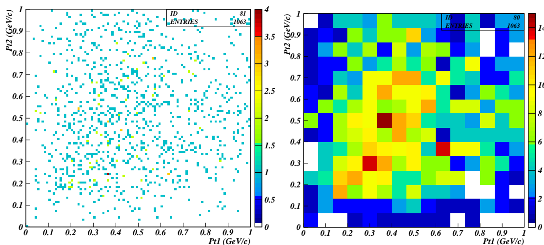
Figure 12.12: Correlation between the transverse momenta of the two branches of the cosmic rays tracks. In the left plot the bin width is 10 \text{ MeV}/c while in the right plot it is 66 \text{ MeV}/c .
