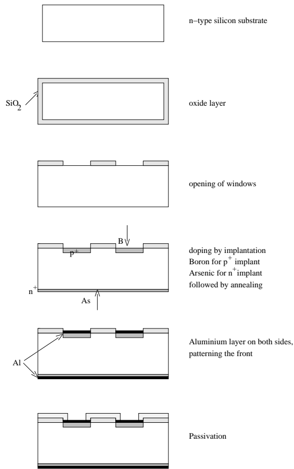
Figure 2.4: The planar process for detector fabrication.
