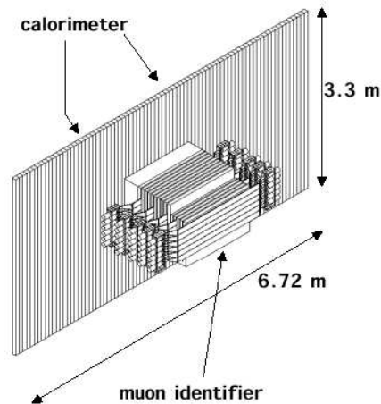
Figure 9.9: Layout of the muon identifier.
