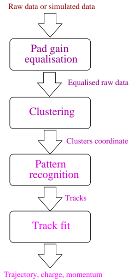
Figure 10.9: Logic flow of the HARP TPC reconstruction chain.
