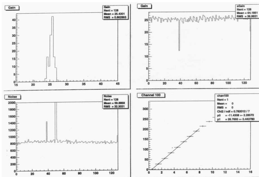
Figure 5.6: Chip performance test. The upper left plot represents the gain distribution in unit of mV/fC; the upper right plot shows the gain, in mV/fC, over the 128 channels. The lower left figure shows the noise, in number of electrons, for all the channels, while the last one shows the gain of the channel 100 versus the test pulse height.
