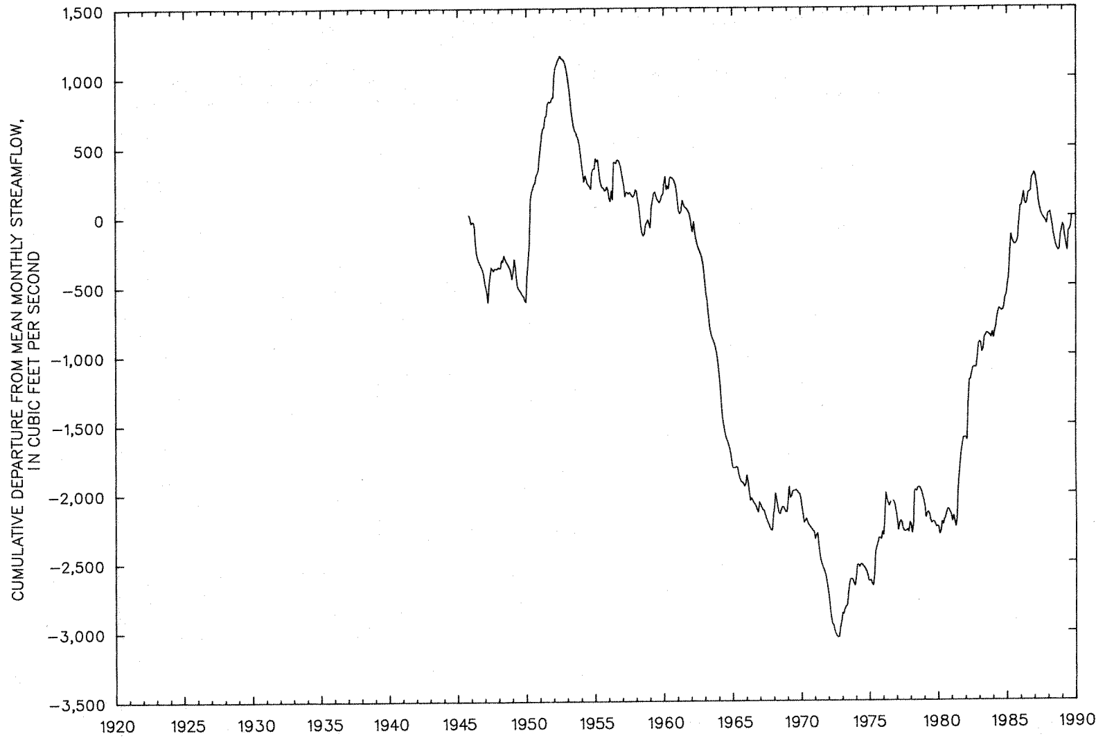
Figure 61.—Cumulative departure from mean monthly streamflow for Pigeon Creek near Angola (04099510), water years 1946–89.
