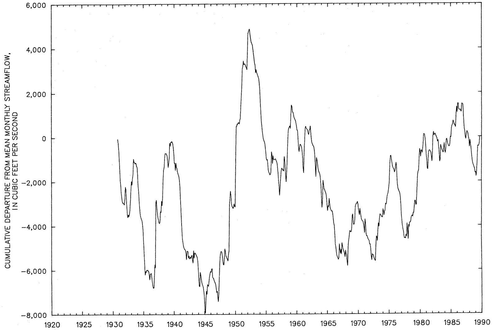
Figure 57.—Cumulative departure from mean monthly streamflow for Flatrock River at St. Paul (03363500), water years 1931–89.
