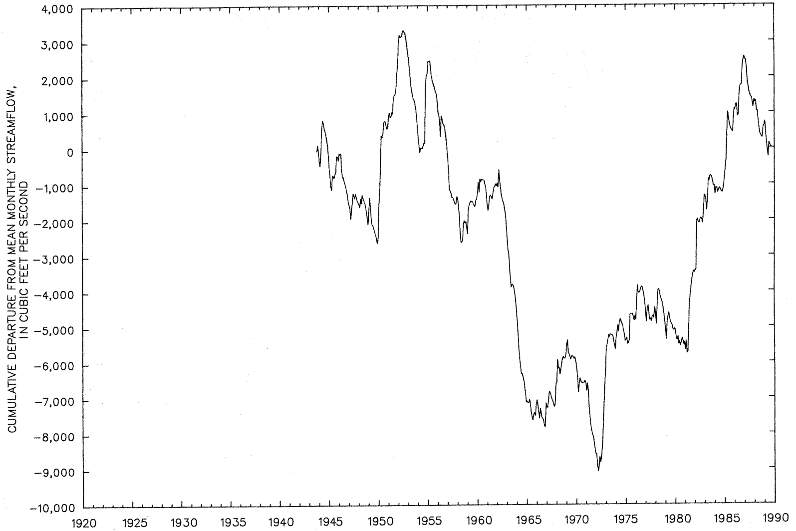
Figure 65.—Cumulative departure from mean monthly streamflow for Yellow River at Knox (05517000), water years 1944–89.
