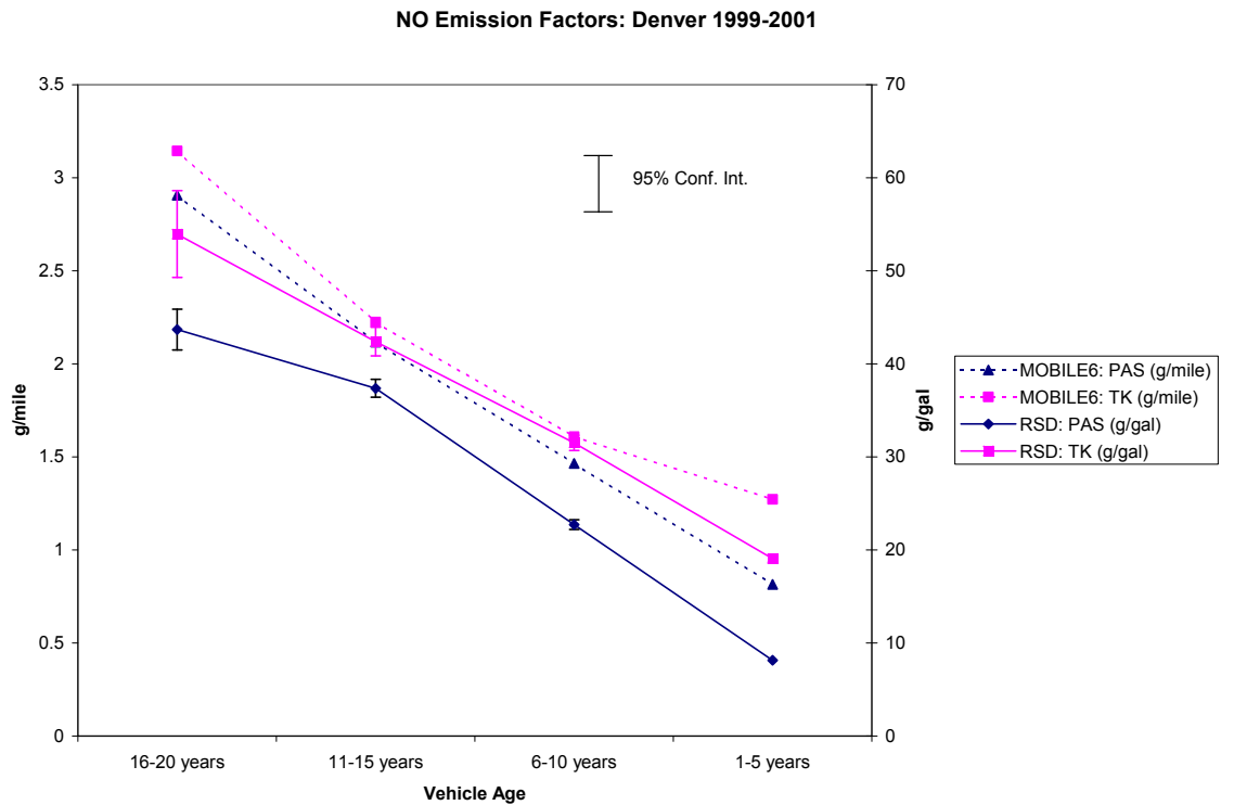
Figure 4-5. Mean NO emissions as a function of vehicle age from RSD data (in g/gal) and from MOBILE6 (in g/mile): Denver, 1999 – 2001.
