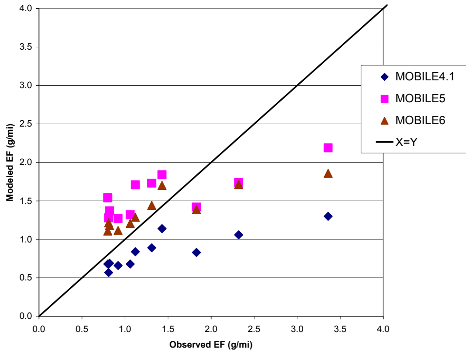
Figure 2-5. Comparison of observed to modeled fleet average NOx emission factors at Fort McHenry (1992), Bore 3.
