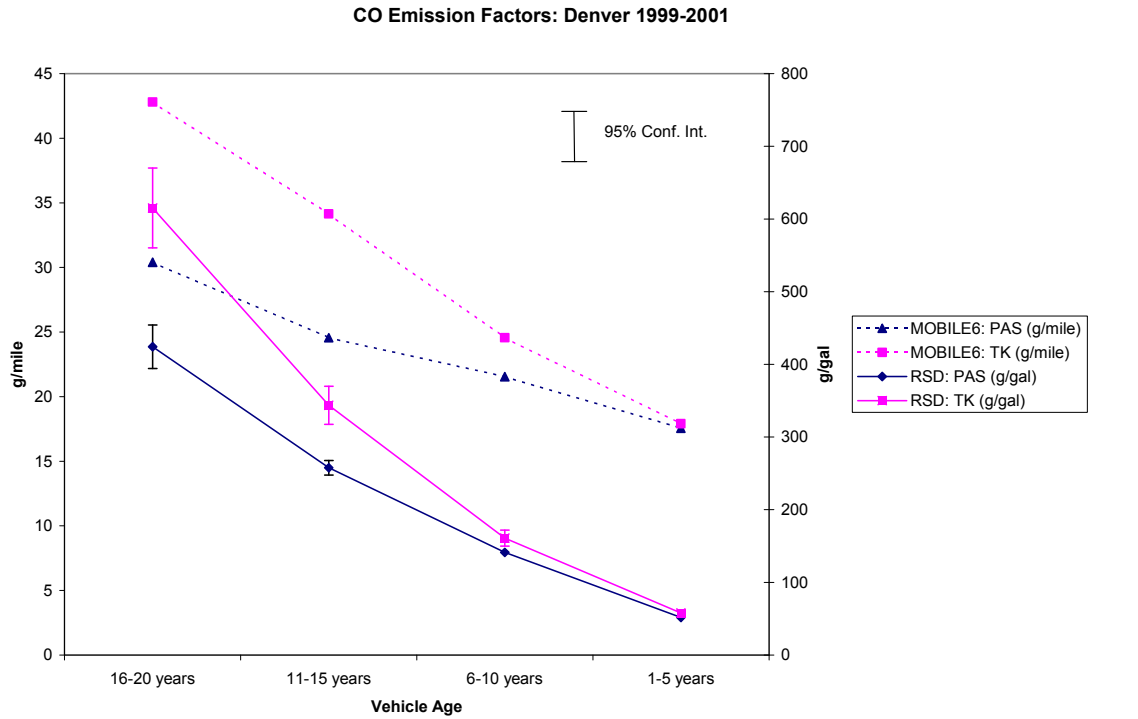
Figure 4-4. Mean CO emissions as a function of vehicle age from RSD data (in g/gal) and from MOBILE6 (in g/mile): Denver, 1999 – 2001.
