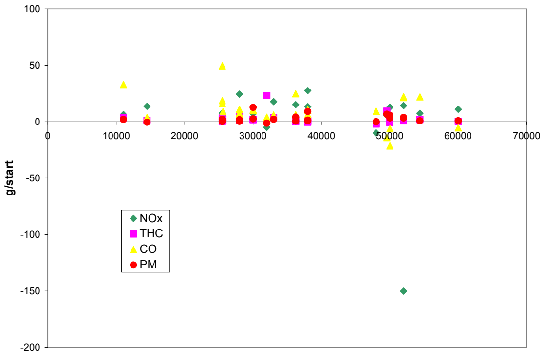
Figure 5-7. HDDV start increment by gross vehicle weight rating.
