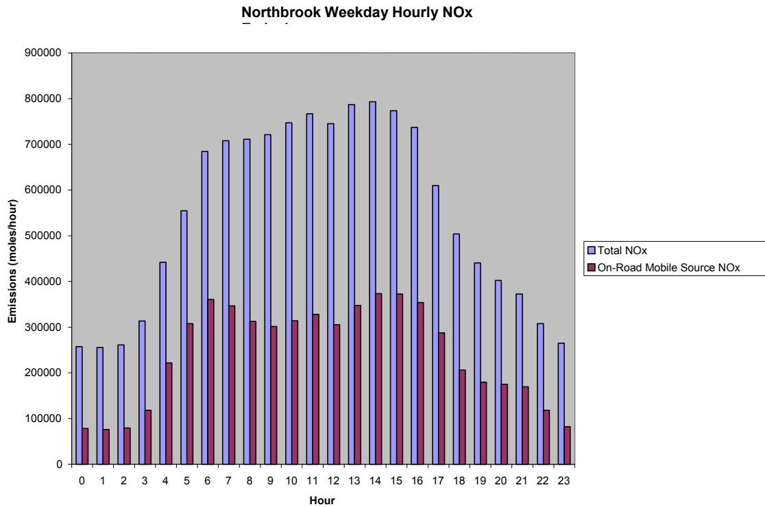
Figure 3-11. Weekday hourly emissions Northbrook: VOC (above), NOx (below).
