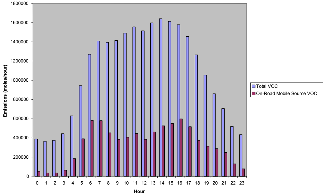
McMillan Weekday Hourly VOC Emissions
