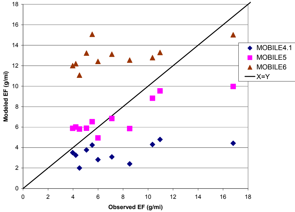
Figure 2-3. Comparison of observed to modeled fleet average CO emission factors at Fort McHenry (1992), Bore 3.
