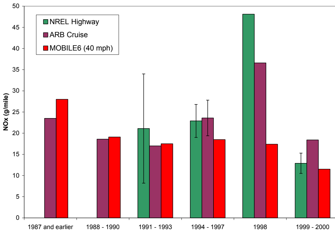
Figure 5-4. Comparison of NOx emission rates by model year for Class 8a truck driving on a freeway with an average speed of 40 mph.
