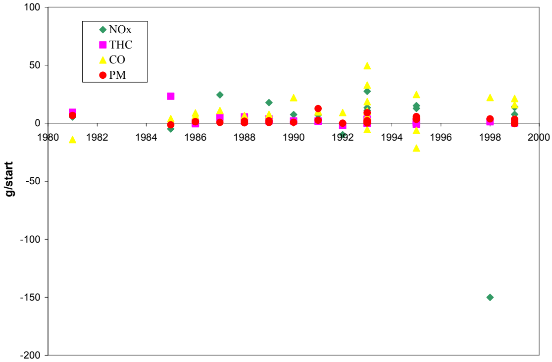
Figure 5-6. HDDV start increment by model year.
