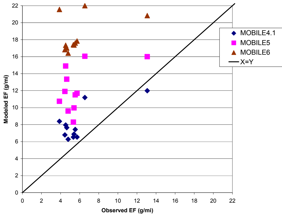
Figure 2-8. Comparison of observed and modeled fleet average CO emission factors at Tuscarora Mountain (1992).
