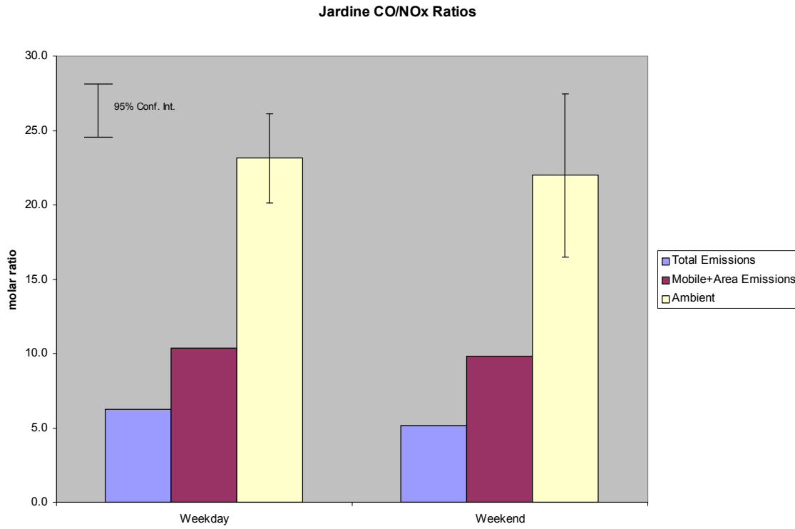
Figure 3-18b. Weekday and weekend morning CO/NOx ratios: Jardine.
