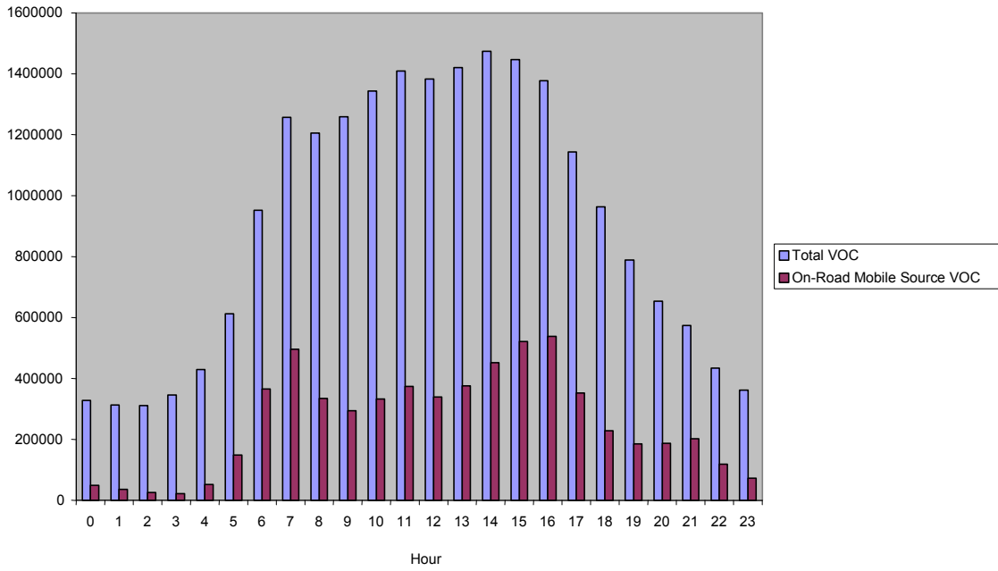
Lynn Weekday Hourly VOC Emissions
