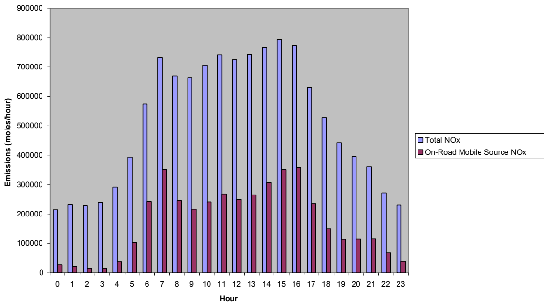
Figure 3-9. Weekday hourly emissions for Lynn: VOC (above), NOx (below).
