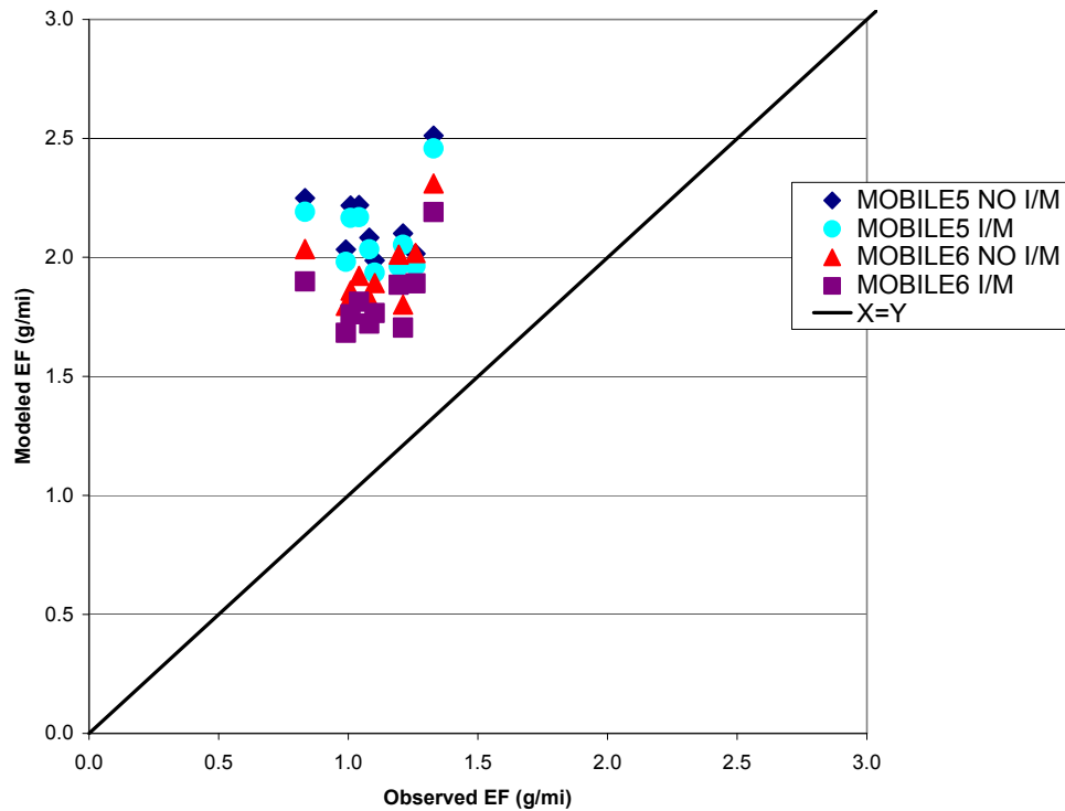
Figure 2-14. Comparison of observed and modeled fleet average NOx emission factors at Callahan Tunnel (1995).
