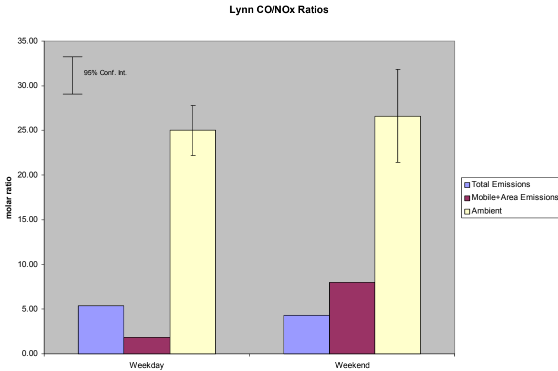
Figure 3-18c. Weekday and weekend morning CO/NOx ratios: Lynn.
