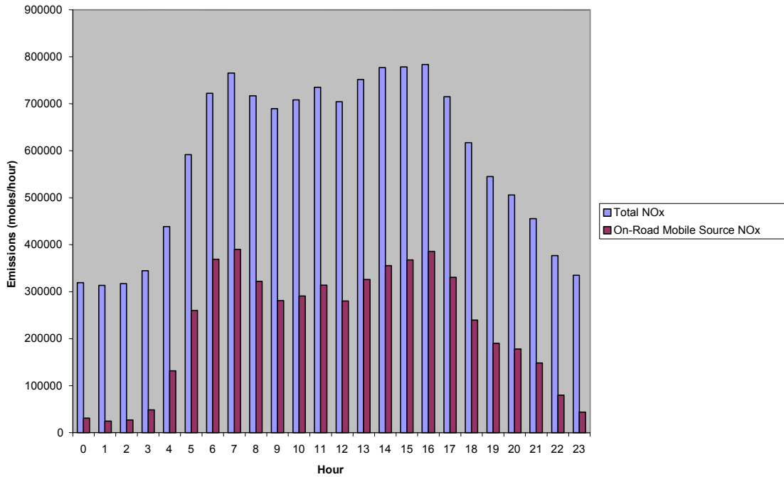
McMillan Weekday Hourly NOx Emissions
