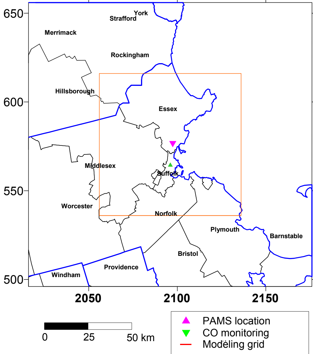
Figure 3-5c. PAMS and CO monitoring station locations (yellow square indicates 40 x 40 km emissions grid area): Lynn.
