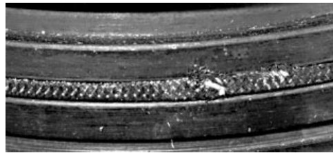
Figure 8.—Photo of 1/16 in. hybrid seal after scrubbing, 250 psi preload.
