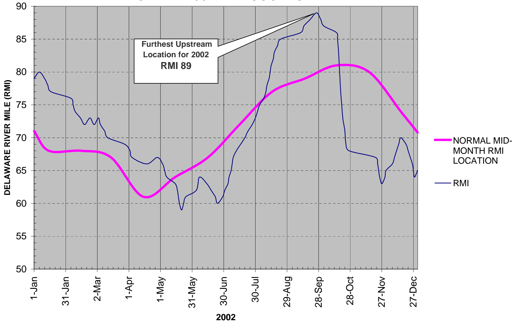
FIGURE 12: LOCATION OF THE 7-DAY AVERAGE OF THE 250-PPM ISOCHLOR
