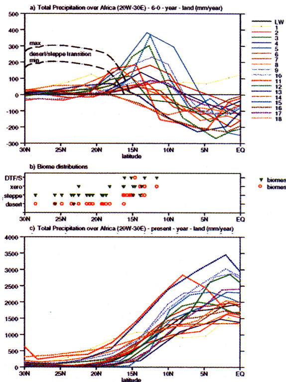
Figure 3. Zonal average climate and distribution of biomes in northern Africa (20W-30E). (a) 6 ka BP minus present annual precipitation (mm/year). The hatched lines are estimated upper and lower bounds for the excess precipitation required to support grassland, based on present climatic limits of desert and grassland taxa in paleoecological records (D. Jolly and I.C. Prentice, unpublished results). (b) Biome distributions (desert, steppe, xerophytic and dry tropical forest/savannah (DTF/S)), 6 ka BP and present (c) Simulated present day annual precipitation (mm/year) compared to climatology [Legates and Willmott (LW), 1990].
