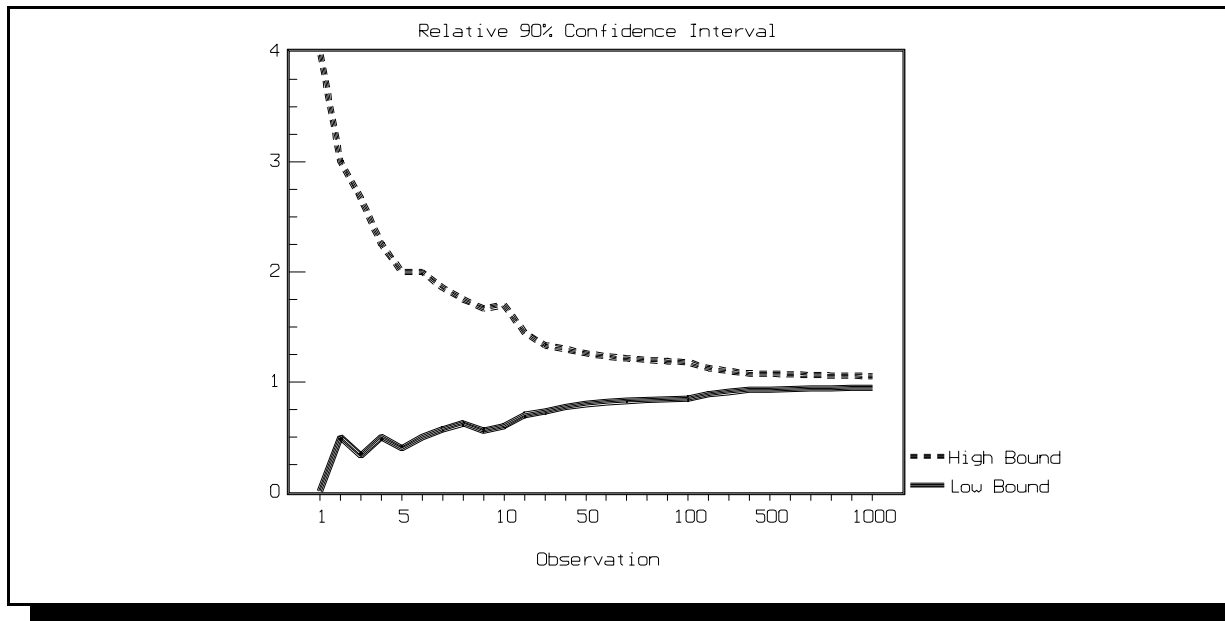
EXHIBIT 13 CONFIDENCE INTERVAL VERSUS NUMBER OF OBSERVATIONS
