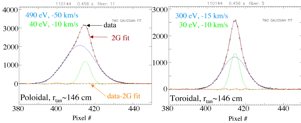
FIGURE 2. The He II spectrum under the influence of RF heating, fit with 2 Gaussians.
