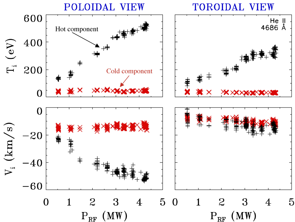
FIGURE 4. The temperature of the "hot" component scales as P_{RF}^{0.47} , whereas the temperature of the "cold" component is not effected by the amount of RF power applied to the plasma. He II data from Shots 110133-110145 are shown.
