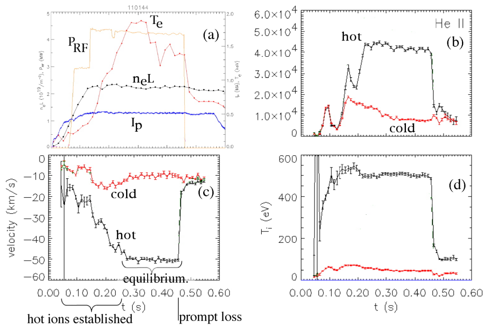
FIGURE 3. Time evolution of NSTX Shot 110144, showing (a) I_p , T_e , n_e , and P_{RF} and the hot and cold components of poloidally measured He II (b) brightness, (c) velocity, and (d) temperature at a tangency radius of 146 cm.
