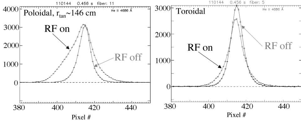
FIGURE 1. The He II spectrum from Shot 110144 during adjacent 10 ms time slices (centered on 455 and 465 ms), showing the difference in the poloidal view and toroidal view when HHFW RF heating is applied to the plasma. RF heating ends at 460 ms. Both views are tangent to the flux surface at \sim 146 cm. Error bars indicate statistical uncertainty.
